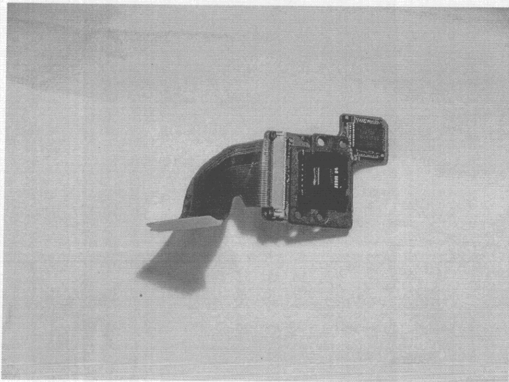
CCD PCB (Top View)
