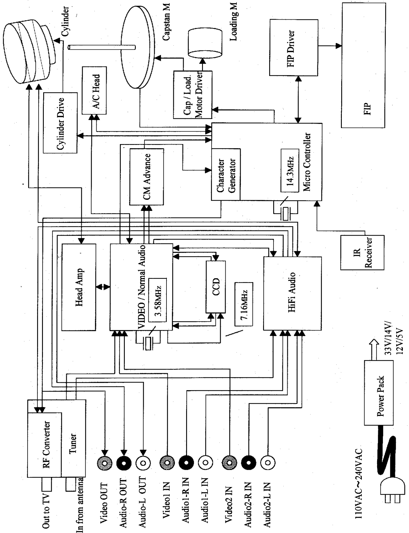
Block Diagram
