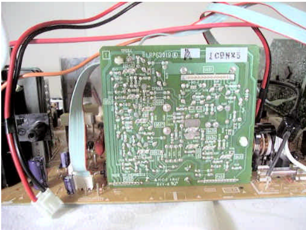
Vertical PCB (Bottom view)
