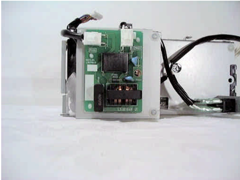
Line Filter PCB (Top View)
