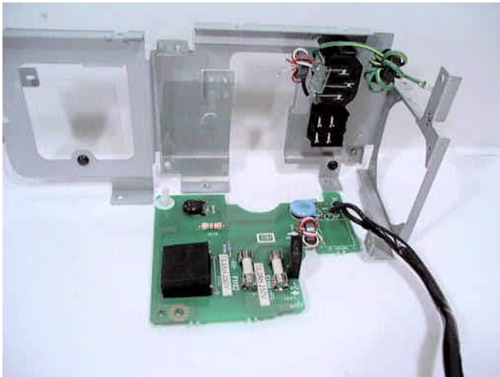
Filter PCB (Top View)
