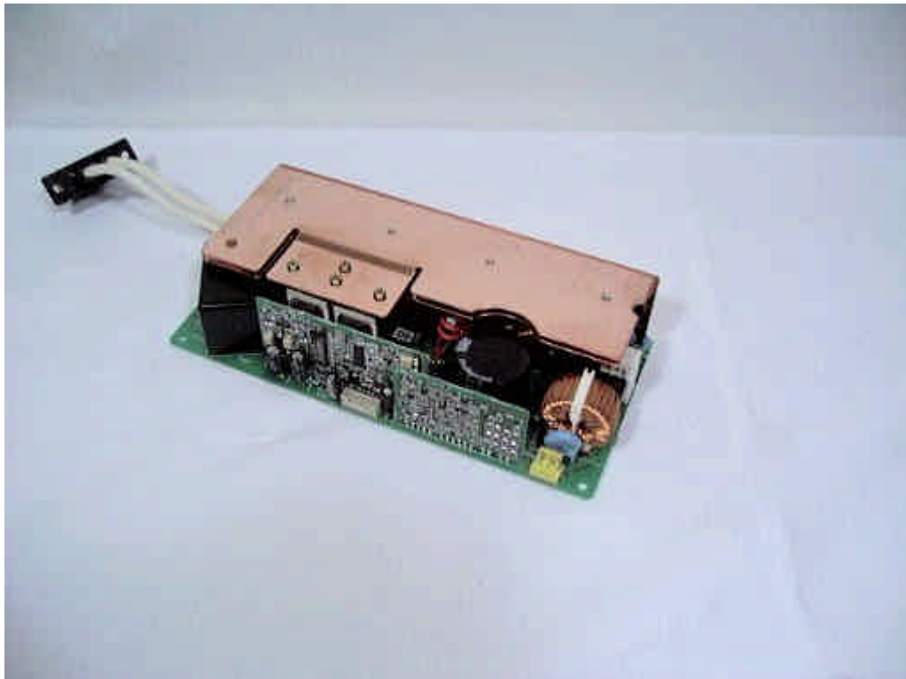
Main Power PCB (Top view)
