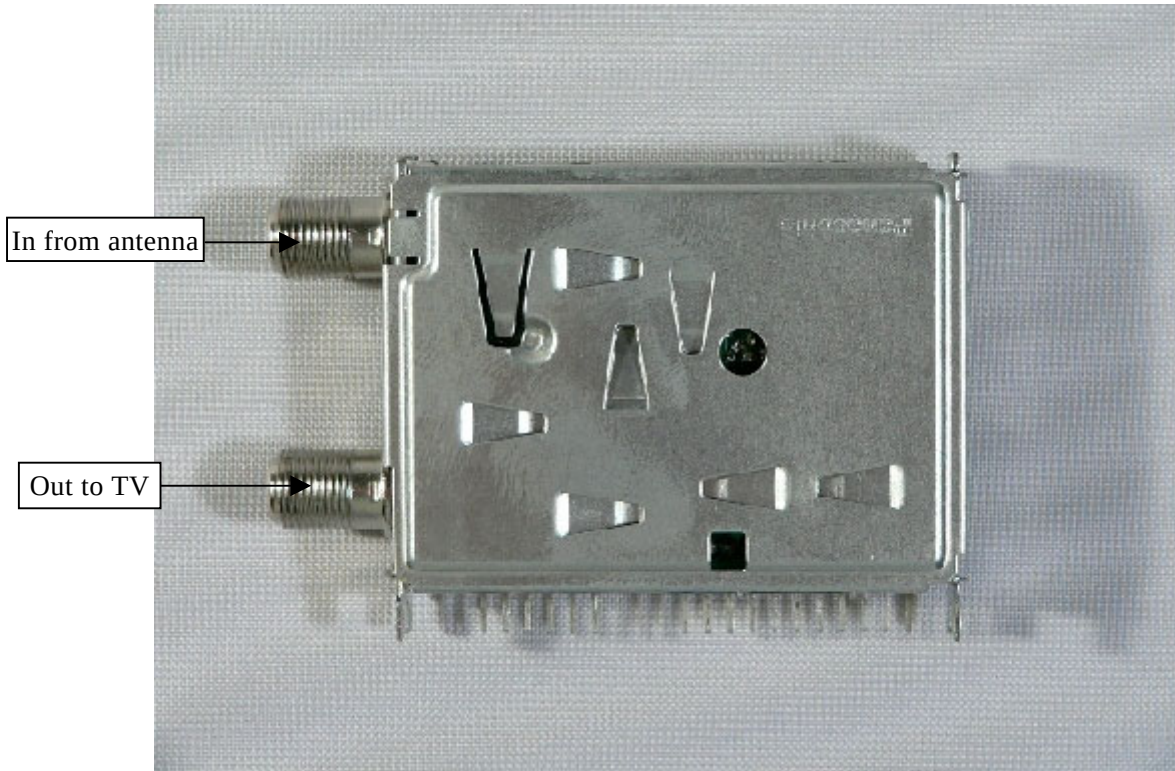
Tuner (ENG56D06G1: Top view)
