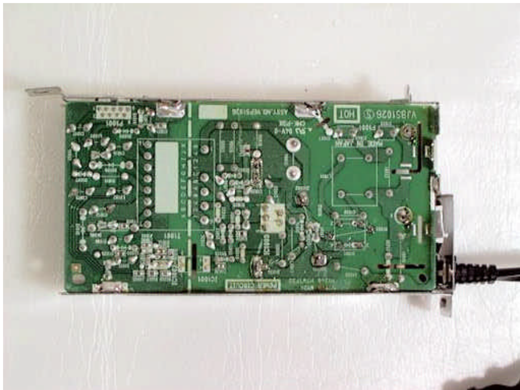
Power PCB (Bottom view)
