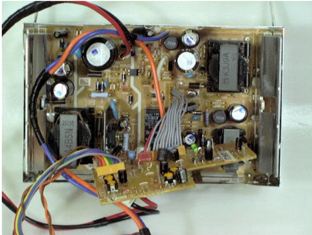
Power PCB (Top view)
