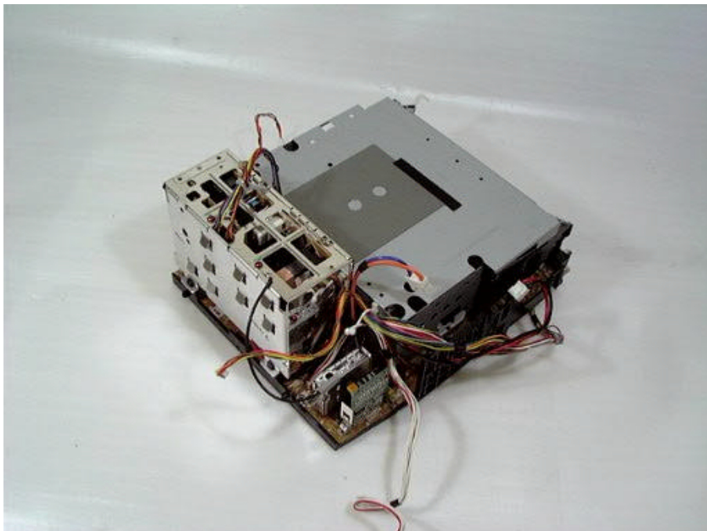
Power PCB & VCR Main PCB
