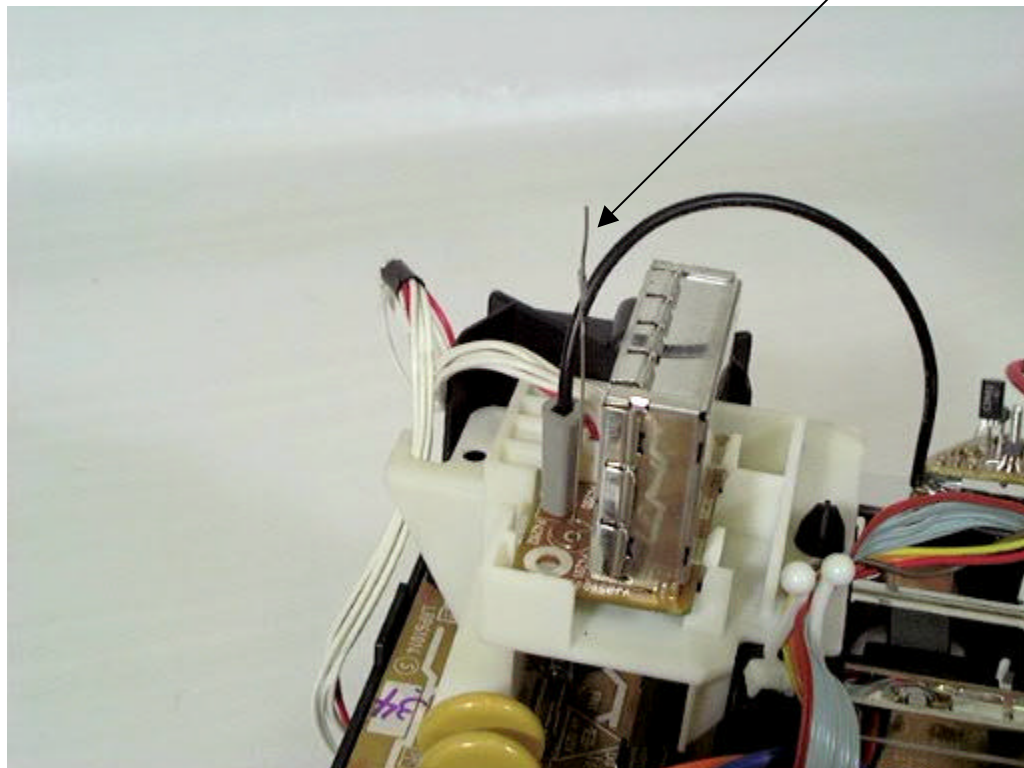
FM Transmitter PCB (Top view) Rod Antenna
