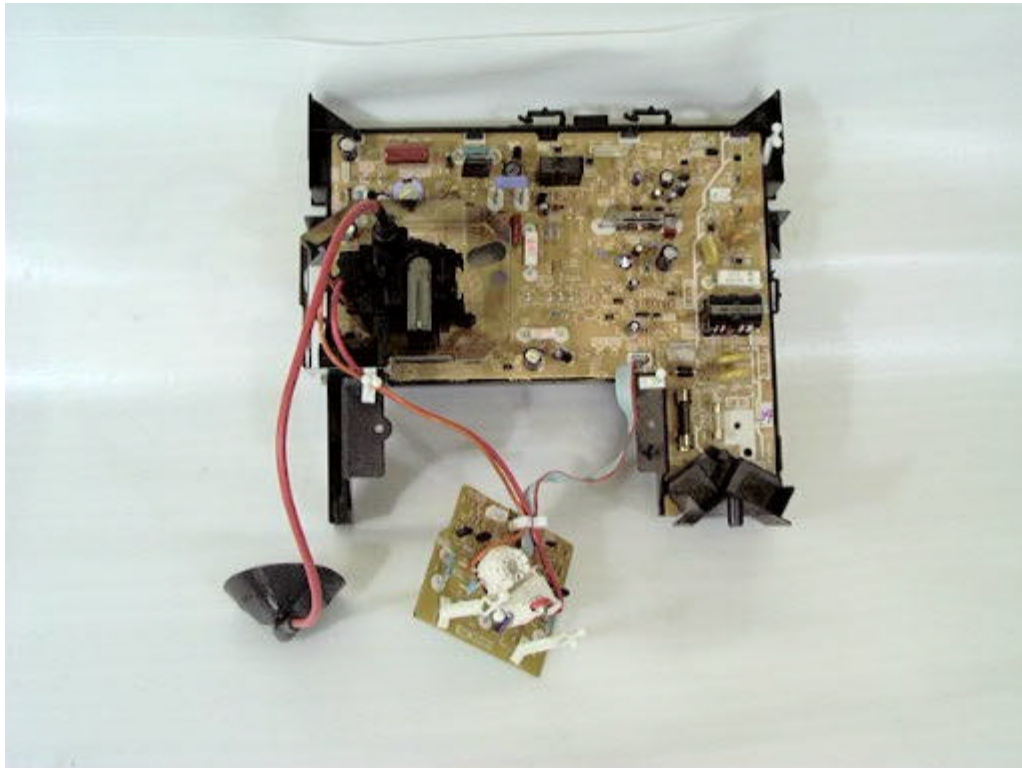
TV Main PCB (Top View)
