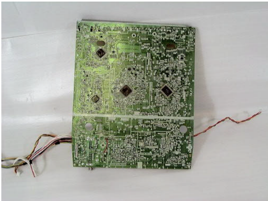
VCR Main PCB (Bottom View)
