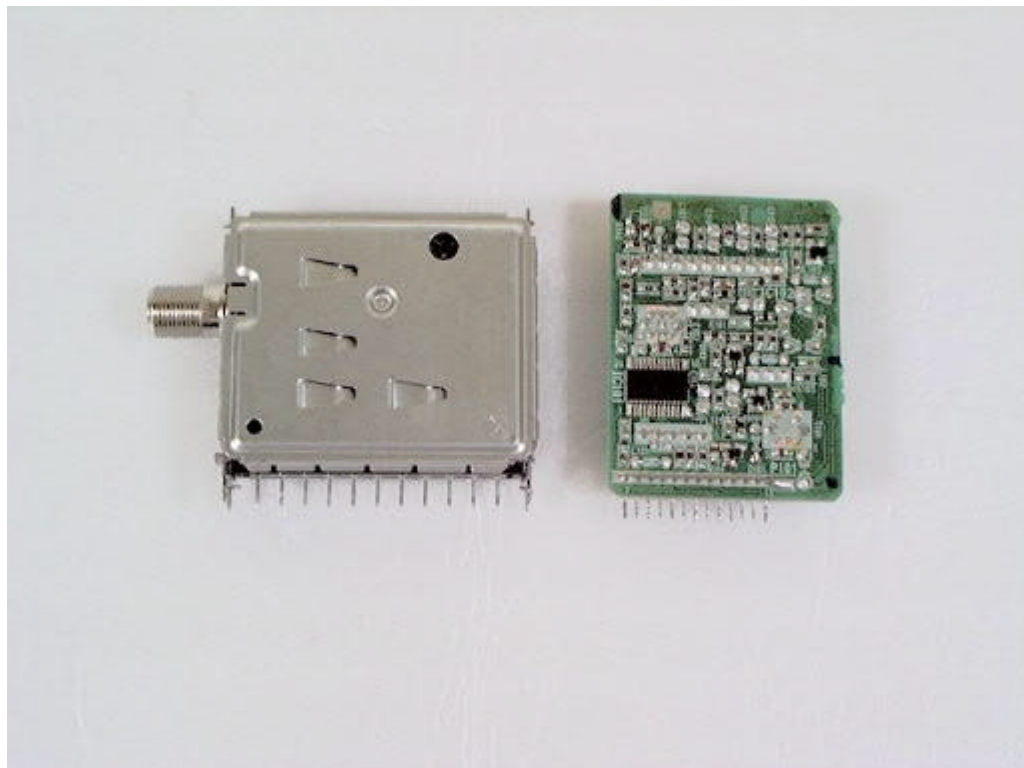
Tuner PCB & IF PCB (Bottom View)
