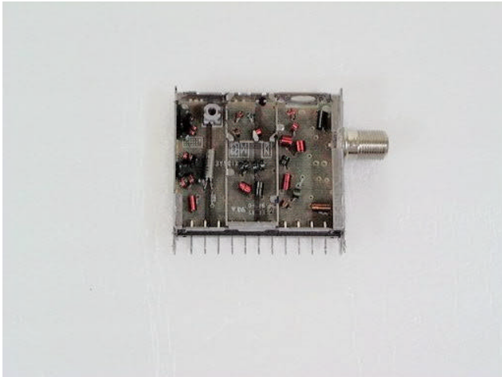
Tuner PCB (Top View)
