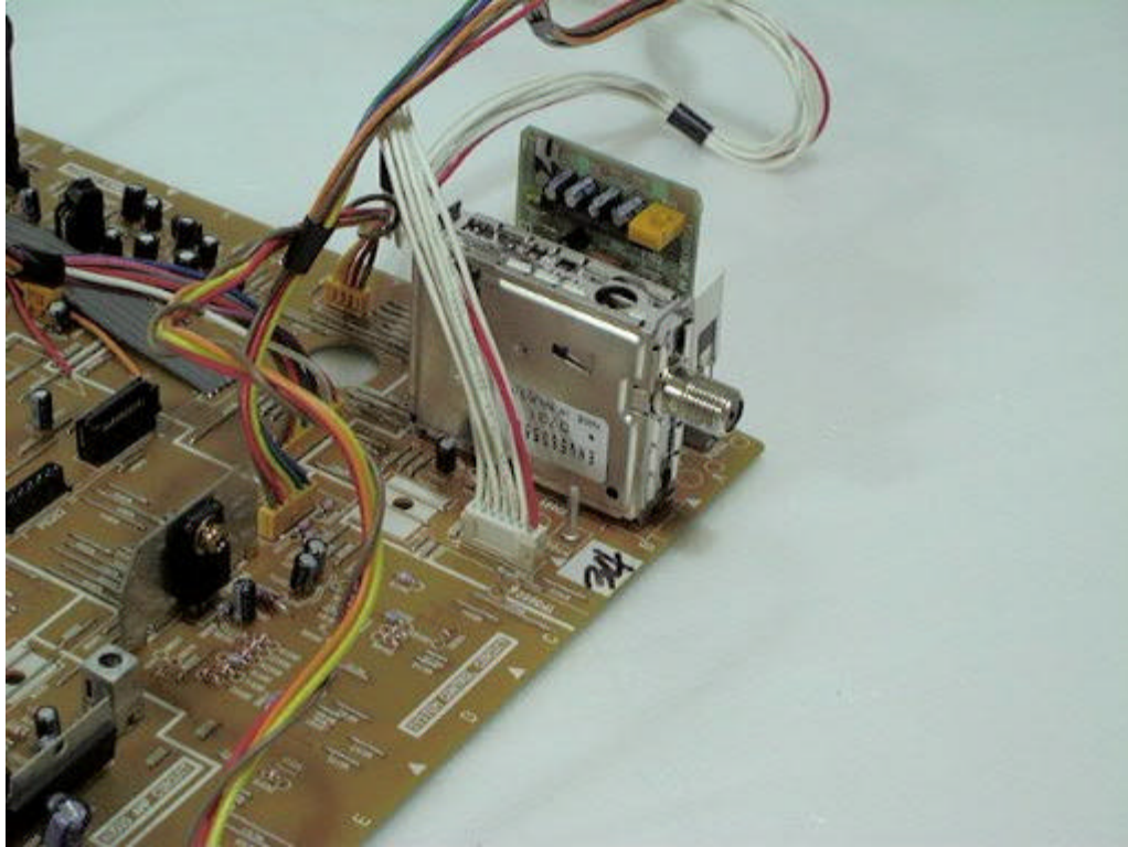
Tuner PCB & IF PCB (Top View)
