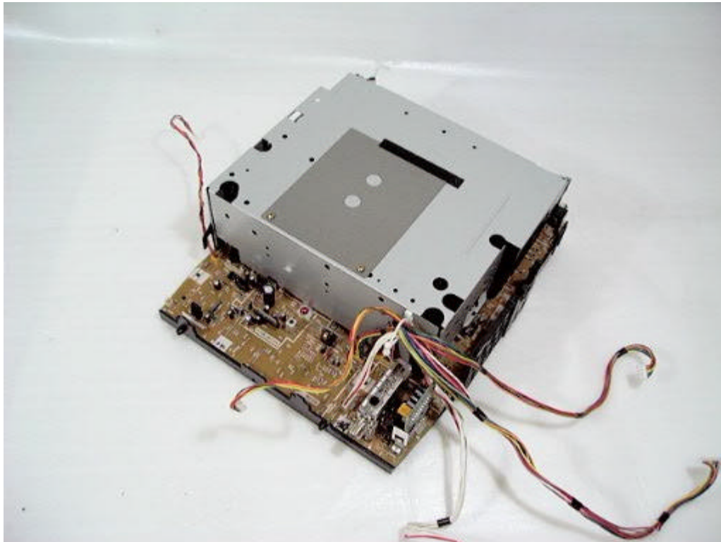
VCR Main PCB (Top View)
