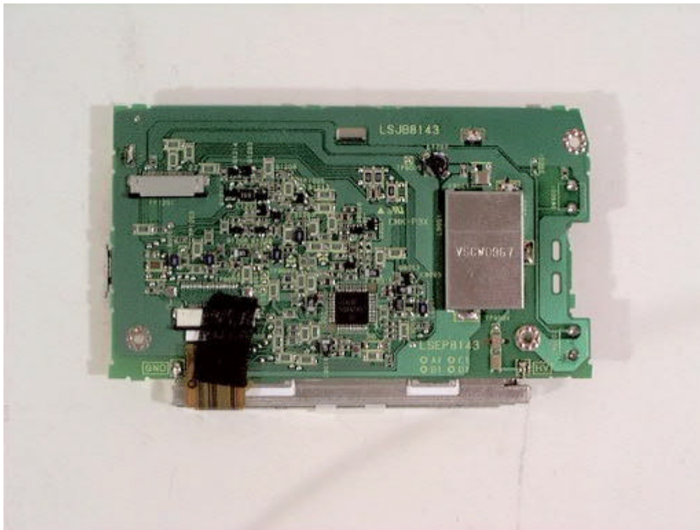
LCD Power PCB (Bottom view / Pulse transformer: ETJ11K95AM)
