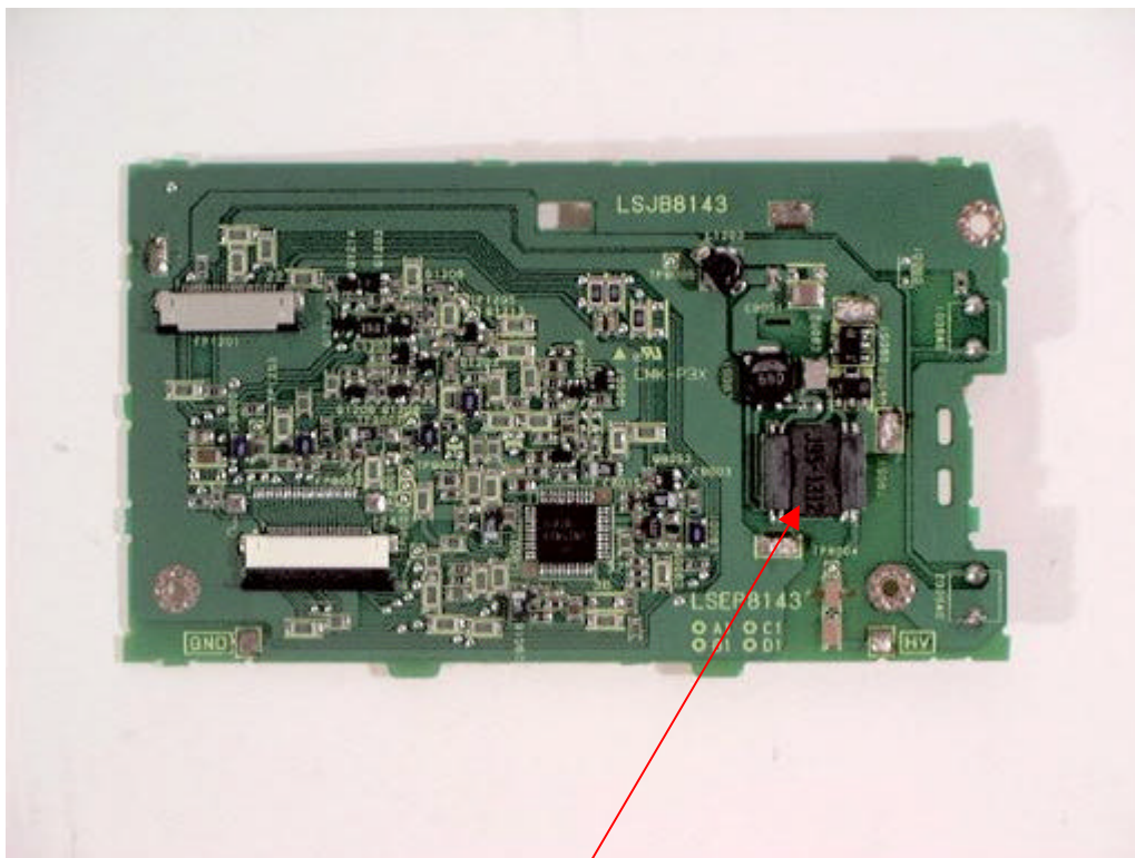
Oscillator circuit (Pulse transformer: ETJ11K95AM)
