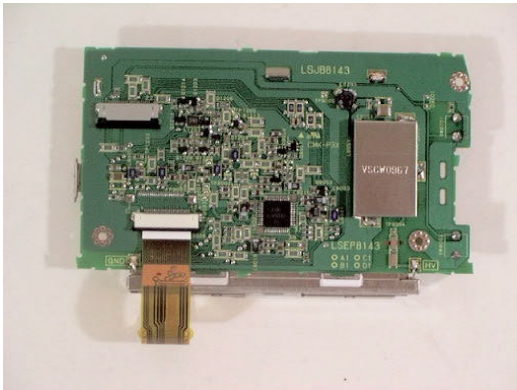
LCD Power PCB (Bottom view / Pulse transformer: ETJ11K114AM)
