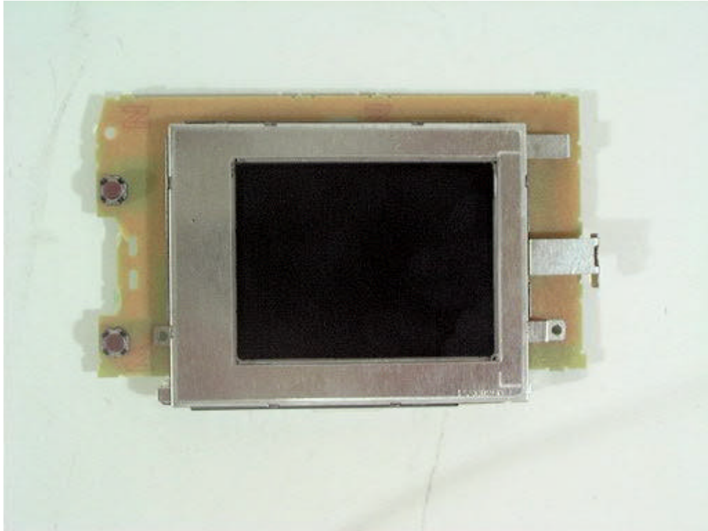
LCD Power PCB (Top view / Pulse transformer: ETJ11K95AM)
