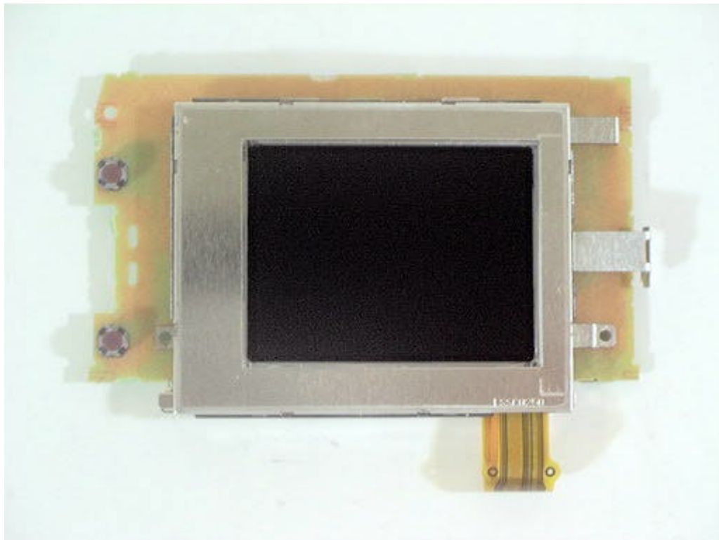
LCD Power PCB (Top view / Pulse transformer: ETJ11K114AM)
