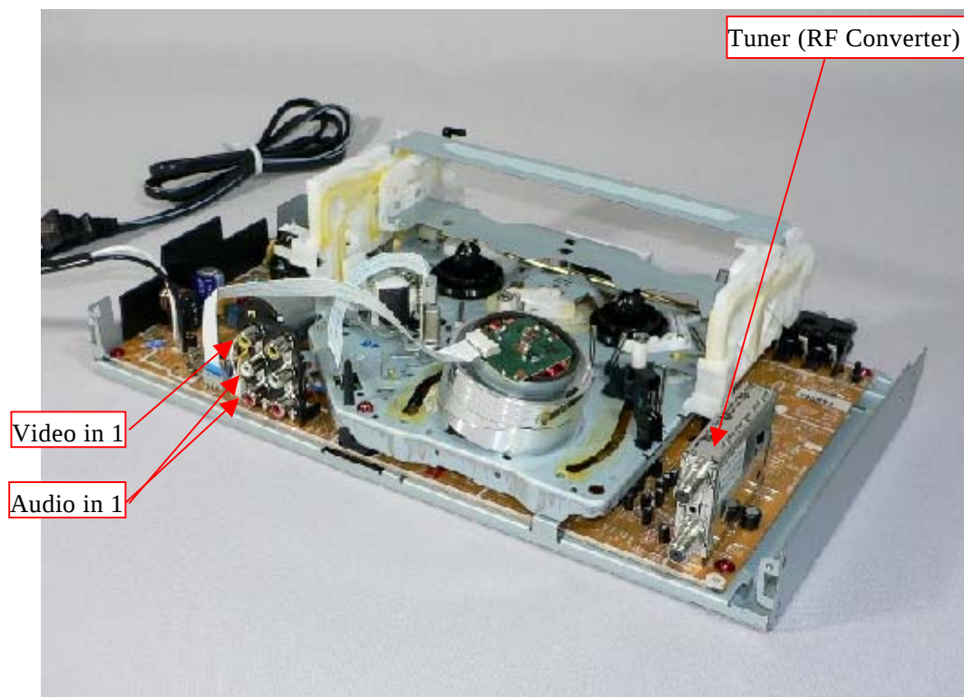
Main PCB (Top view)
