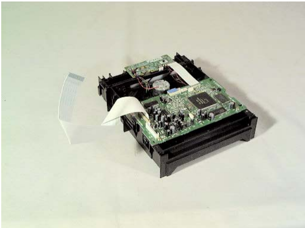
DVD Unit (Bottom view)
