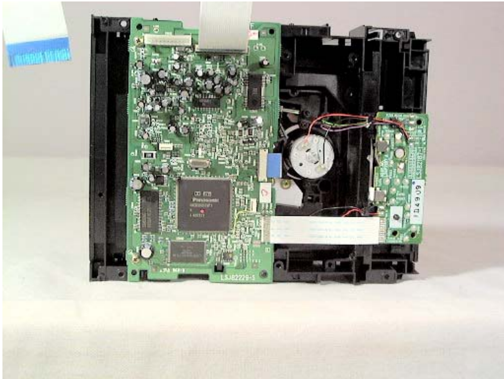
DVD Unit PCB (Top view)
