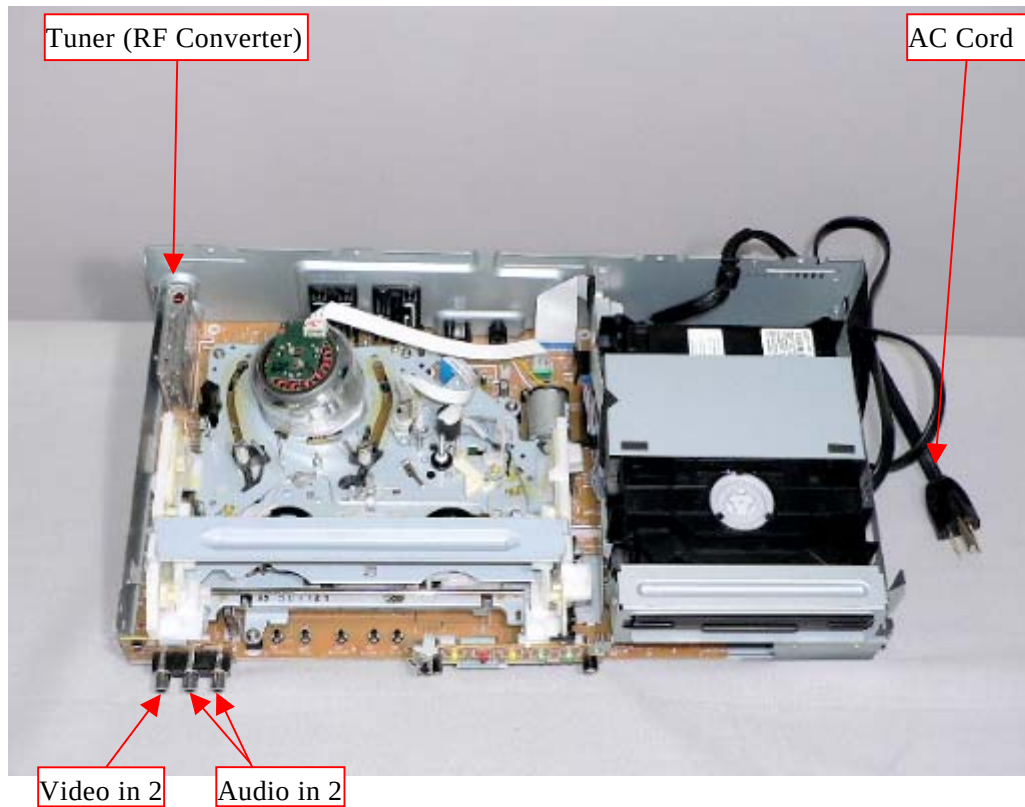
Main PCB (Top view)
