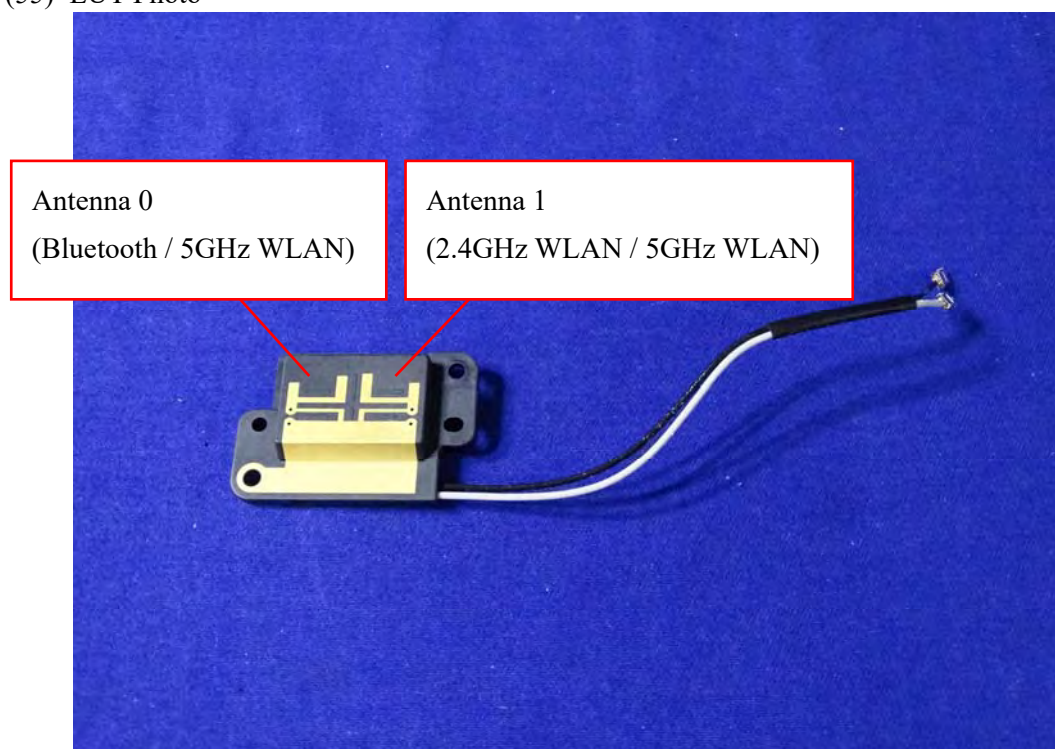
(55) EUT Photo
