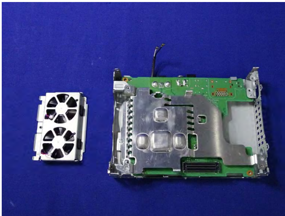
(38) EUT Photo
