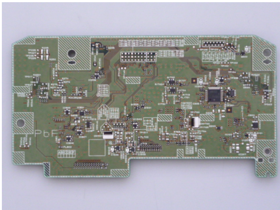
Fig.6 PCB (Back)
