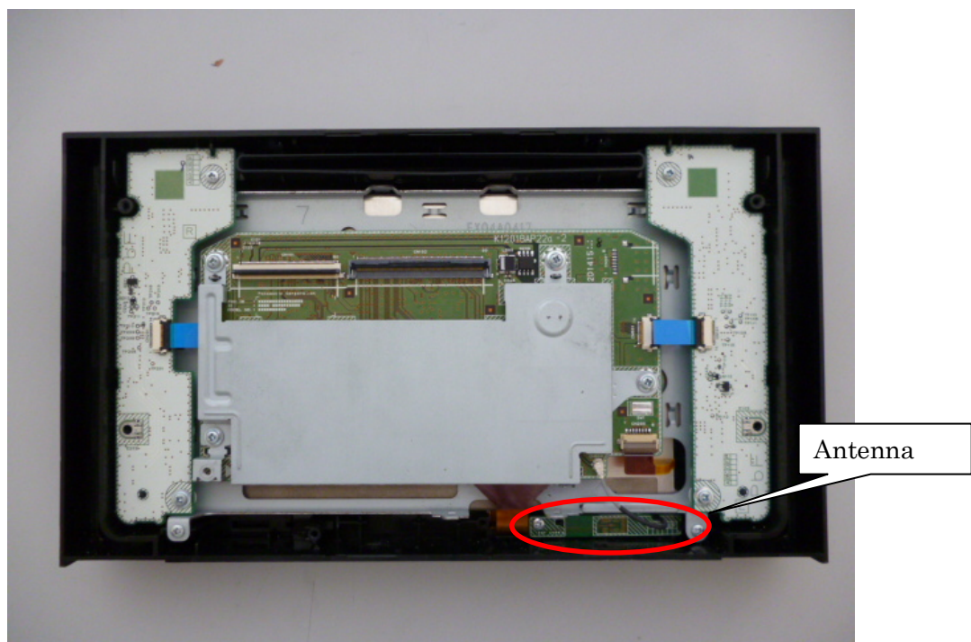
Fig.2 Display ASSY (with Shield)
