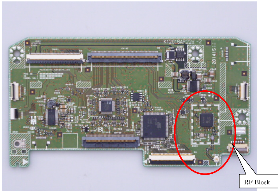
Fig.5 PCB (Surface)
