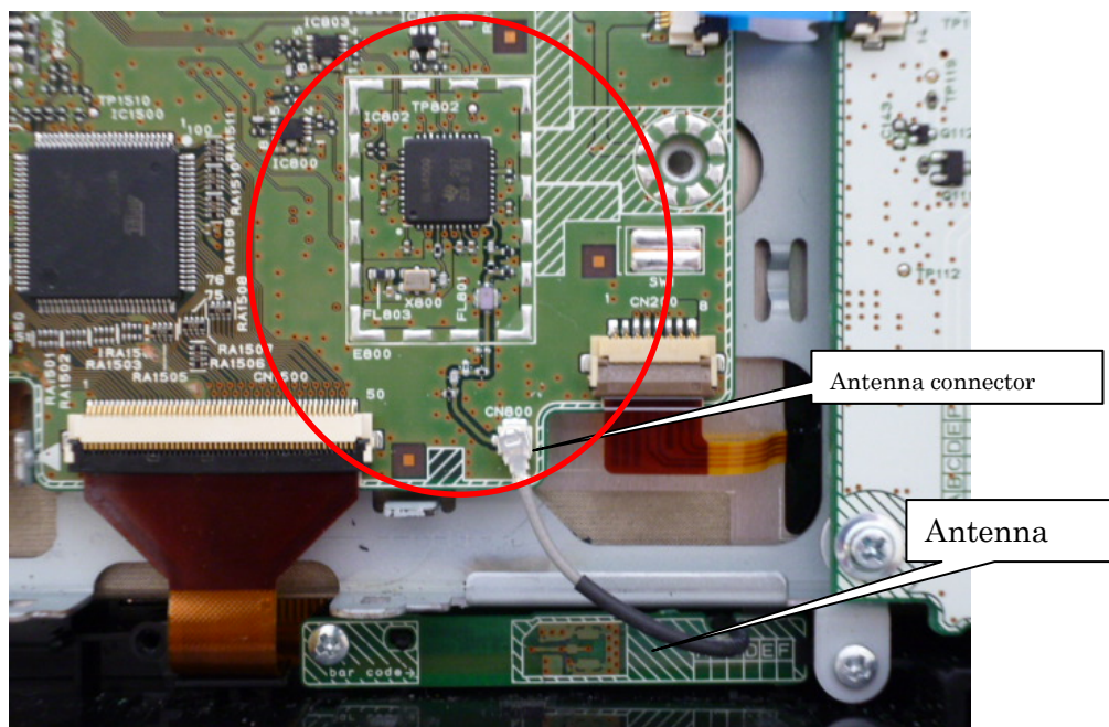
Fig.4 RF Block (without Shield)
