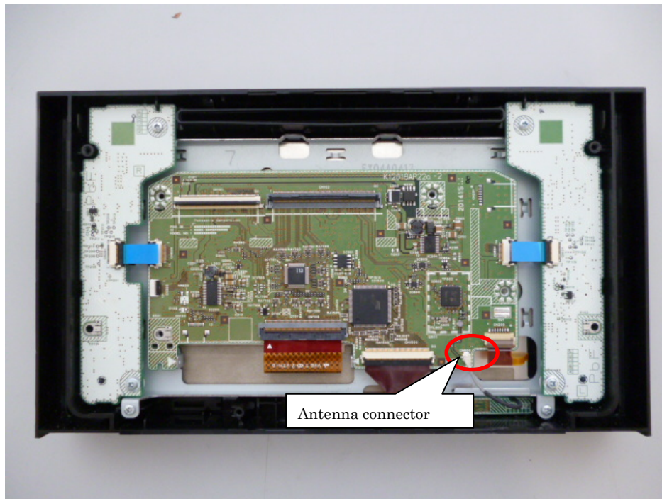
Fig.3 Display ASSY (without Shield)
