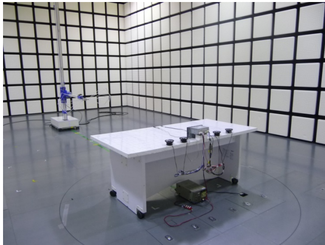
Rear(Below 1GHz)
