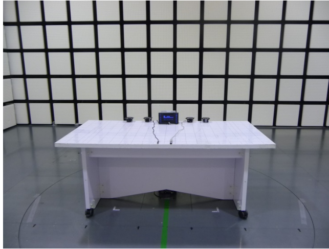
Front(Below 1 GHz)
