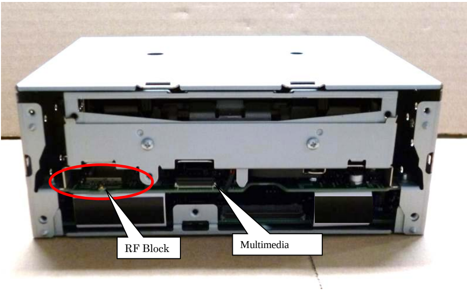
Fig.3 Without Front Plate
