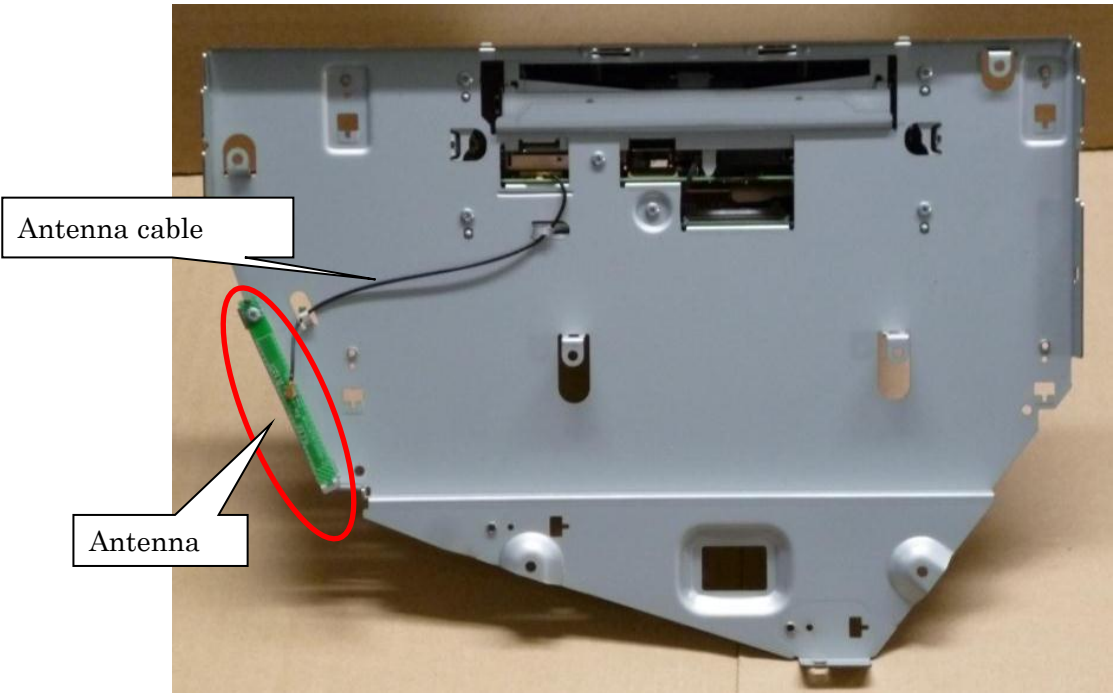
Fig.2 Without Display ASSY
