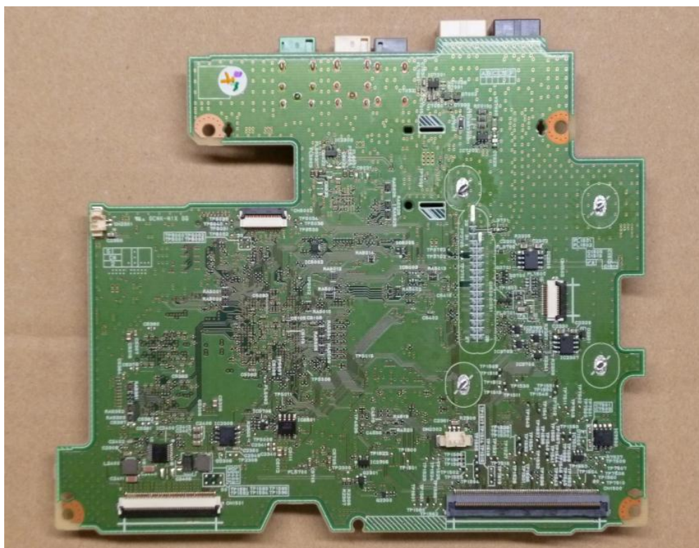
Fig.6 Multimedia PCB (Back side)
