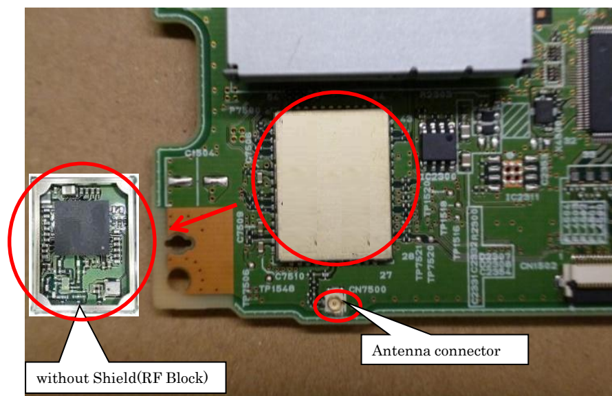
Fig.5 RF Block
