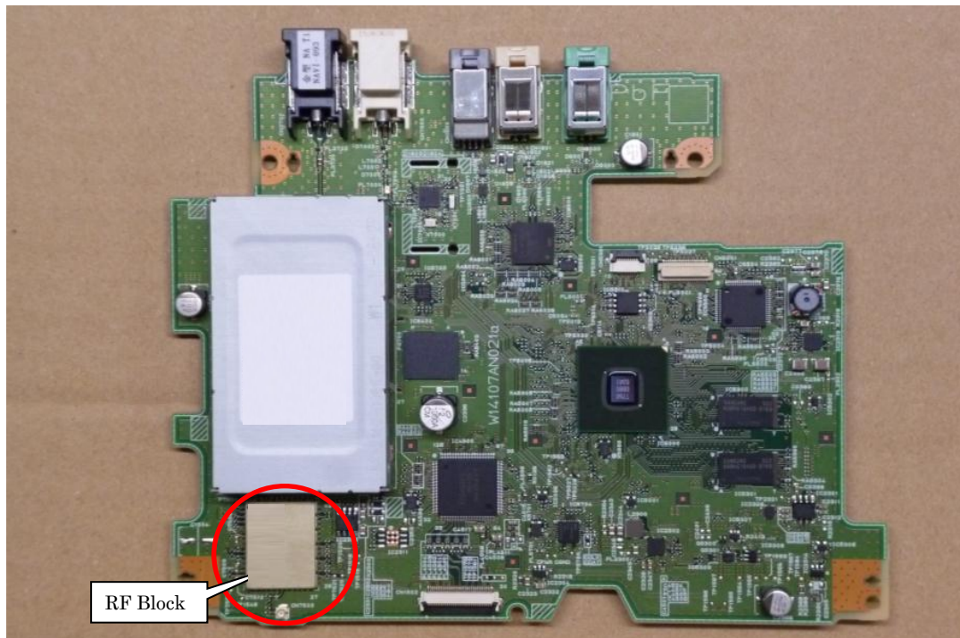
Fig.4 Multimedia PCB (Surface side)
