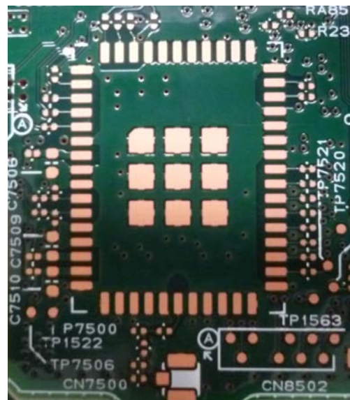
Fig.9 Pattern Resist (Multimedia PCB)
