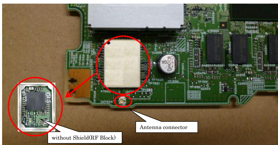
Fig.6 RF Block
