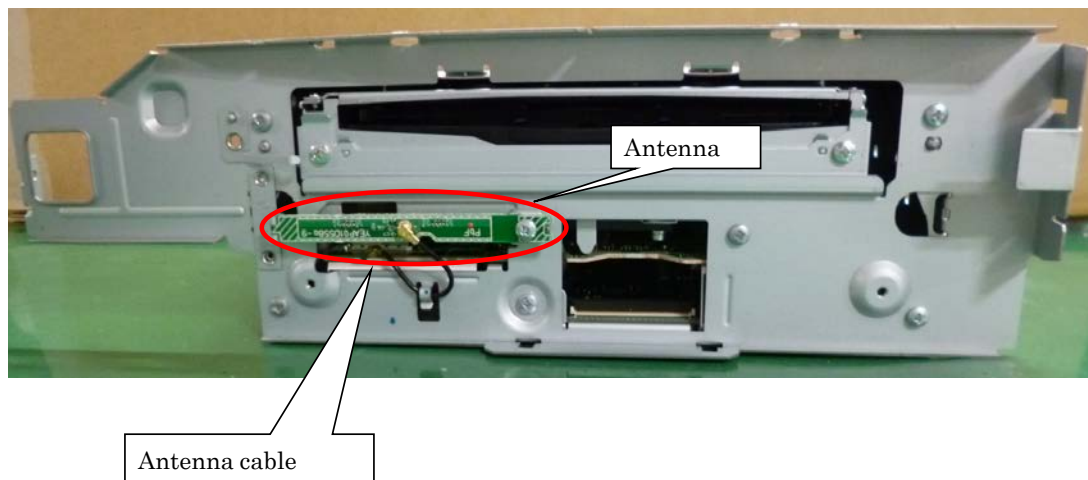
Fig.2 Without Display ASSY
