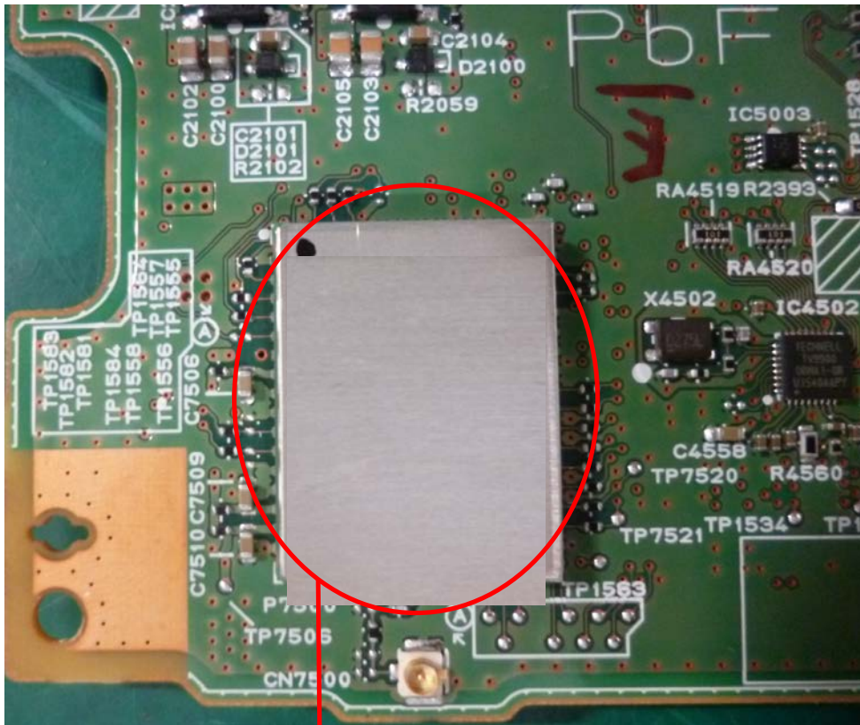
Fig.7 RF Block Detail
