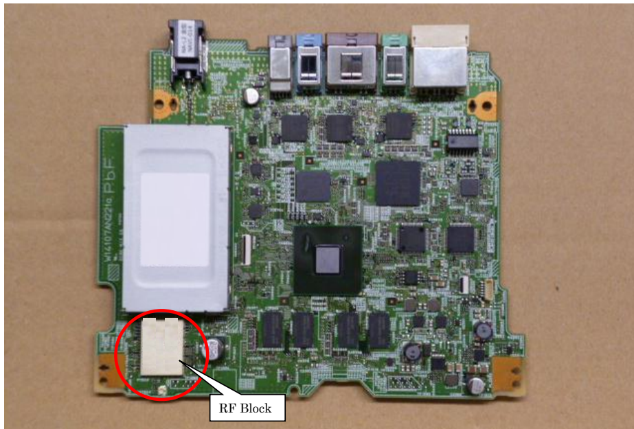
Fig.4 Multimedia PCB (Surface side)
