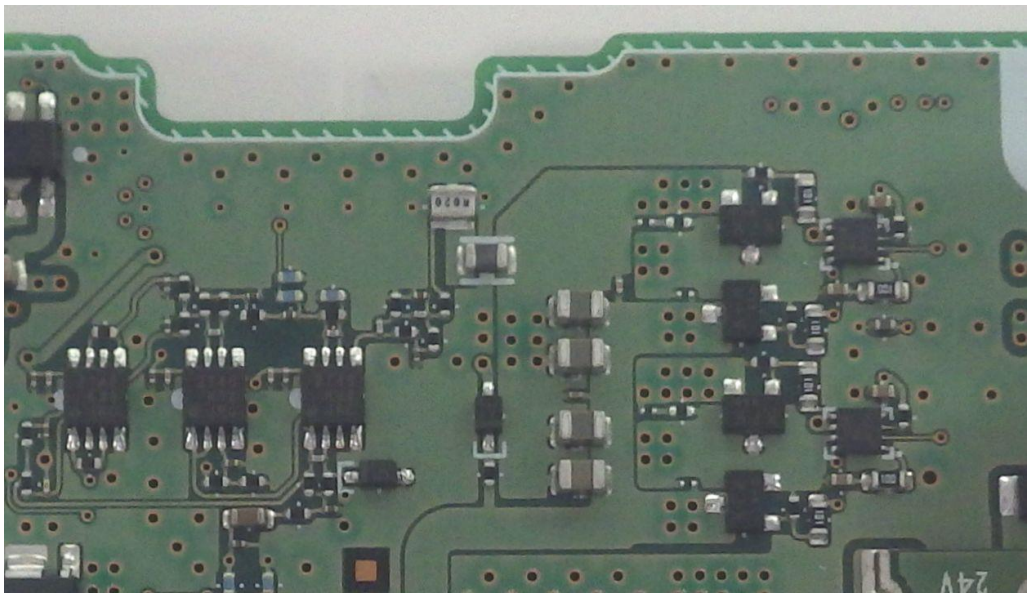
Photo-1. A-Side
