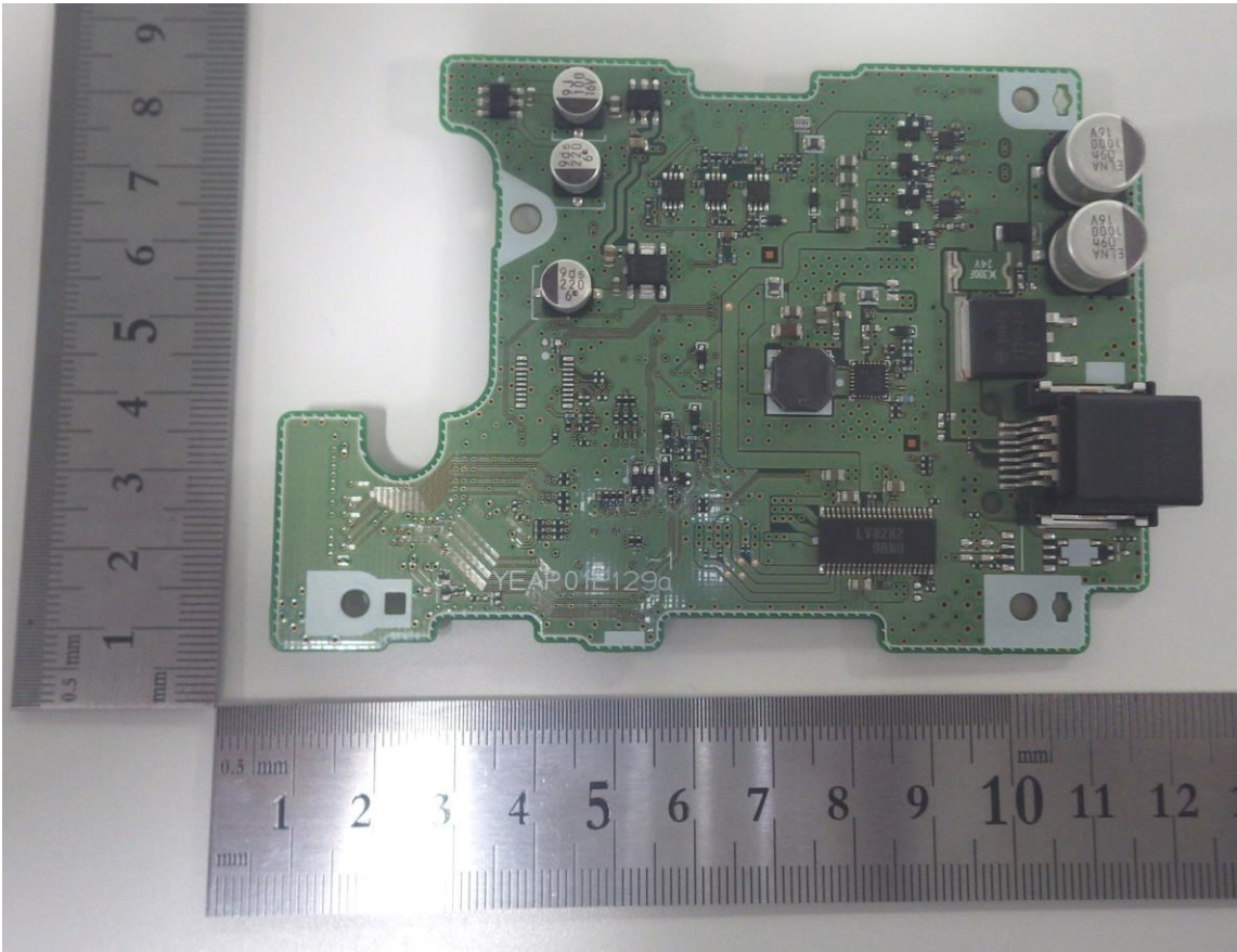
Internal Photo
