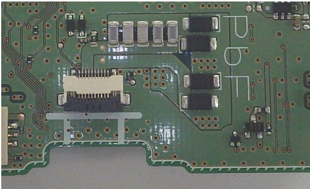
Photo-2. B-Side
