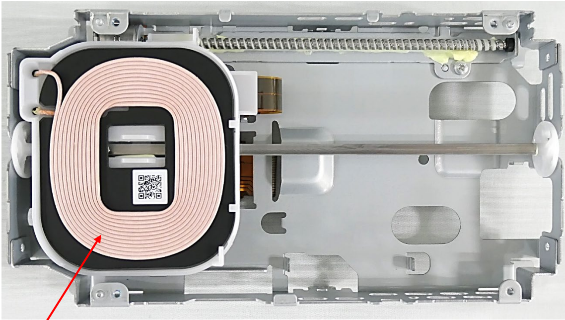
Primary Coil
