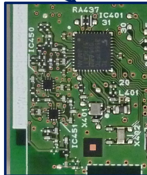
Radio block
