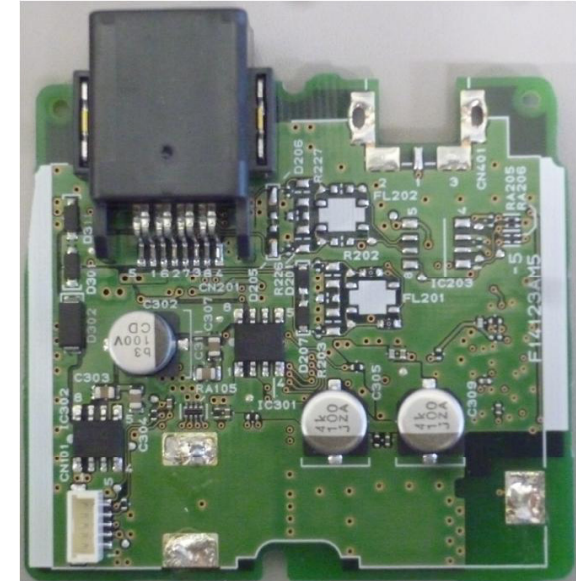
Without antenna (Surface side)
