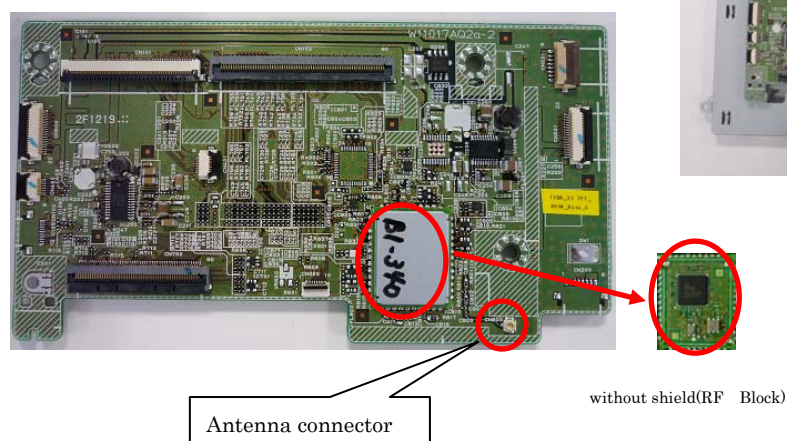
Fig.2 without Shield(Surface)
