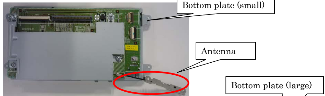
Fig.1 with Shield
