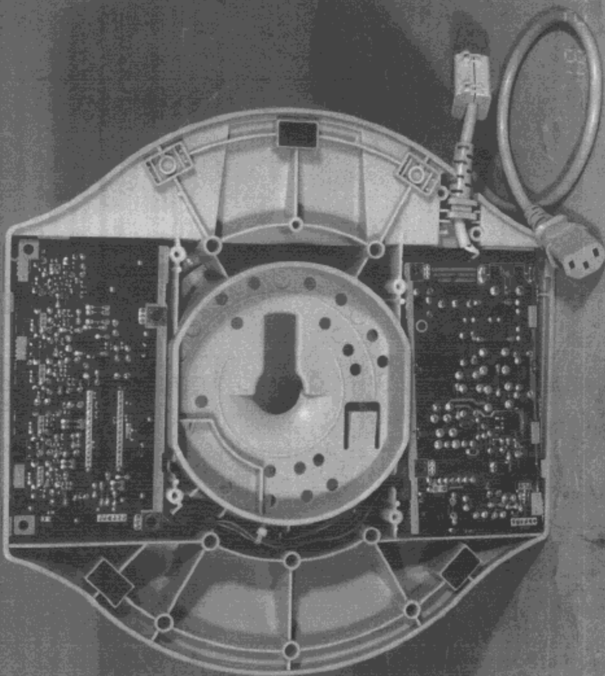
Photo 5. Bottom view with out metal plate of Model No. TY-LD65A
