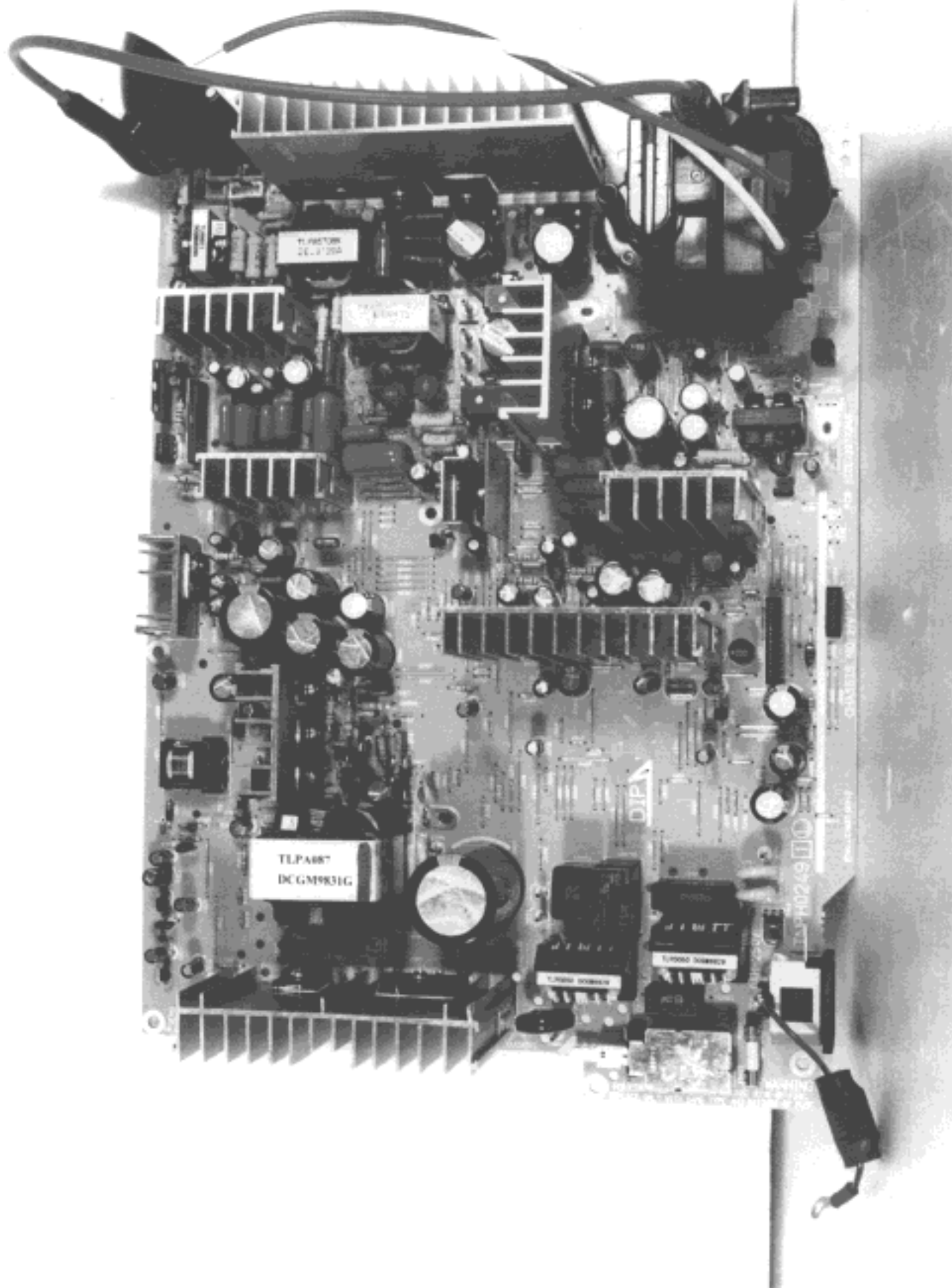
Photo 6. Main and Power Supply PWB (Part side) of TX-D1F64NM
