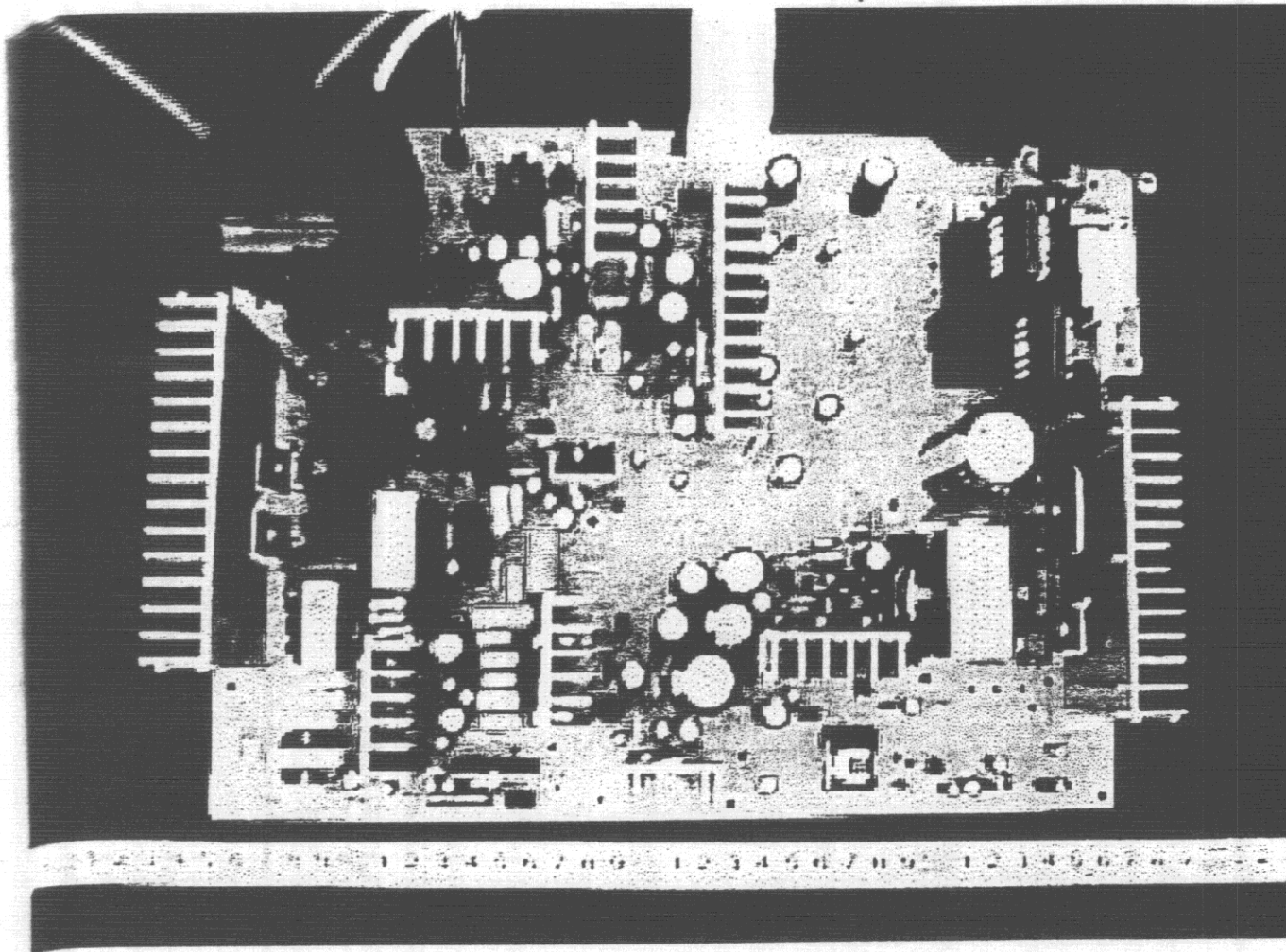
Figure 9.7-1 Power Board Surface
