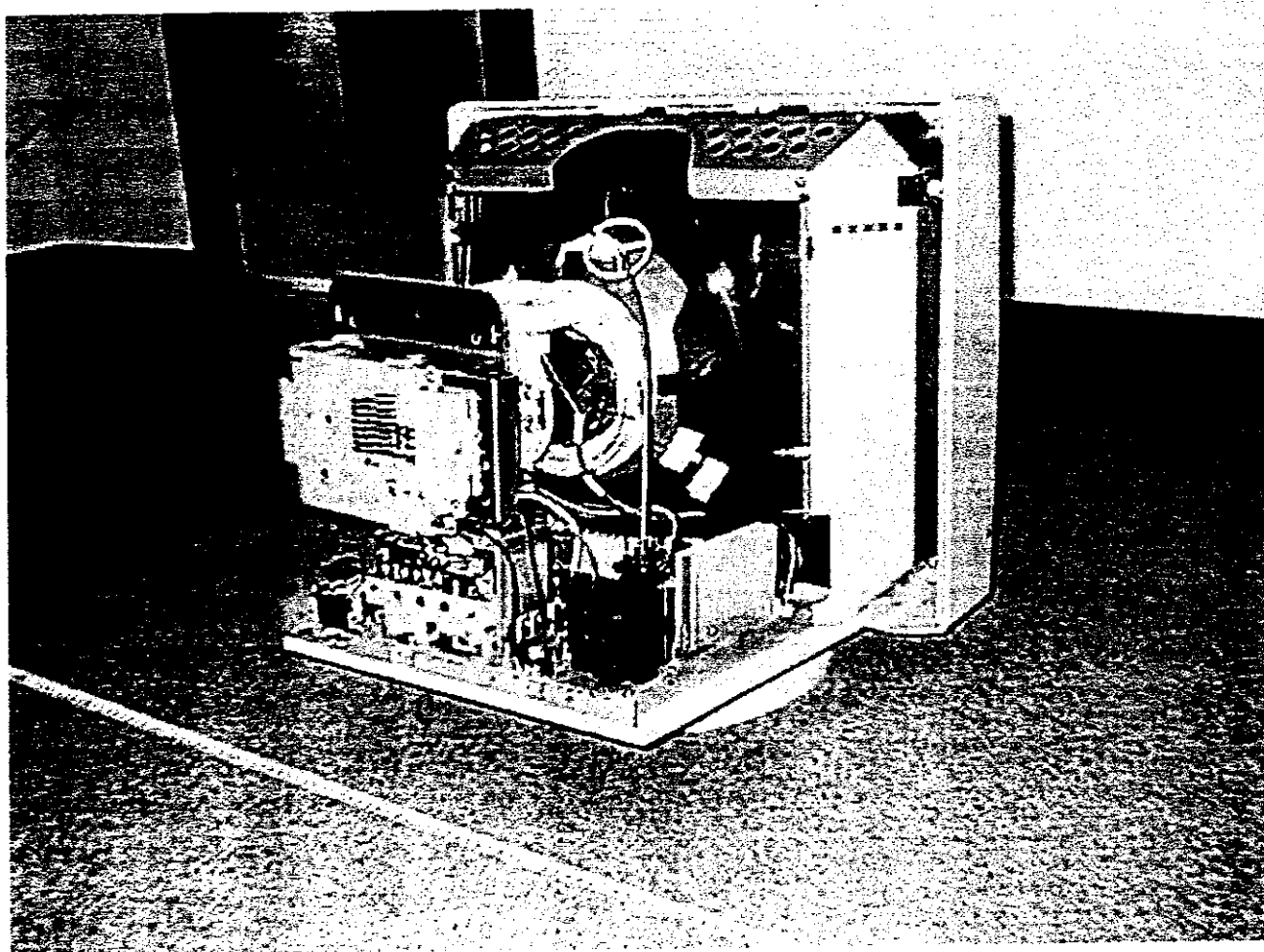
Figure 9.4 Unit disassembly
