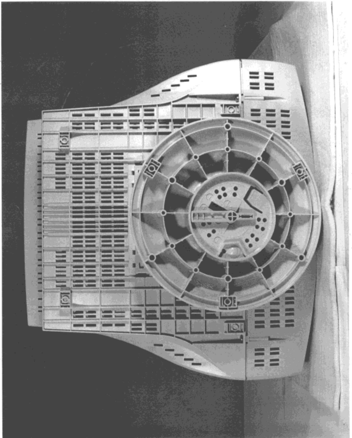
Photo 3. Bottom view of TX-D9S55NM
