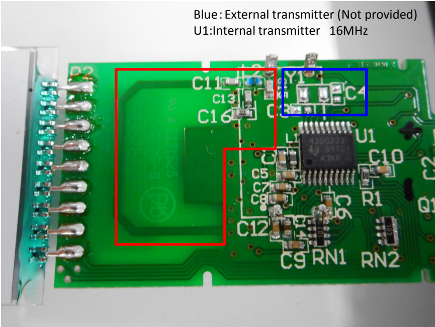
RF Module and Antenna
