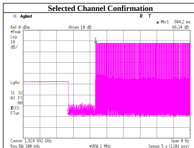
Selected Channel Confirmation, Connection 804.2 msec after interferer removed.
