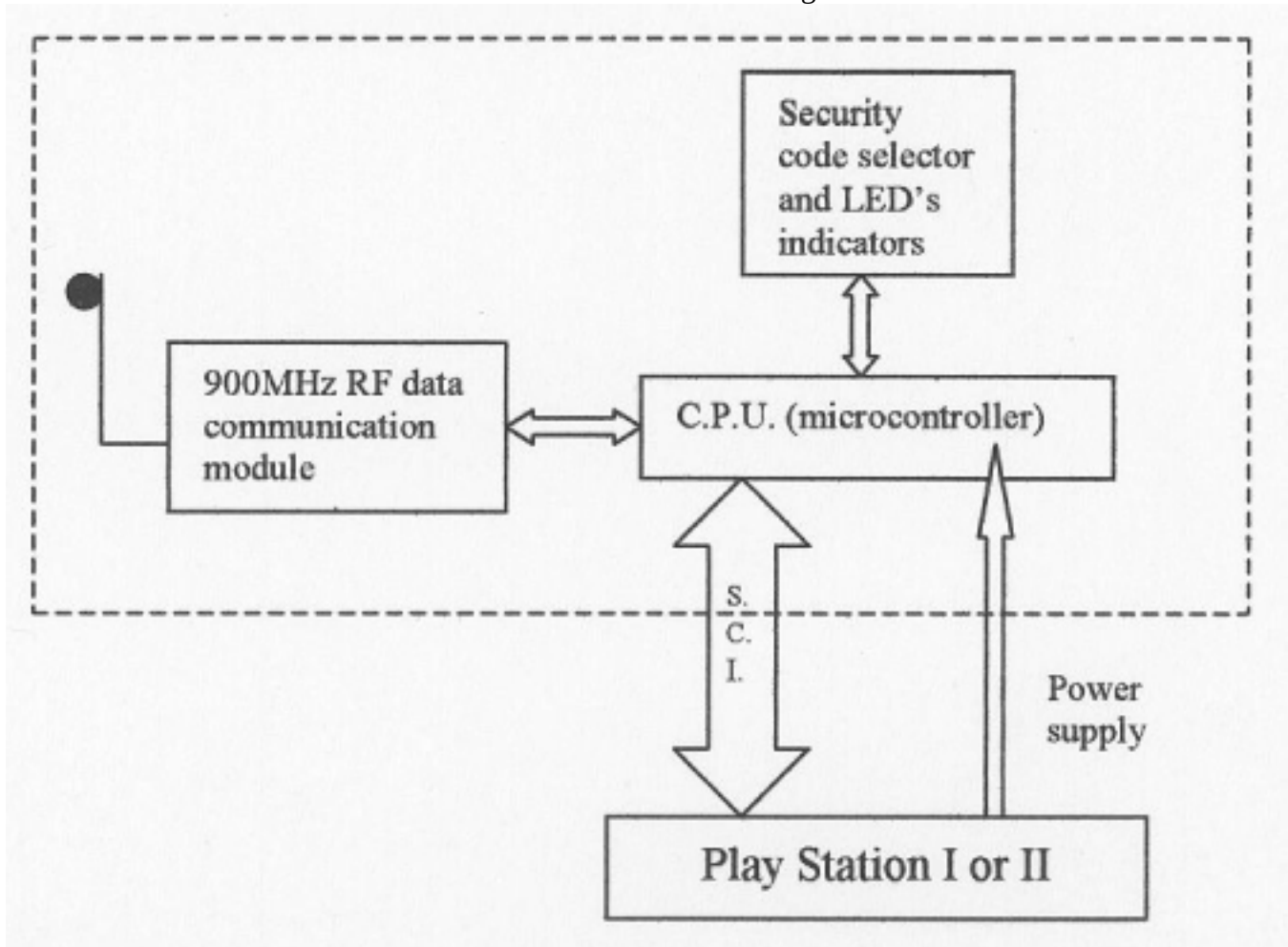
900MHz Base Unit Block Diagram
