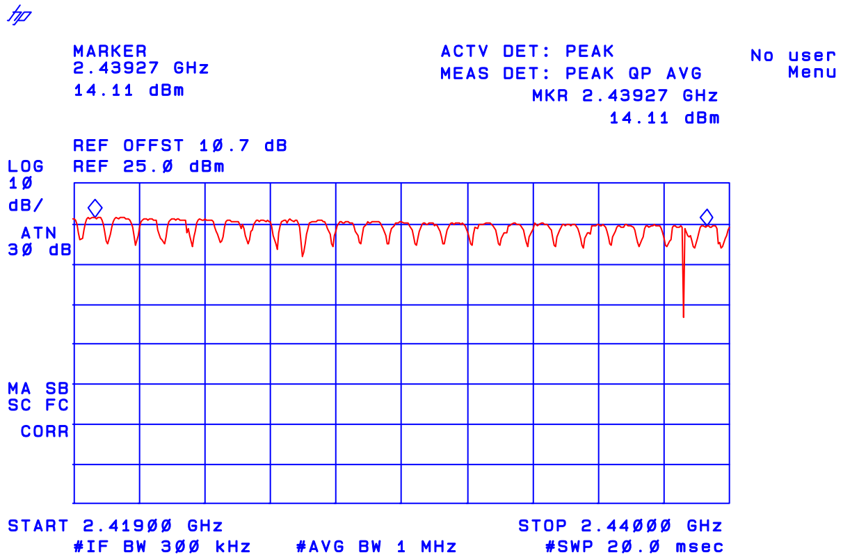
Plot 8: Number of Hopping Frequencies
