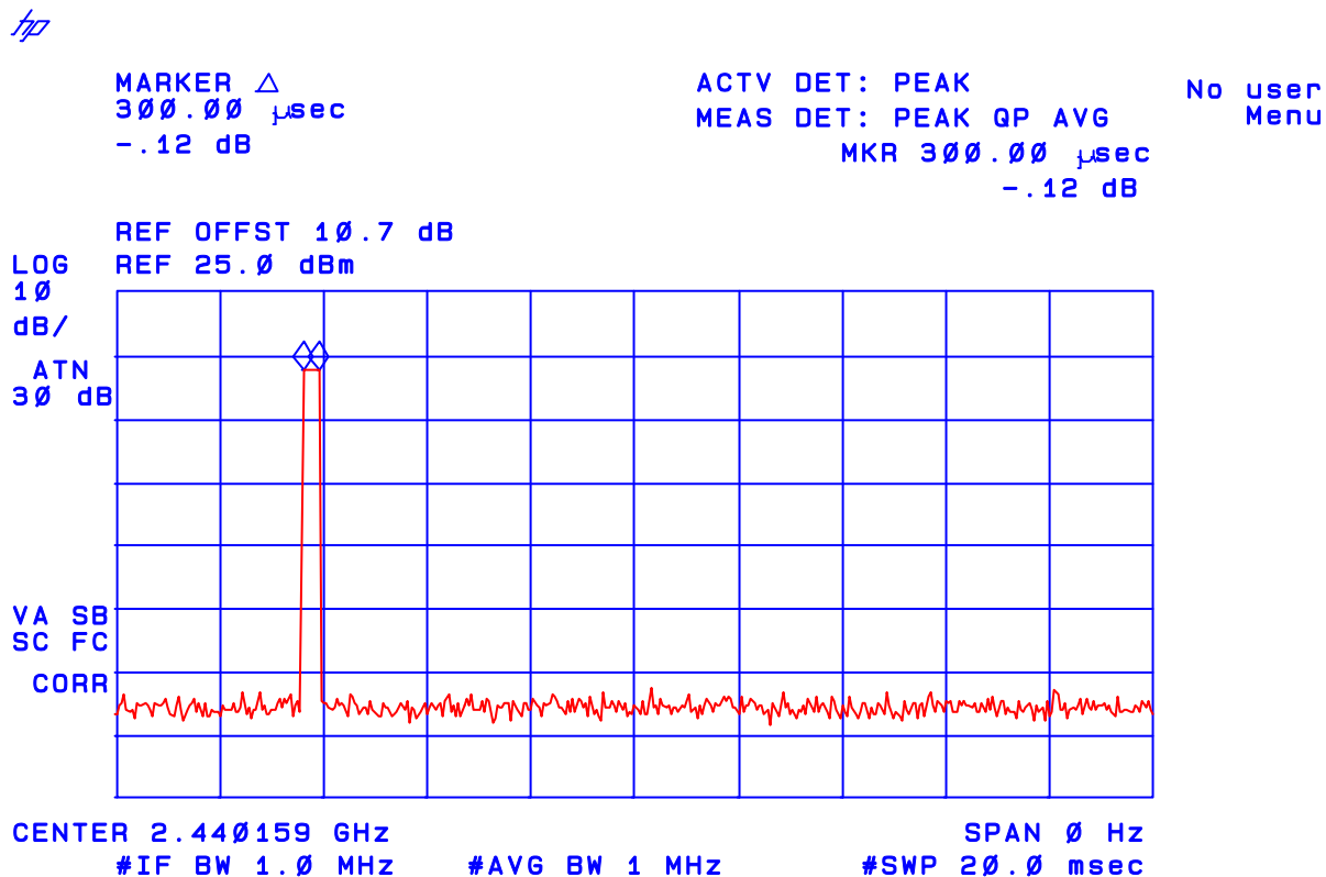
Plot 13: Average Time of Occupancy Frequency: 2440.158968 MHz (CH 45)
