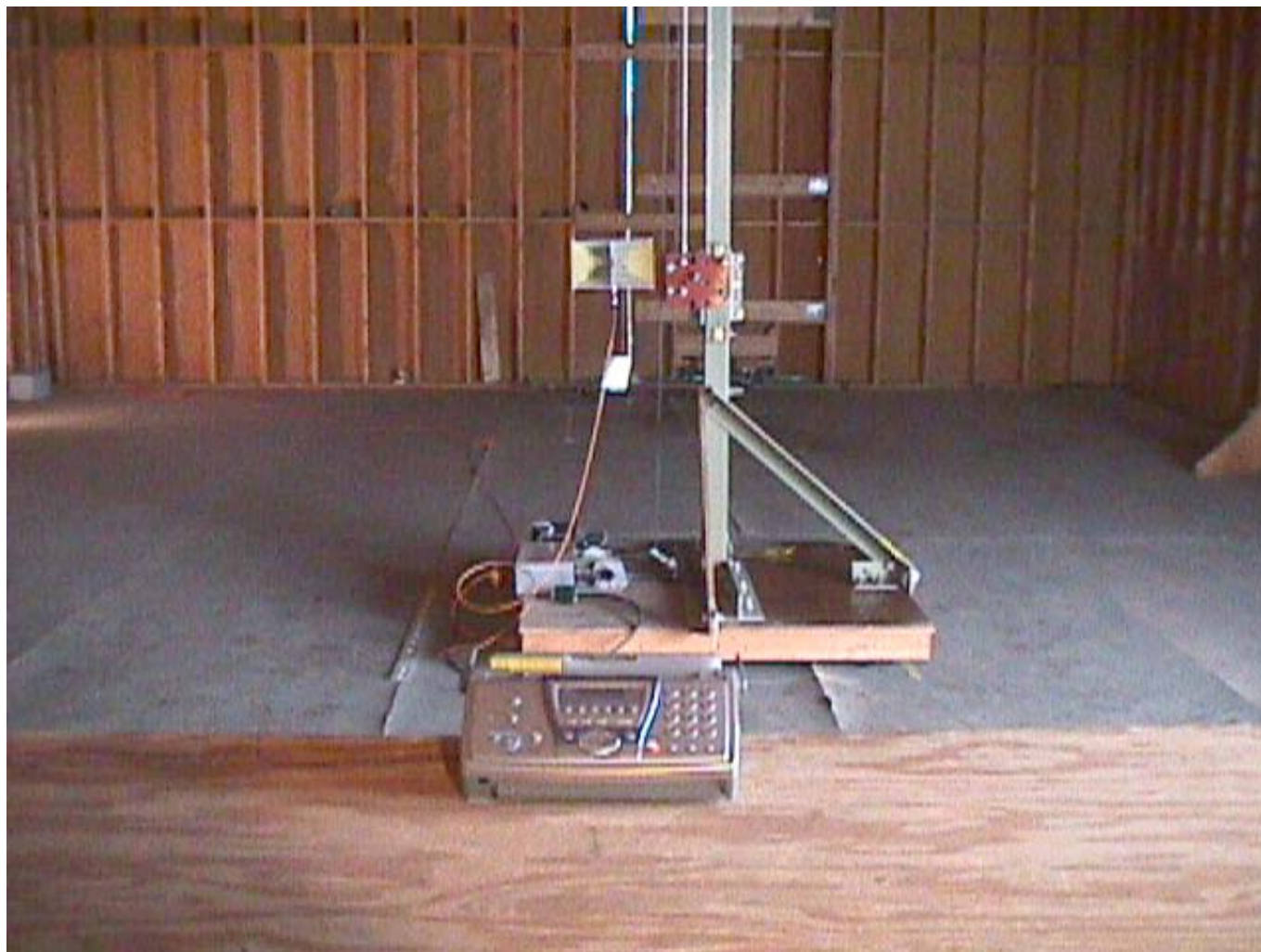
Transmitter Radiated Emissions at 3 Meters
