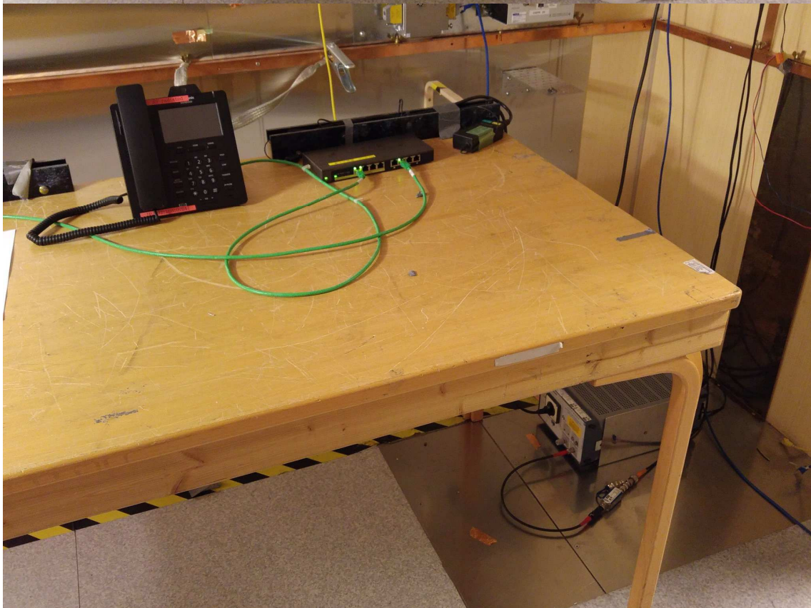
Power line Conducted Emissions Test
