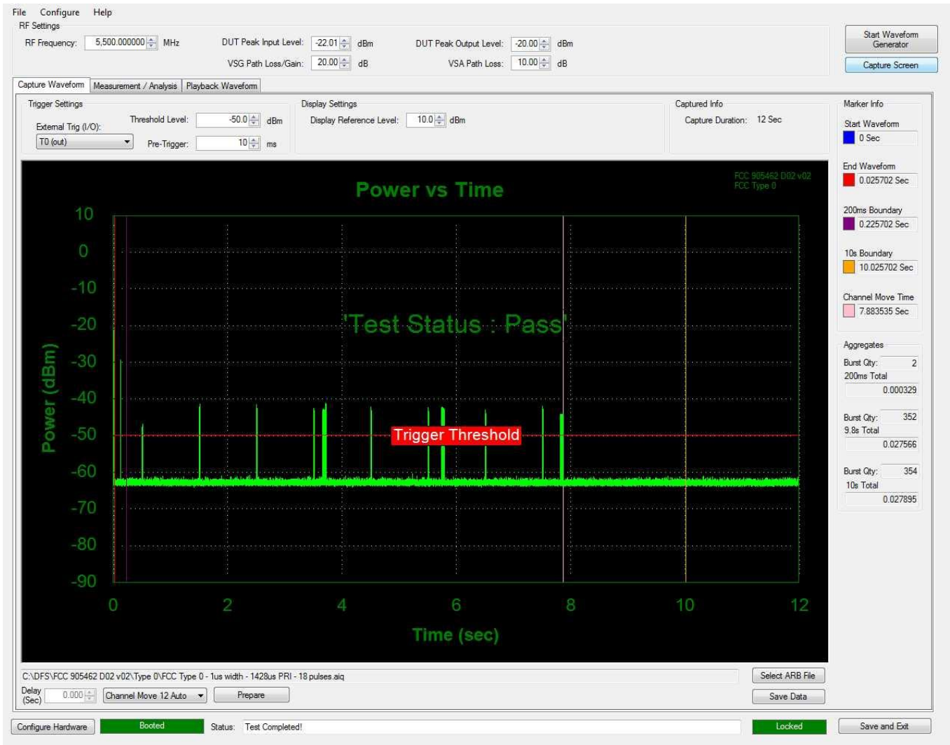
Figure 8.1-1: Channel closing transmission and move time
