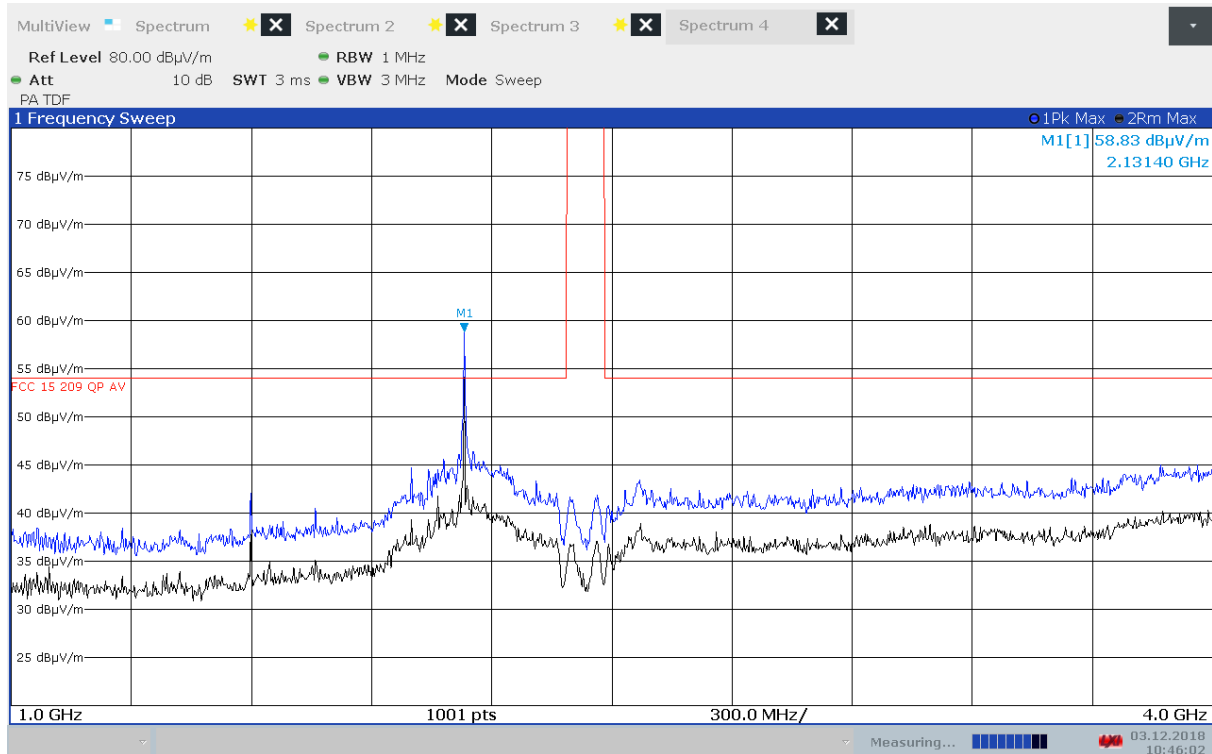
Radiated Emissions, 1000 -4000 MHz, 2412 MHz, VP, 802.11n, MCS0
