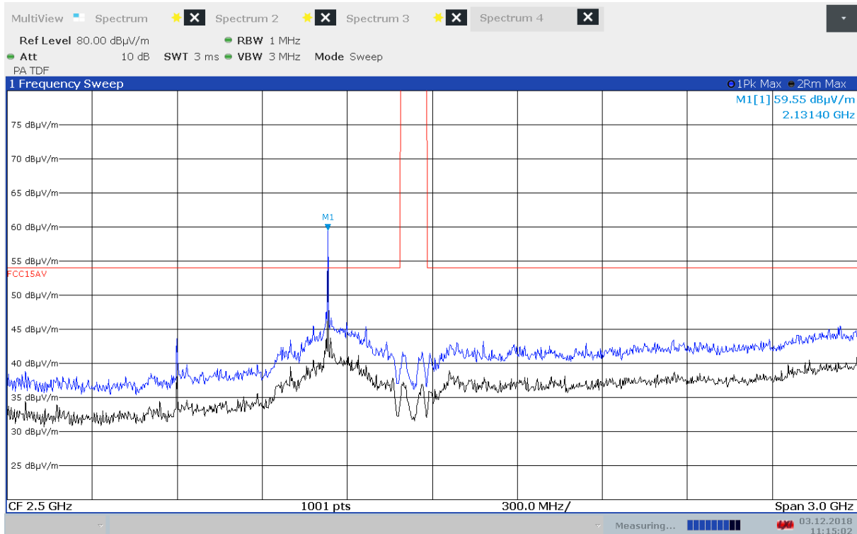
Radiated Emissions, 1000 -4000 MHz, 2462 MHz, VP, 802.11g, 6Mbps
