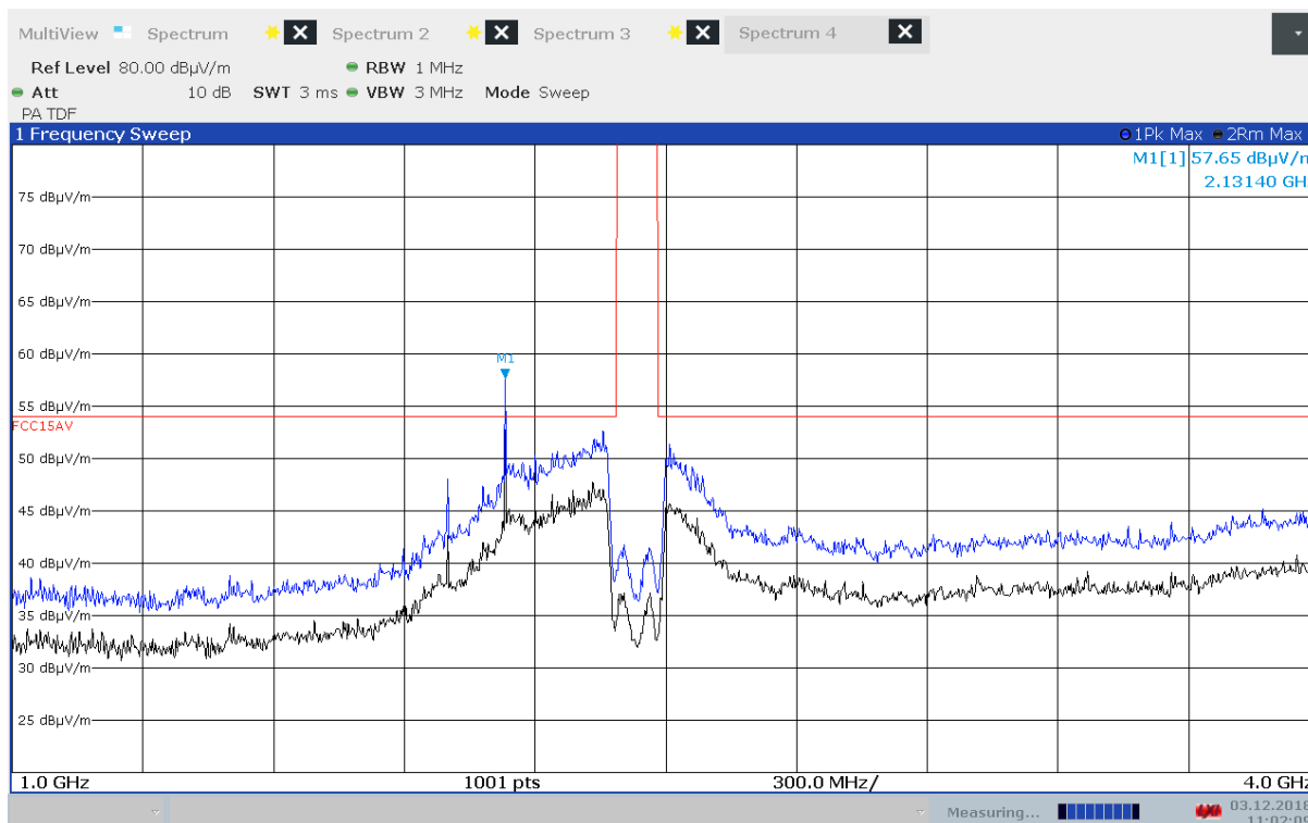
Radiated Emissions, 1000 -4000 MHz, 2412 MHz, HP, 802.11g, 6Mbps
