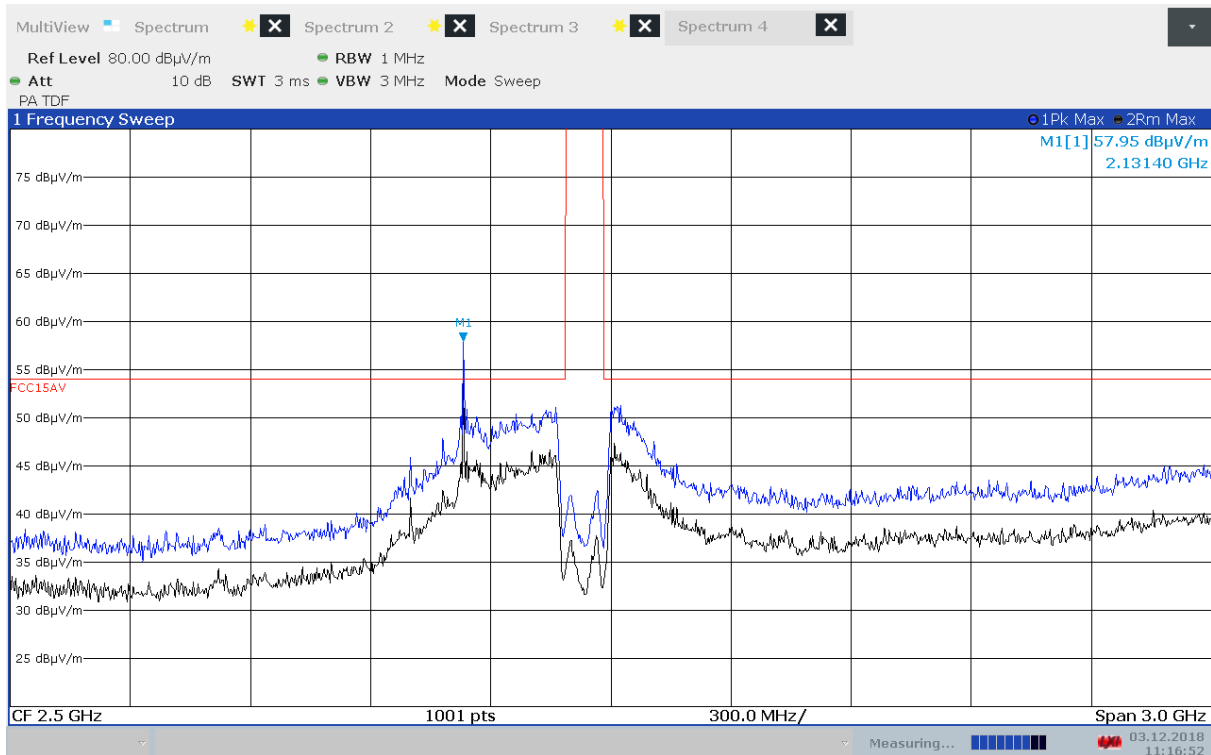
Radiated Emissions, 1000 -4000 MHz, 2462 MHz, HP, 802.11g, 6Mbps
