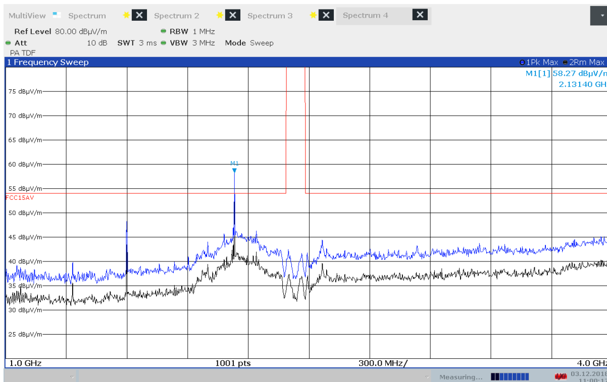
Radiated Emissions, 1000 -4000 MHz, 2412 MHz, VP, 802.11g, 6Mbps
