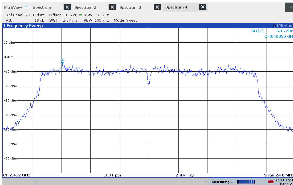
PSD, 2412 MHz, 802.11n, MCS0
