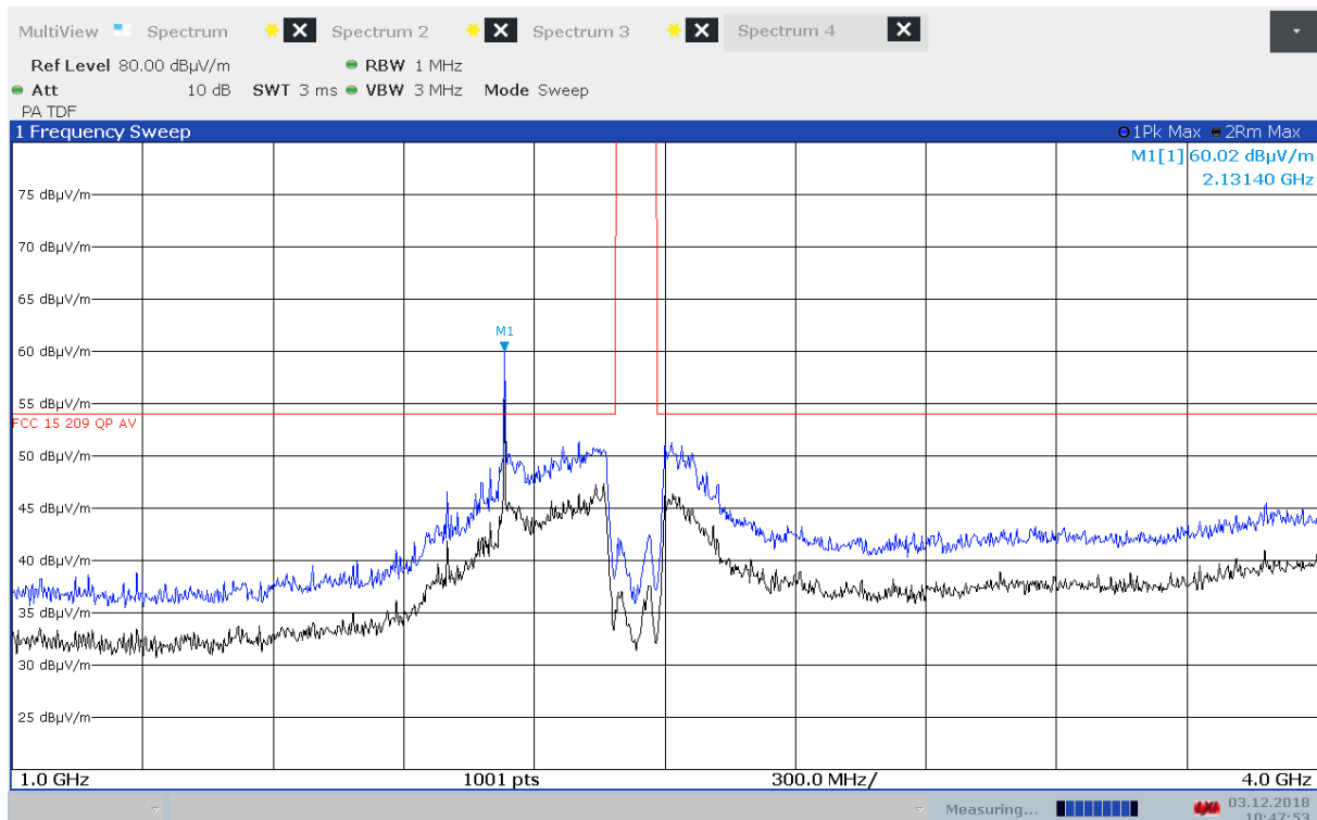
Radiated Emissions, 1000 -4000 MHz, 2412 MHz, HP, 802.11n, MCS0
