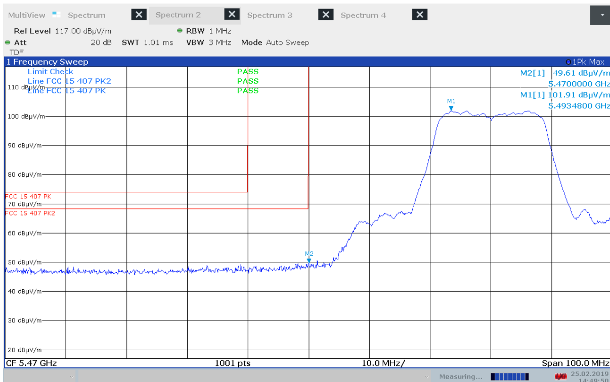
Unwanted Emissions, Band Edge, 5470 MHz, Ch100, 802.11n MCS0, Radiated
