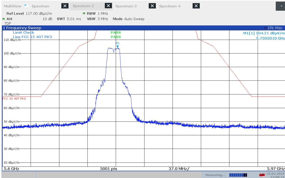
Unwanted Emissions, Band Edge, 5725 MHz, Ch149, 802.11a 6Mbps, Radiated
