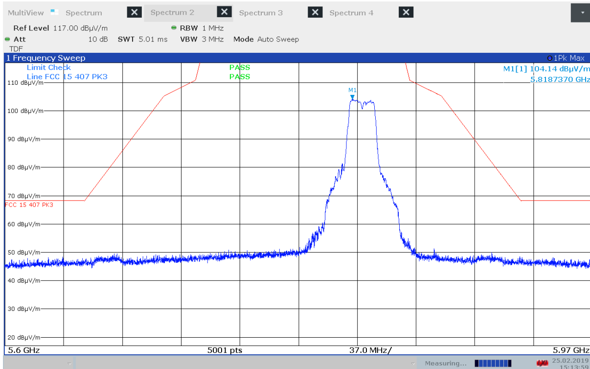
Unwanted Emissions, Band Edge, 5825 MHz, Ch165, 802.11a 6Mbps, Radiated
