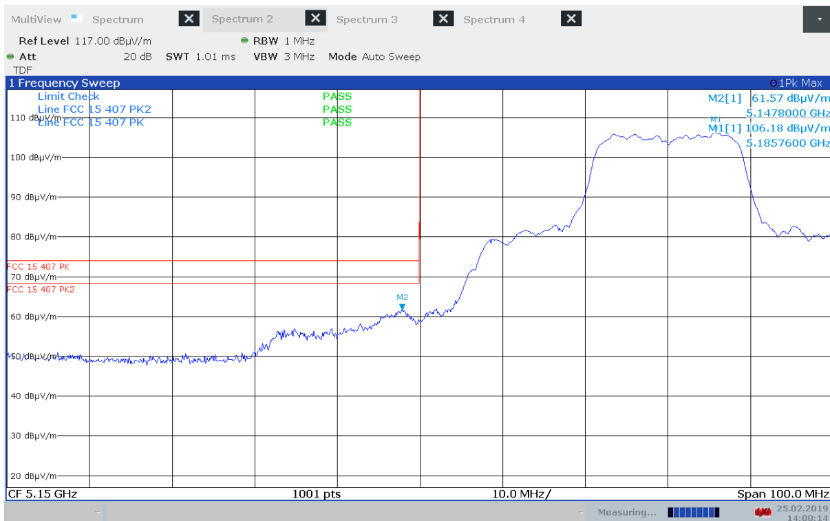
Unwanted Emissions, Band Edge, 5150 MHz, Ch036, 802.11n MCS0, Radiated
