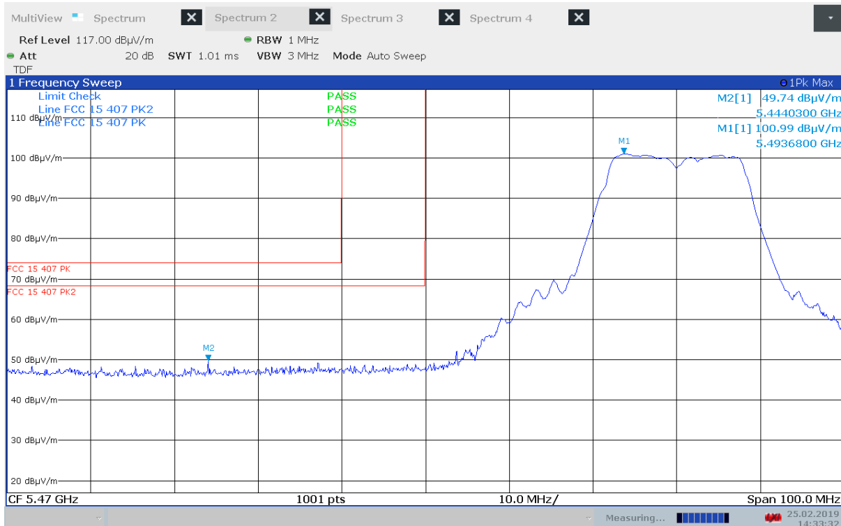
Unwanted Emissions, Band Edge, 5470 MHz, Ch100, 802.11a 6Mbps, Radiated
