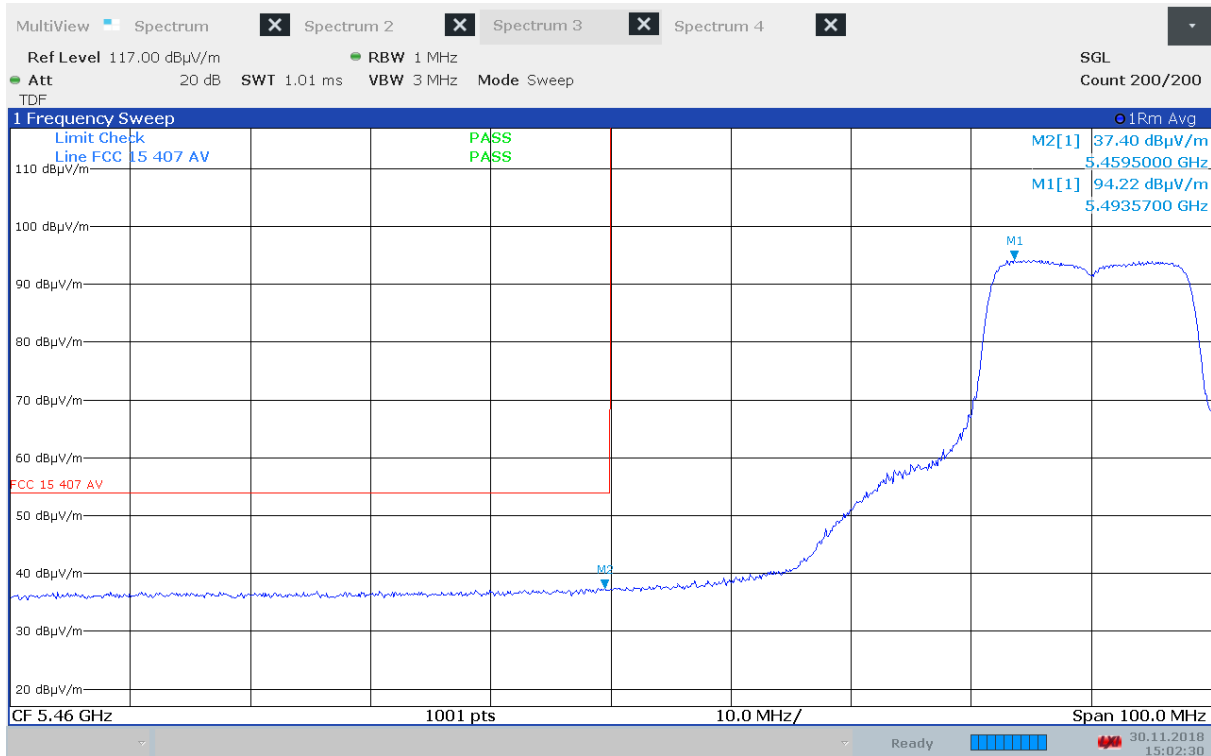
Band Edge, 5460 MHz, 5500 MHz, 802.11a 6Mbps, EUT V (Max: VP), Average
