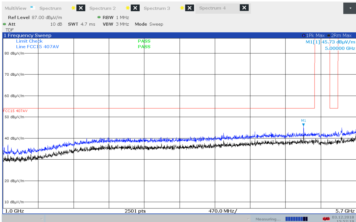
Radiated Emissions, 1000 - 5700 MHz, 5745 MHz, 802.11a 6Mbps, EUT V, VP
