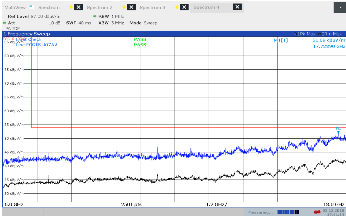
Radiated Emissions, 6000 - 18000 MHz, 5700 MHz, 802.11n MCS0, EUT V, HP
