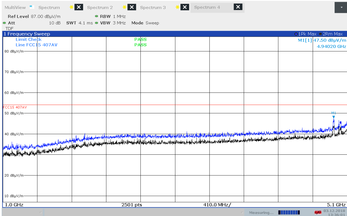
Radiated Emissions, 1000 - 5100 MHz, 5180 MHz, 802.11n MCS0, EUT V, HP
