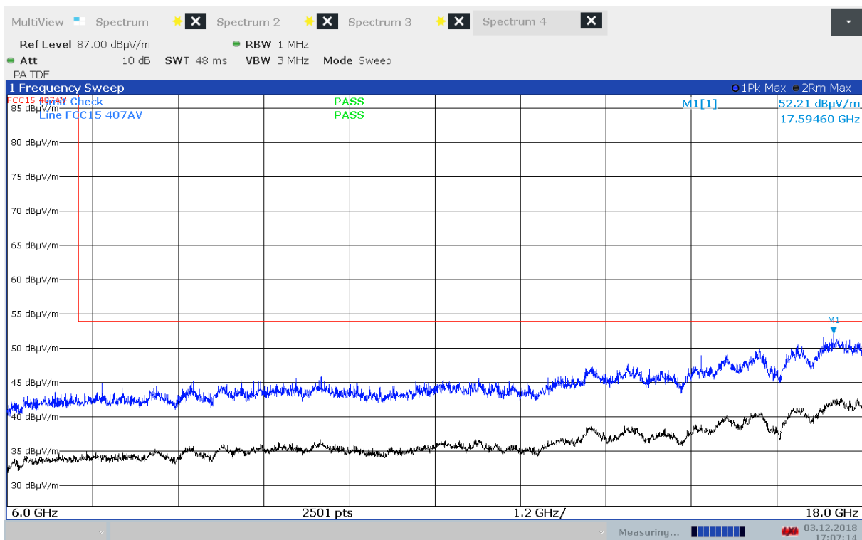
Radiated Emissions, 6000 - 18000 MHz, 5500 MHz, 802.11n MCS0, EUT V, HP
