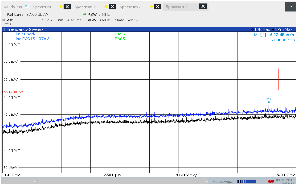
Radiated Emissions, 1000 - 5410 MHz, 5500 MHz, 802.11n MCS0, EUT V, VP
