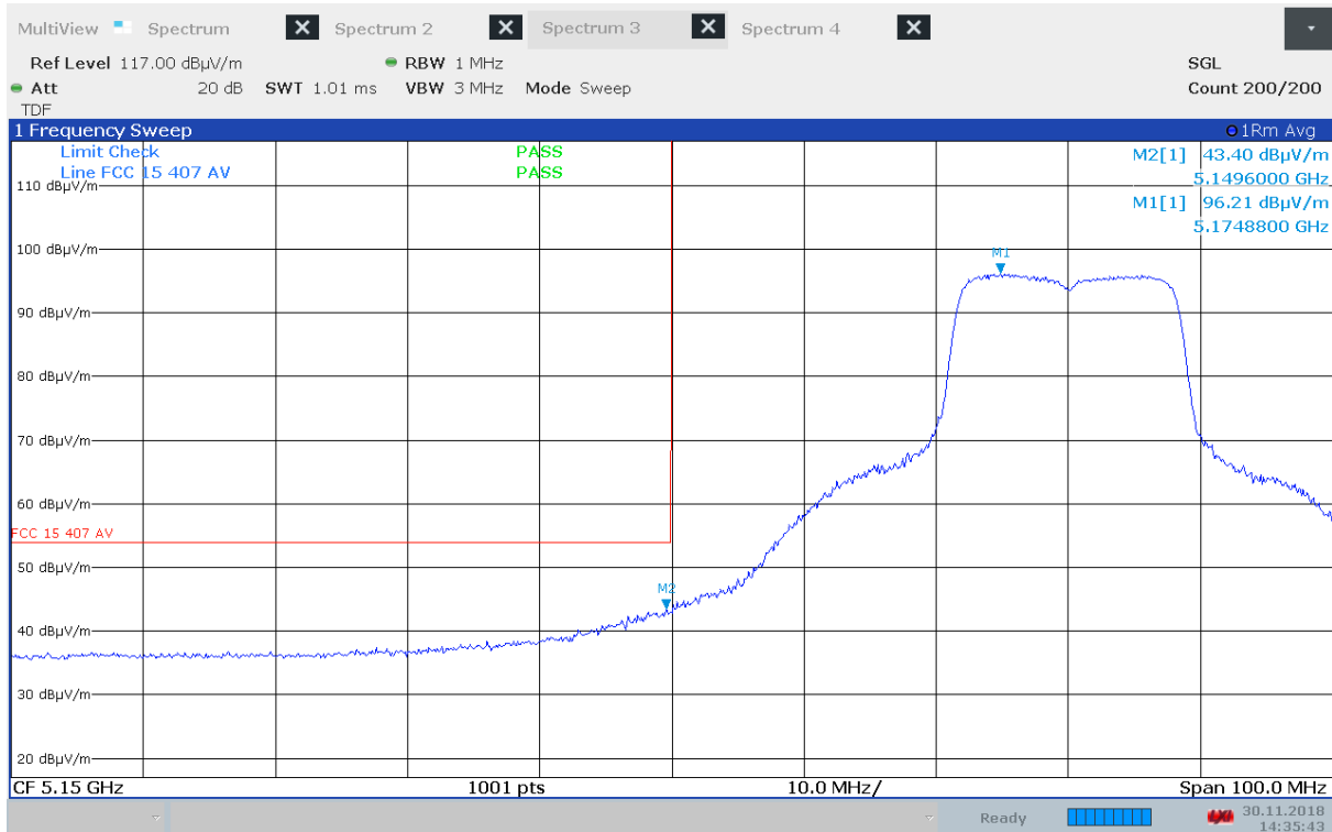
Band Edge, 5150 MHz, Ch036, 802.11a 6Mbps, EUT V (Max: VP), Average
