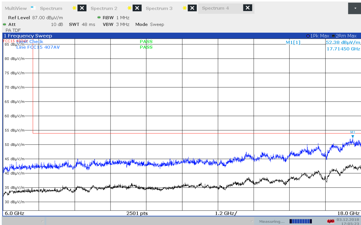
Radiated Emissions, 6000 - 18000 MHz, 5500 MHz, 802.11n MCS0, EUT V, VP
