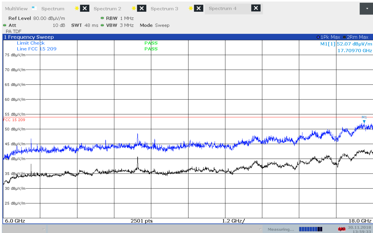
Radiated Emissions, 6000 - 18000 MHz, 5180 MHz, 802.11a 6Mbps, EUT V, VP
