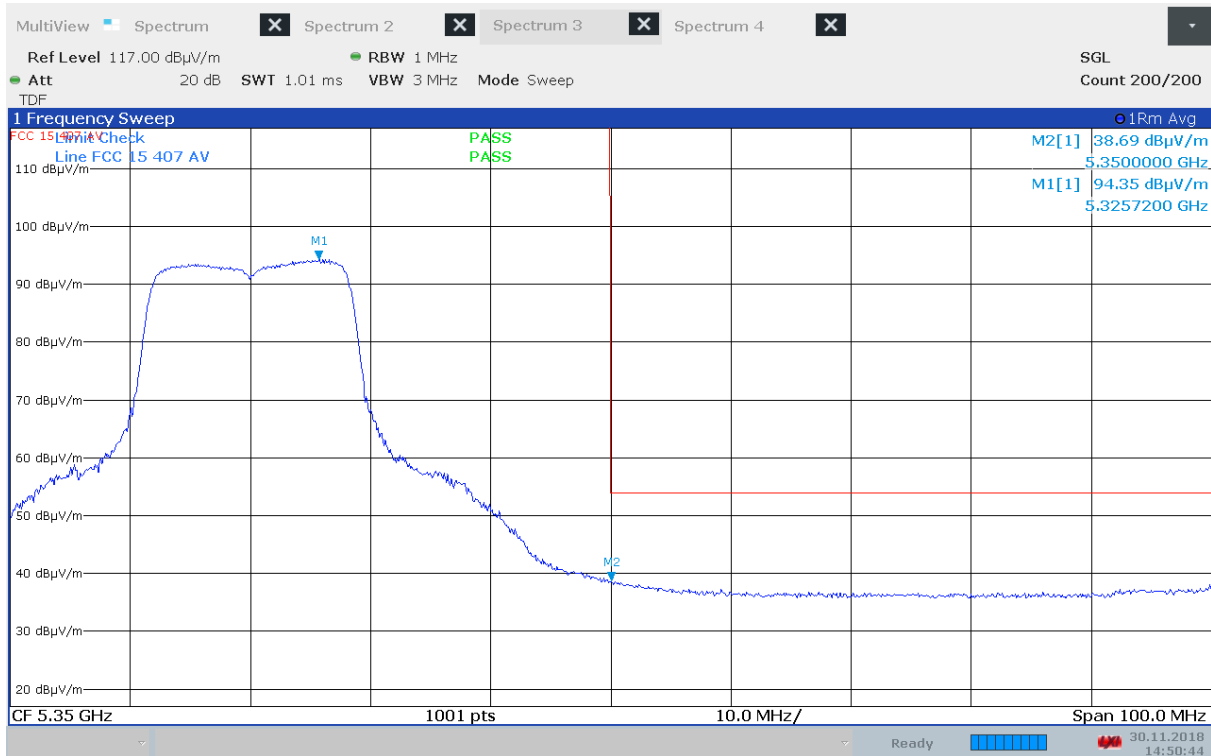
Band Edge, 5350 MHz, 5320 MHz, 802.11a 6Mbps, EUT V (Max: VP), Average
