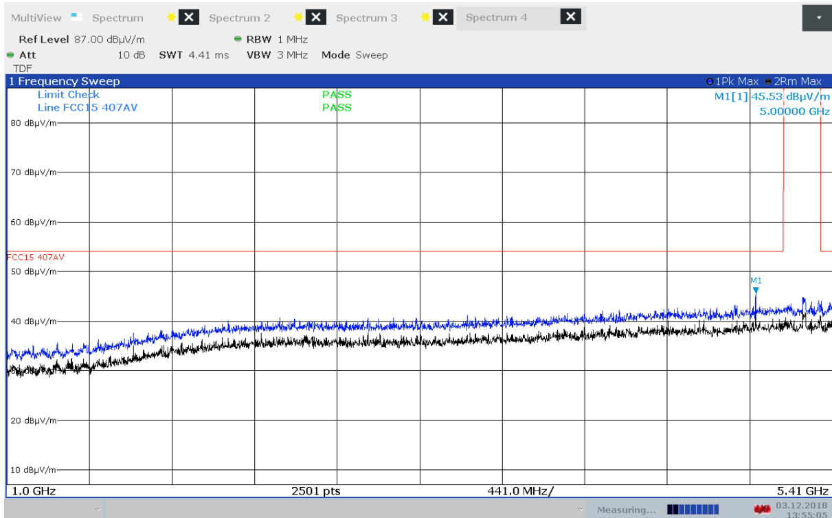
Radiated Emissions, 1000 - 5410 MHz, 5500 MHz, 802.11n MCS0, EUT V, HP
