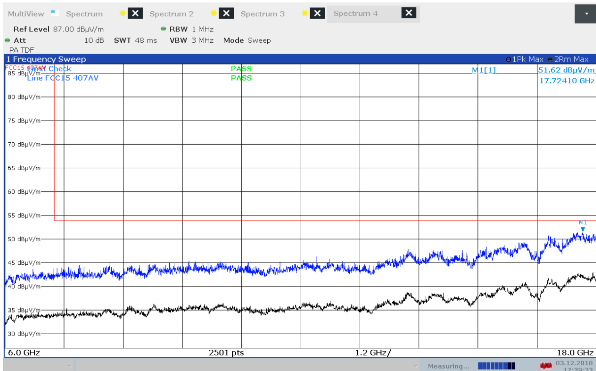
Radiated Emissions, 6000 - 18000 MHz, 5700 MHz, 802.11n MCS0, EUT V, VP
