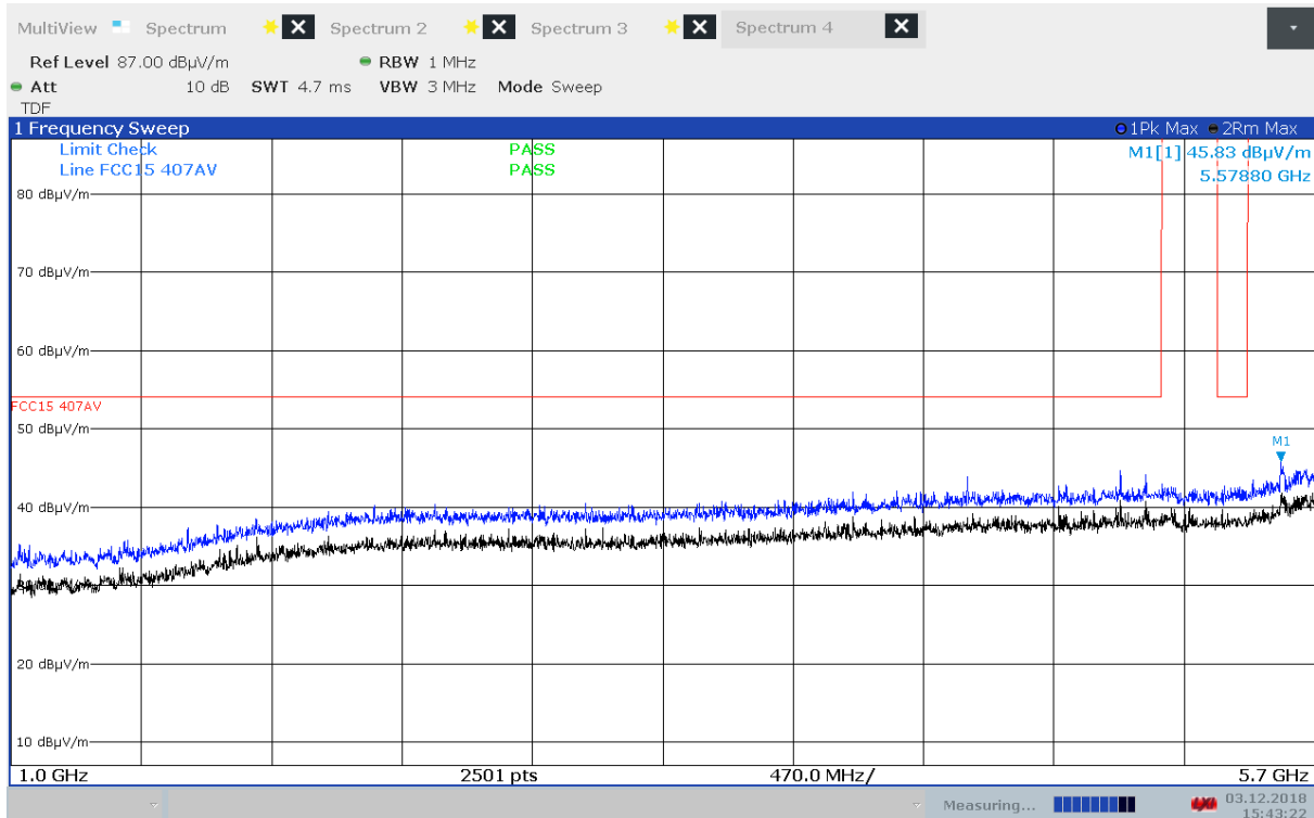
Radiated Emissions, 1000 - 5700 MHz, 5745 MHz, 802.11n MCS0, EUT V, HP
