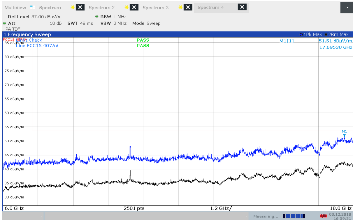
Radiated Emissions, 6000 - 18000 MHz, 5180 MHz, 802.11n MCS0, EUT V, HP
