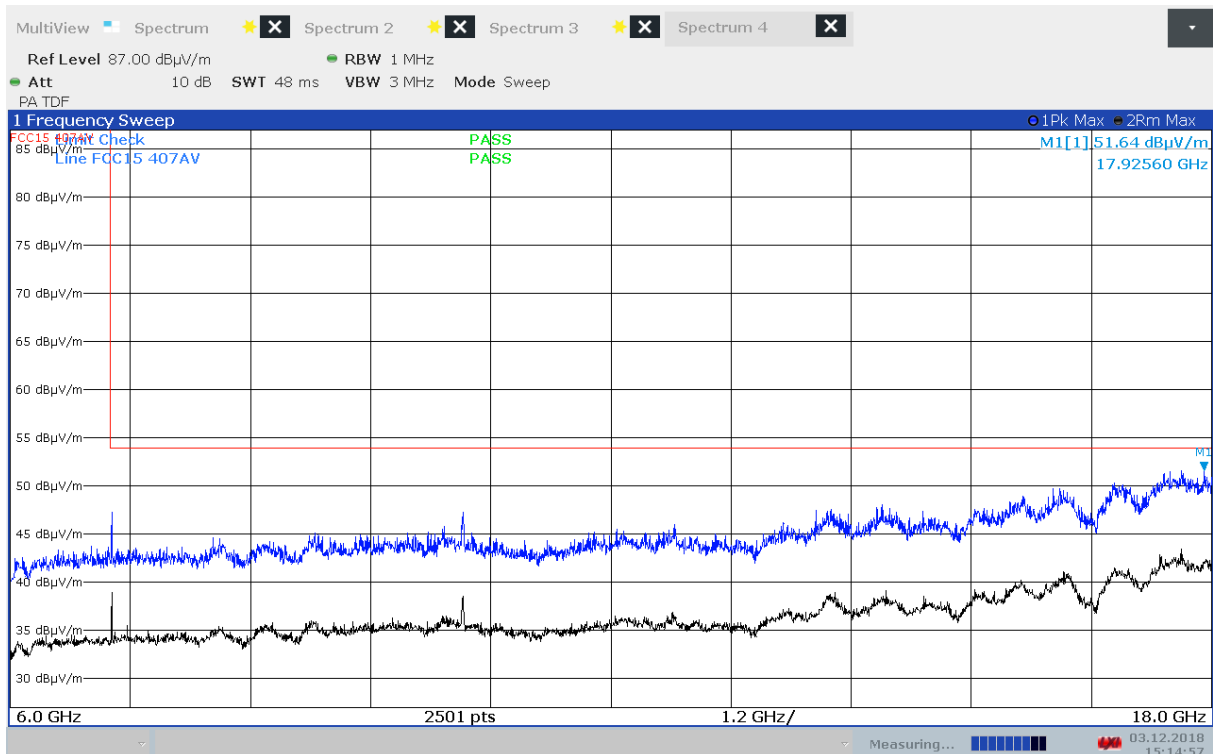
Radiated Emissions, 6000 - 18000 MHz, 5260 MHz, 802. 11a 6Mbps, EUT V, VP
