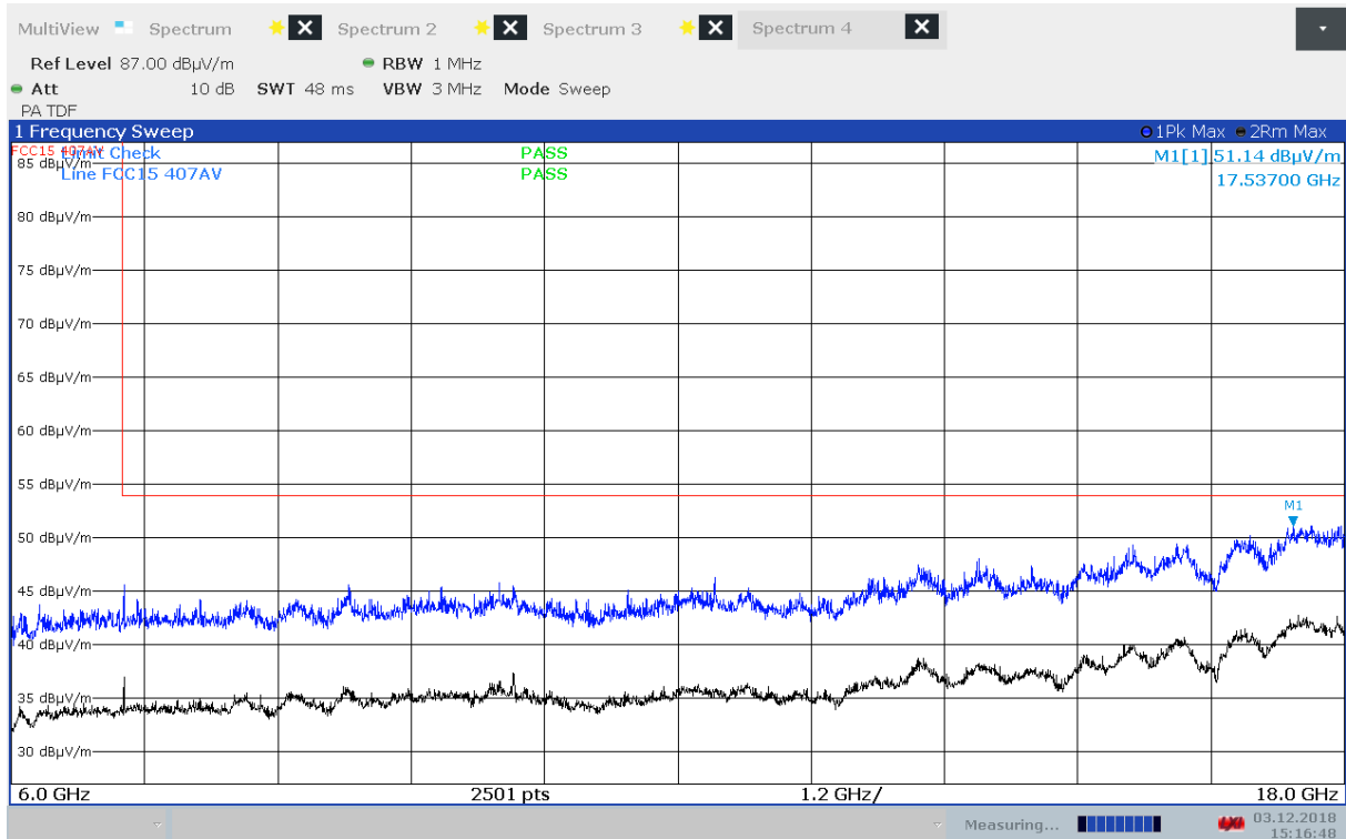
Radiated Emissions, 6000 - 18000 MHz, 5260 MHz, 802.11a 6Mbps, EUT V, HP
