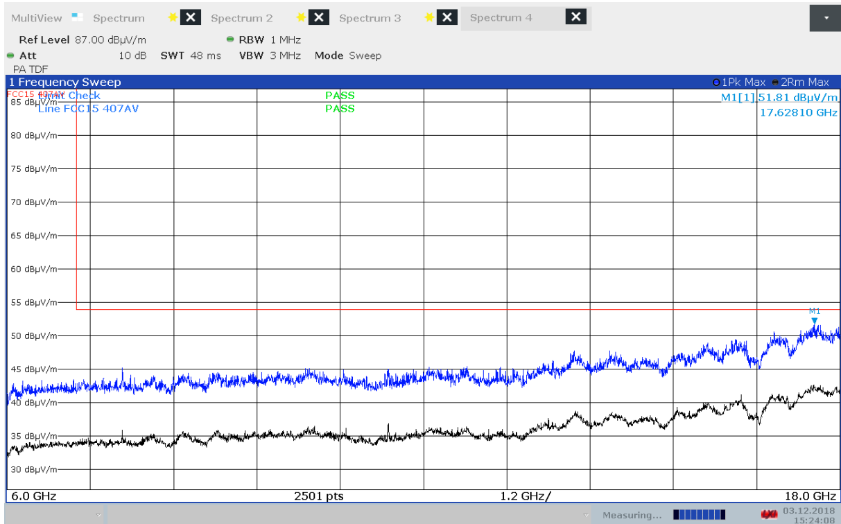
Radiated Emissions, 6000 - 18000 MHz, 5785 MHz, 802.11n MCS0, EUT V, HP
