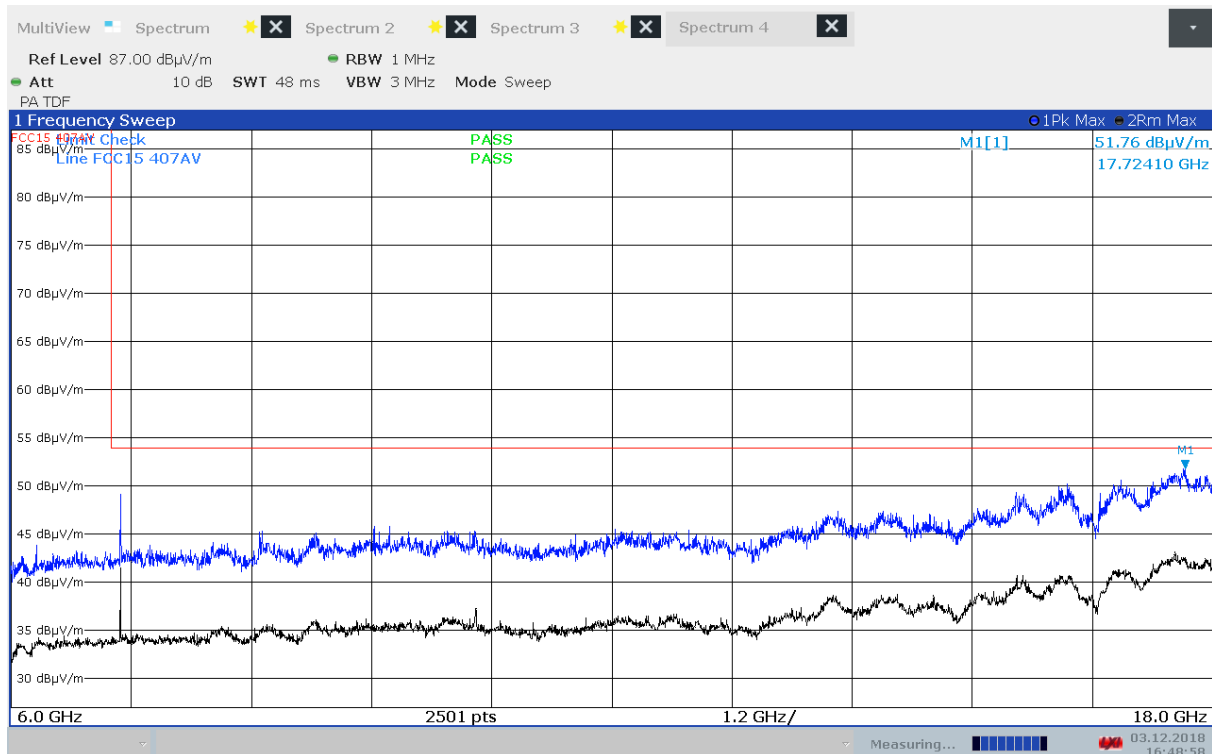
Radiated Emissions, 6000 - 18000 MHz, 5320 MHz, 802.11n MCS0, EUT V, VP
