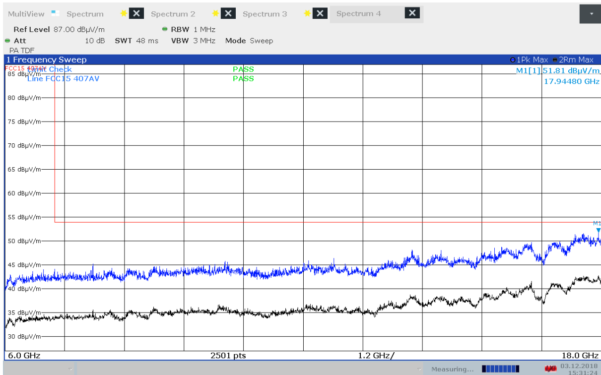
Radiated Emissions, 6000 - 18000 MHz, 5825 MHz, 802.11a 6Mbps, EUT V, VP
