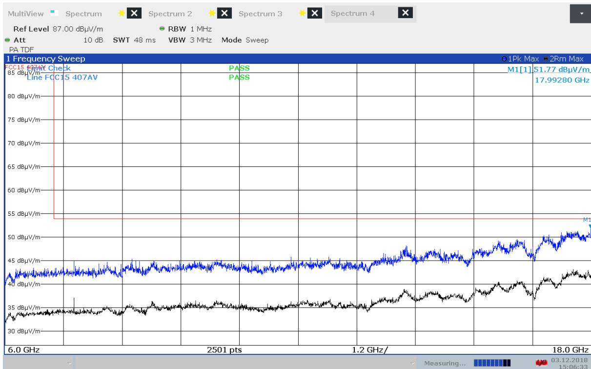
Radiated Emissions, 6000 - 18000 MHz, 5560 MHz, 802. 11a 6Mbps, EUT V, VP
