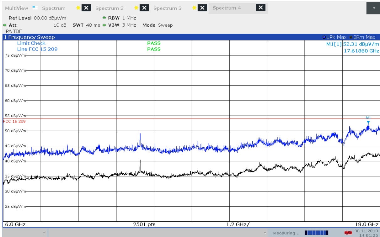
Radiated Emissions, 6000 - 18000 MHz, 5180 MHz, 802.11a 6Mbps, EUT V, HP
