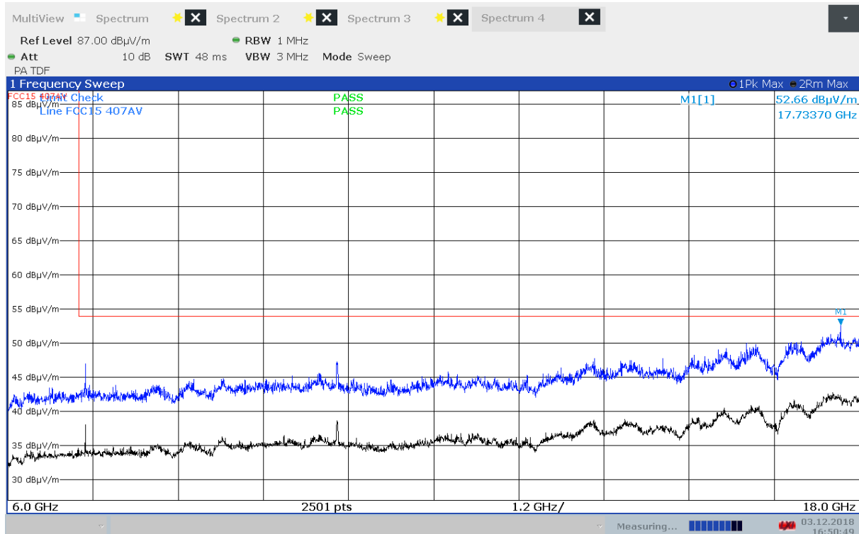
Radiated Emissions, 6000 - 18000 MHz, 5320 MHz, 802.11n MCS0, EUT V, HP
