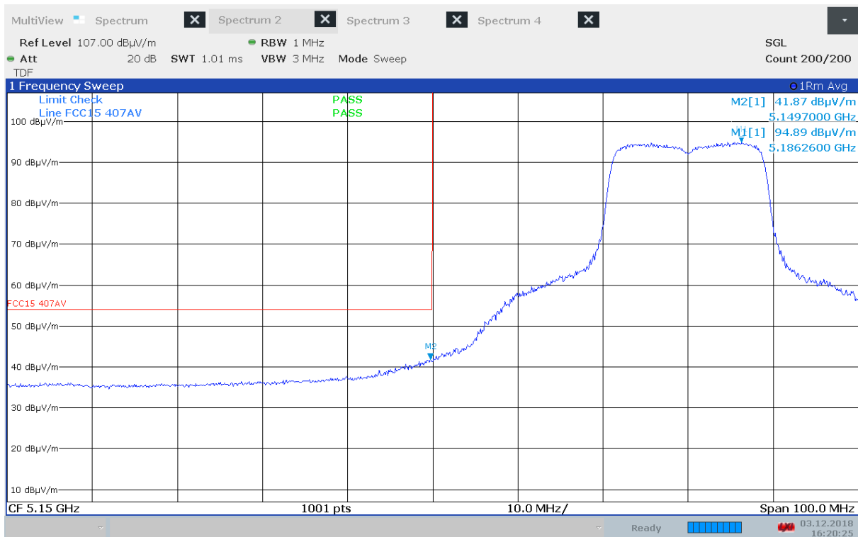
Band Edge, 5150 MHz, Ch036, 802.11n MCS0, EUT V (Max: HP), Average
