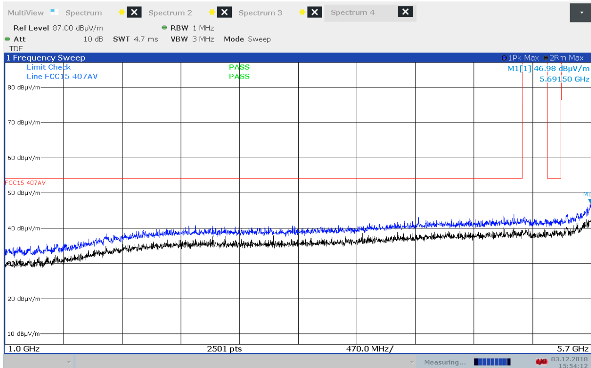
Radiated Emissions, 1000 - 5700 MHz, 5745 MHz, 802.11a 6Mbps, EUT V, HP
