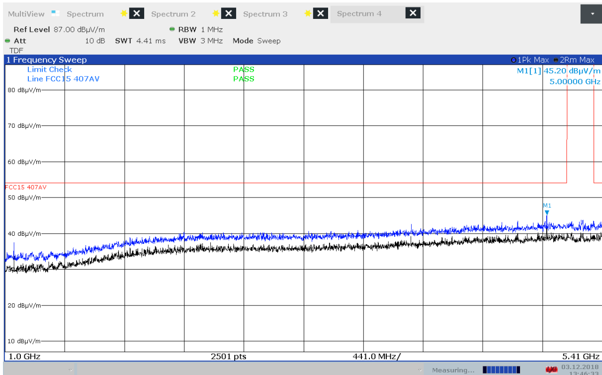
Radiated Emissions, 1000 - 5410 MHz, 5500 MHz, 802.11a 6Mbps, EUT V, VP
