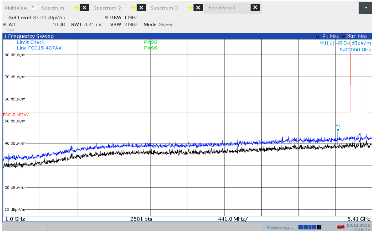
Radiated Emissions, 1000 - 5410 MHz, 5500 MHz, 802.11a 6Mbps, EUT V, HP
