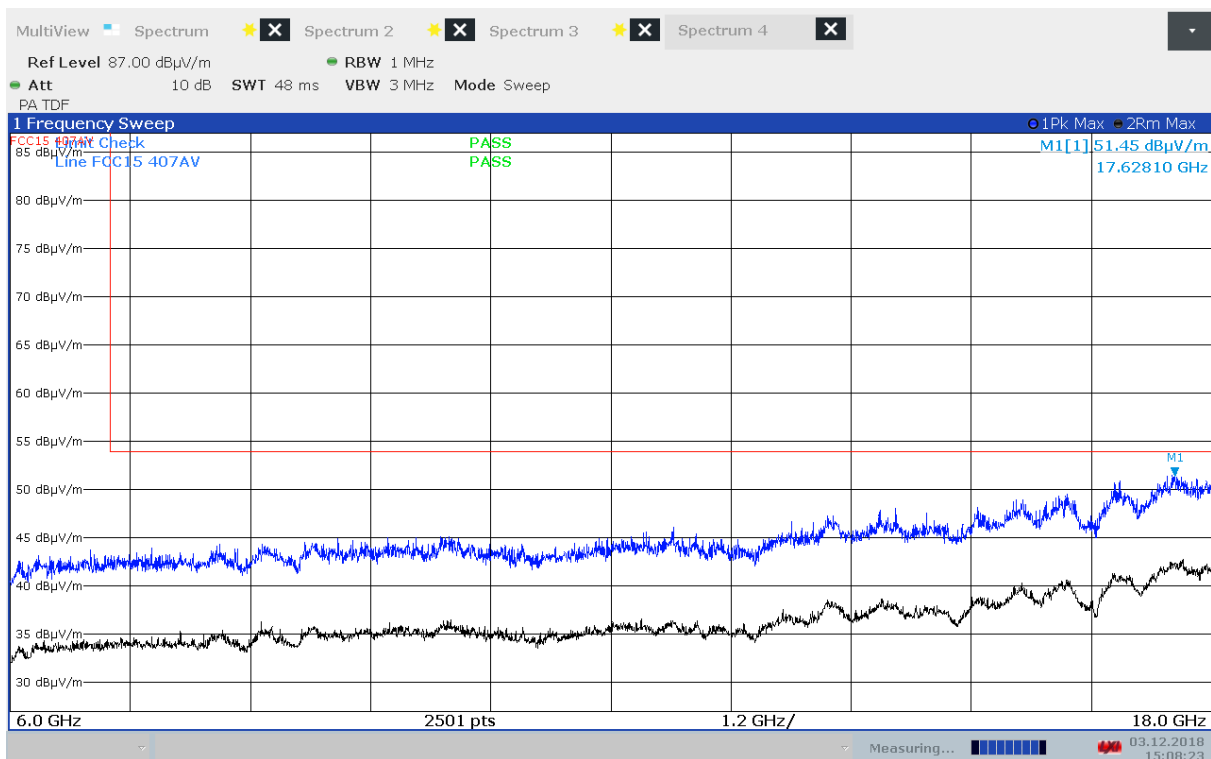
Radiated Emissions, 6000 - 18000 MHz, 5560 MHz, 802.11a 6Mbps, EUT V, HP
