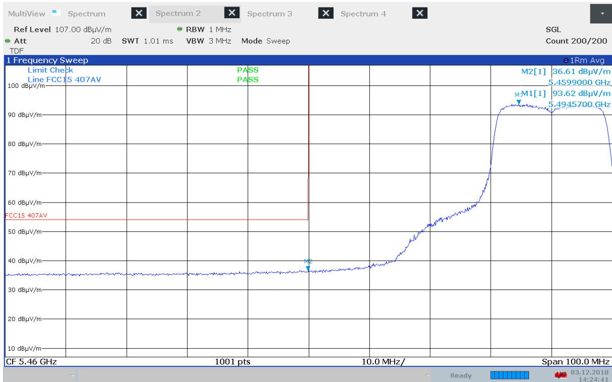
Band Edge, 5460 MHz, 5500 MHz, 802.11n MCS0, EUT V (Max: VP), Average
