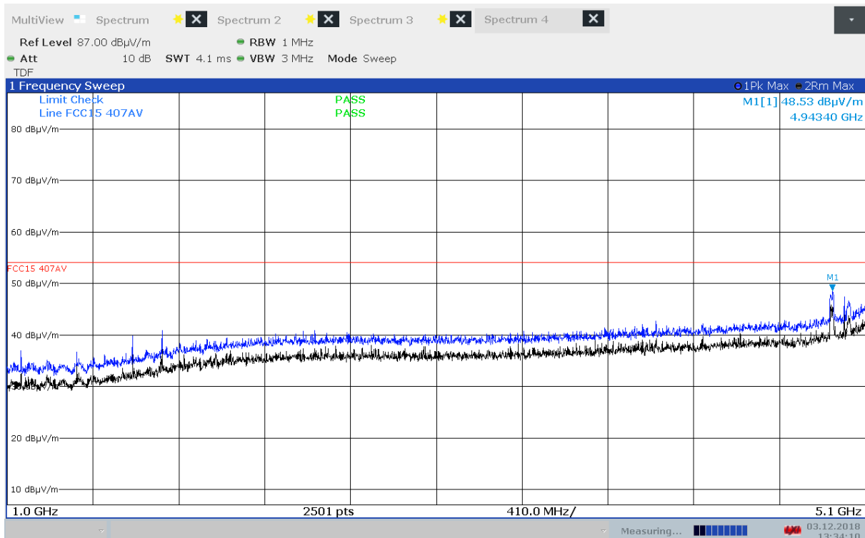
Radiated Emissions, 1000 - 5100 MHz, 5180 MHz, 802.11n MCS0, EUT V, VP
