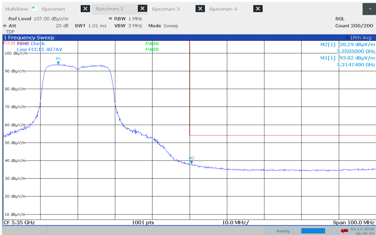
Band Edge, 5350 MHz, 5320 MHz, 802.11n MCS0, EUT V (Max: HP), Average
