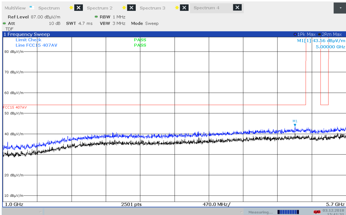
Radiated Emissions, 1000 - 5700 MHz, 5745 MHz, 802.11n MCS0, EUT V, VP
