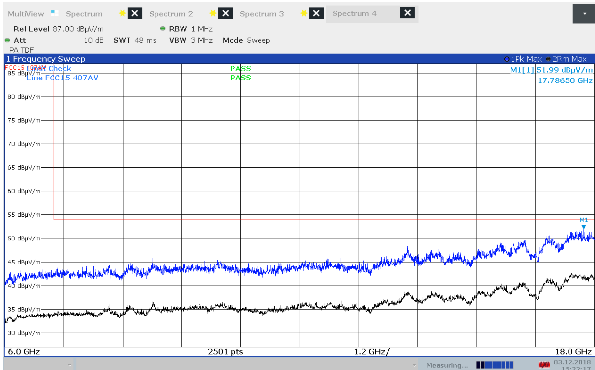
Radiated Emissions, 6000 - 18000 MHz, 5785 MHz, 802.11n MCS0, EUT V, VP
