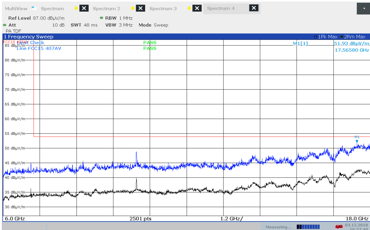
Radiated Emissions, 6000 - 18000 MHz, 5180 MHz, 802.11n MCS0, EUT V, VP
