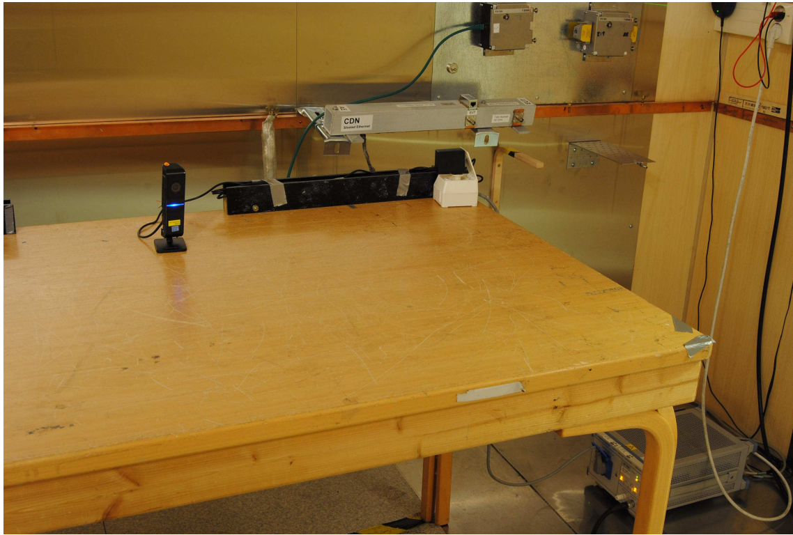
Power-Line Conducted Emissions Test
