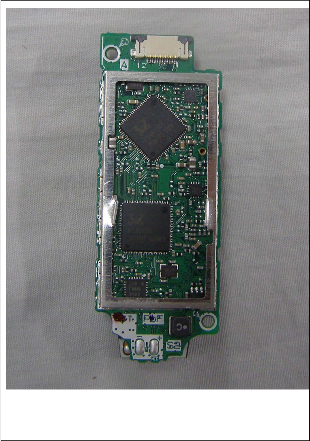
RF Board (Without Shield)
