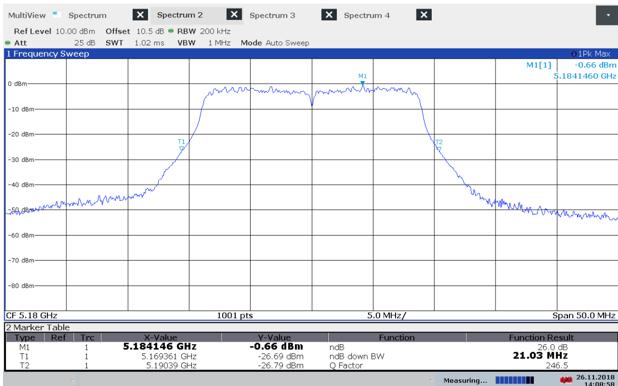
Emission Bandwidth B, 5180 MHz, 802.11n MCS0
