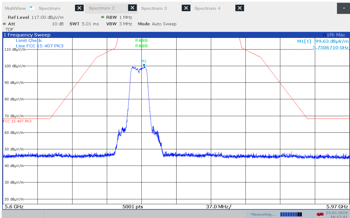
Unwanted Emissions, Band Edge, 5725 MHz, Ch149, 802.11n MCS0, Radiated
