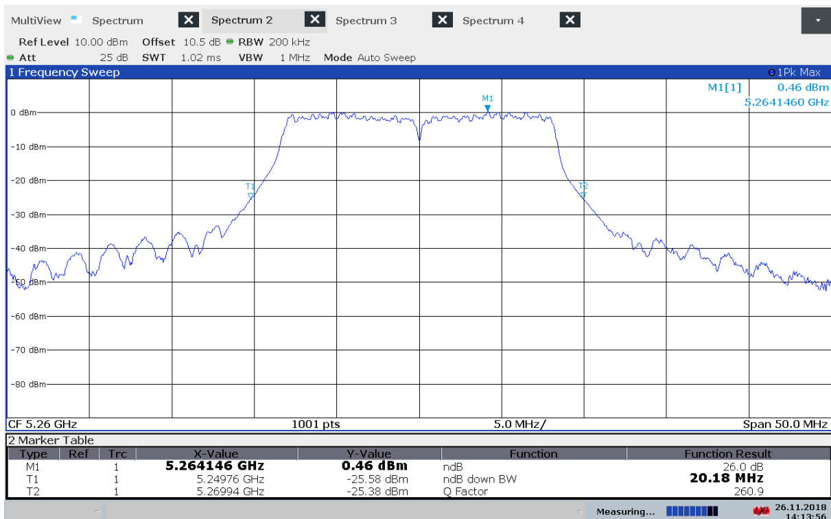
Emission Bandwidth B, 5260 MHz, 802.11n MCS0
