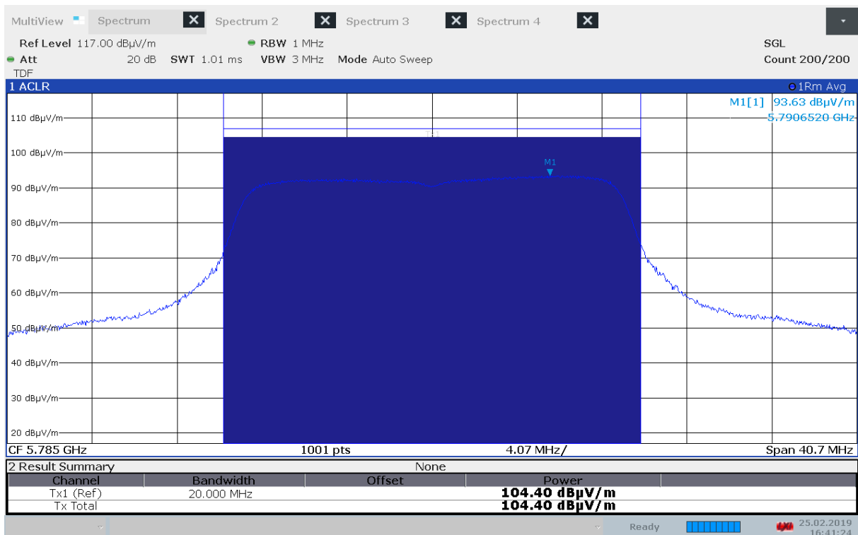
Maximum Field Strength, 5785 MHz, Method 1, 802.11n MCS0
