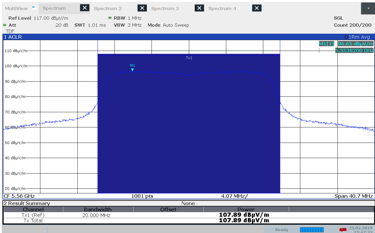
Maximum Field Strength, 5560 MHz, Method 1, 802.11n MCS0
