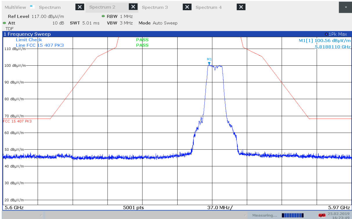
Unwanted Emissions, Band Edge, 5825 MHz, Ch165, 802.11a 6Mbps, Radiated
