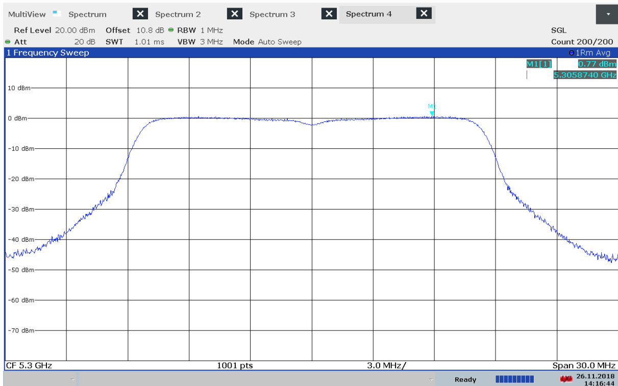
Power Spectral Density, 5300 MHz, 802.11n - MCS0, Method 2
