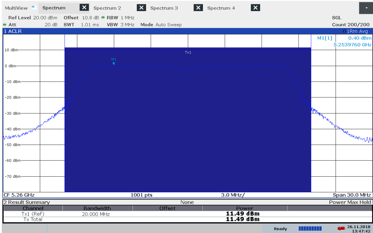
Output Power, 5260 MHz, Method 1, 802.11a 6Mbps, Conducted
