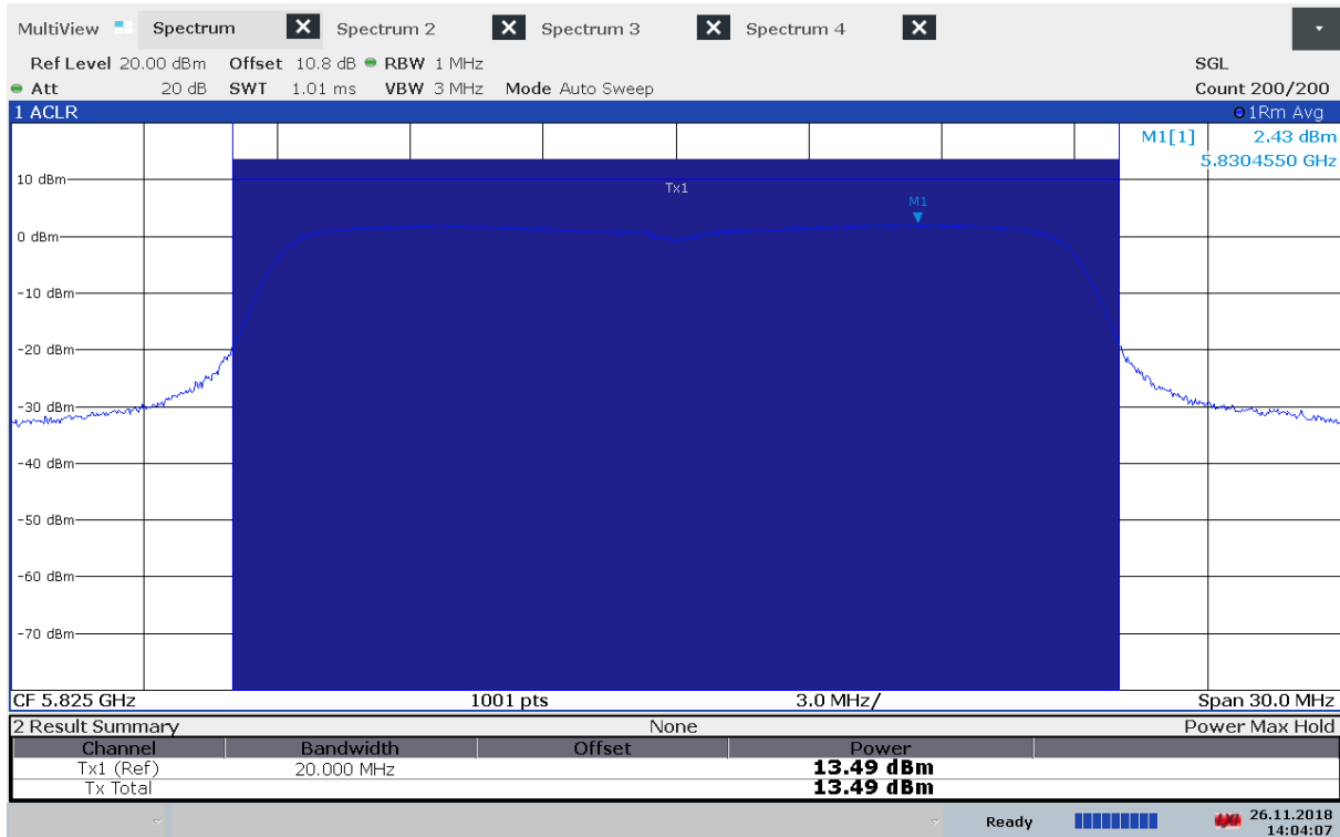
Output Power, 5825 MHz, Method 1, 802.11a 6Mbps, Conducted
