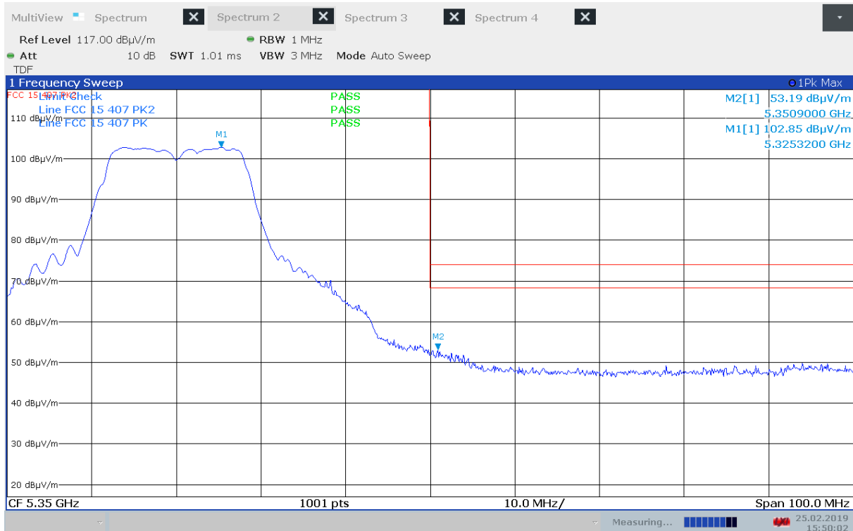
Unwanted Emissions, Band Edge, 5350 MHz, Ch064, 802.11a 6Mbps, Radiated
