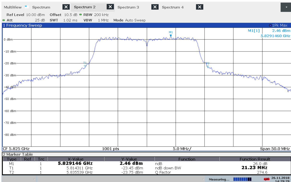
Emission Bandwidth B, 5825 MHz, 802.11n MCS0
