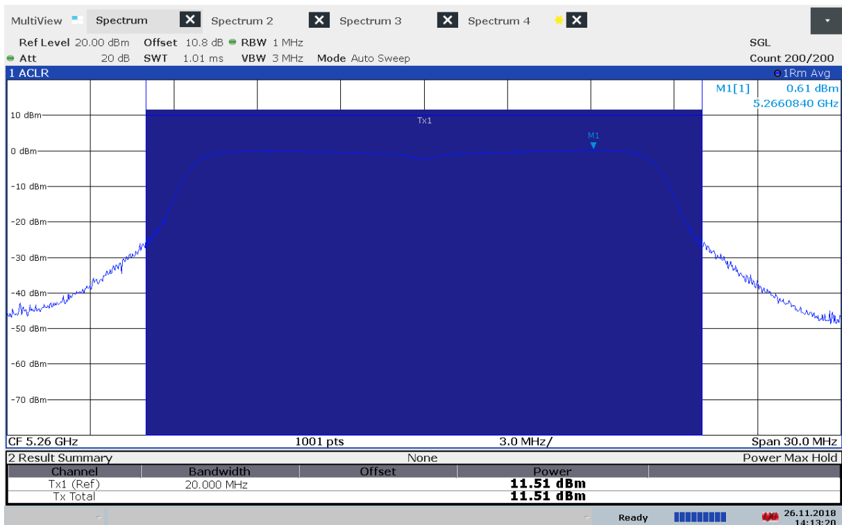
Output Power, 5260 MHz, Method 1, 802.11n MCS0, Conducted
