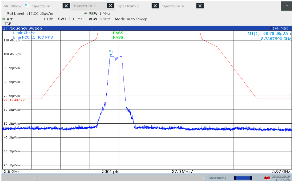
Unwanted Emissions, Band Edge, 5725 MHz, Ch149, 802.11a 6Mbps, Radiated
