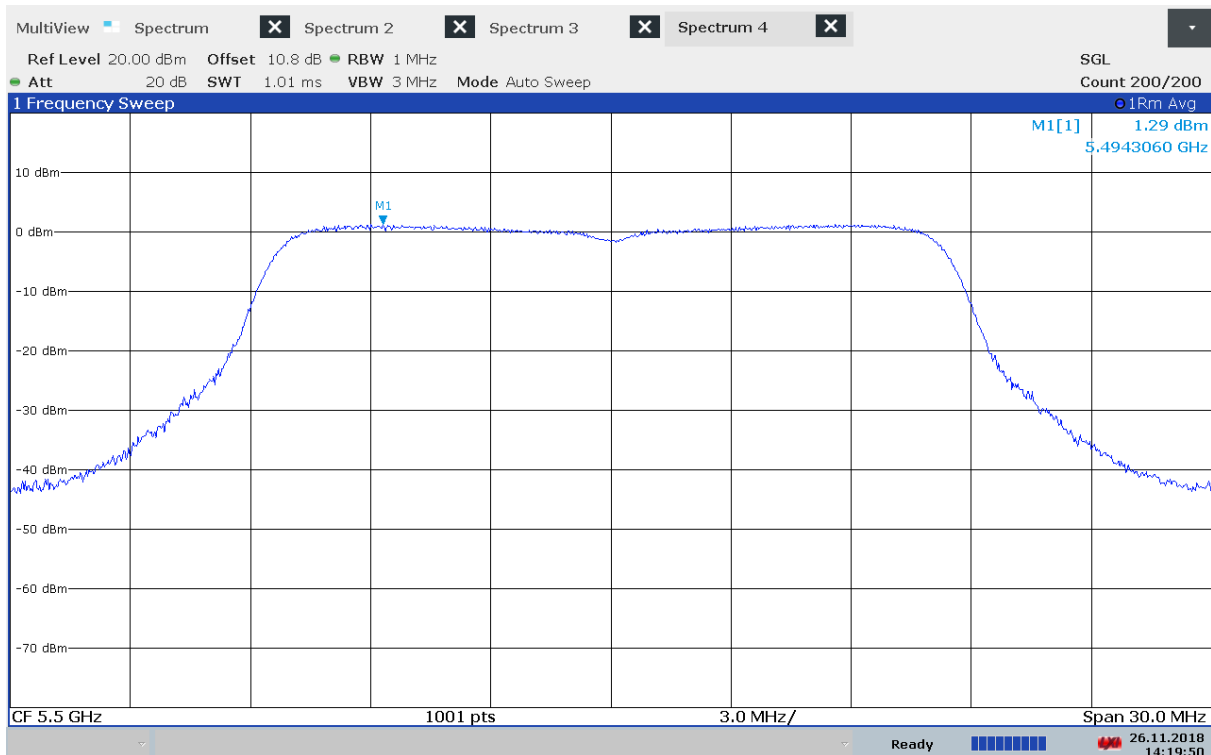
Power Spectral Density, 5500 MHz, 802.11n - MCS0, Method 2
