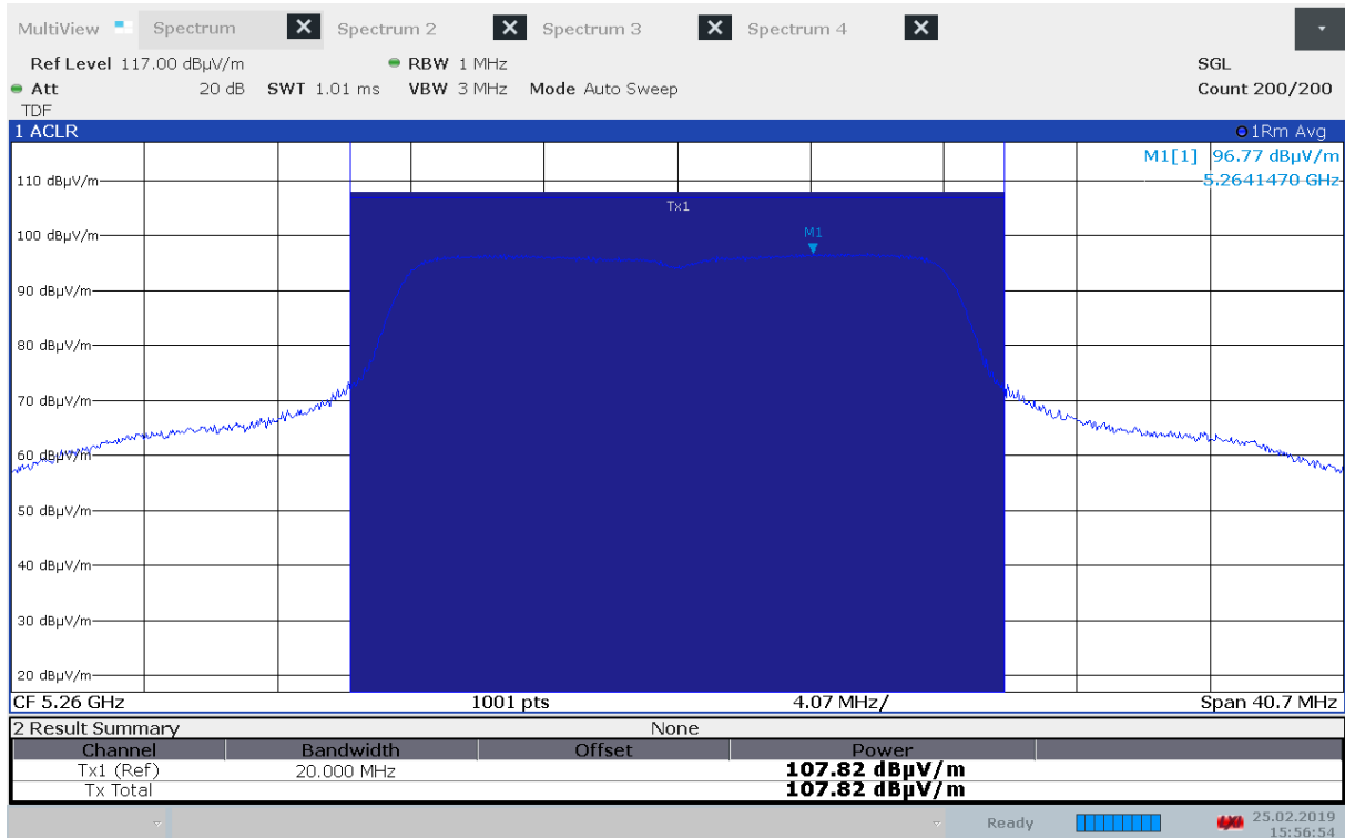
Maximum Field Strength, 5260 MHz, Method 1, 802.11a 6Mbps
