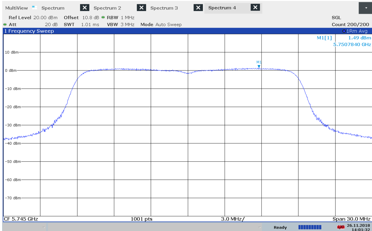
Power Spectral Density, 5745 MHz, 802.11a - 6Mbps, Method 2
