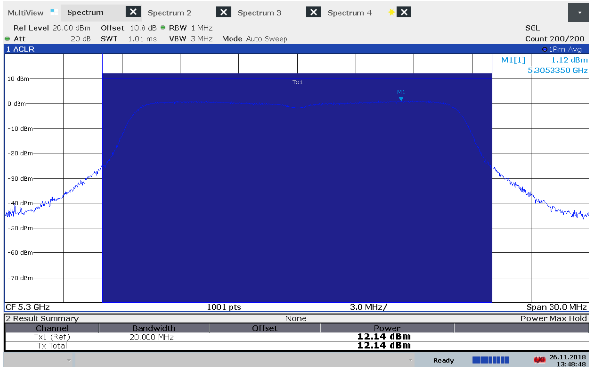
Output Power, 5300 MHz, Method 1, 802.11a 6Mbps, Conducted
