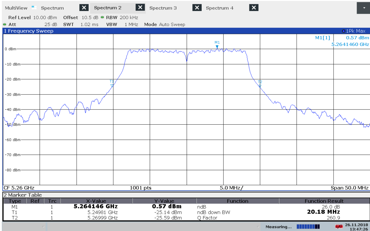
Emission Bandwidth B, 5260 MHz, 802.11a 6Mbps
