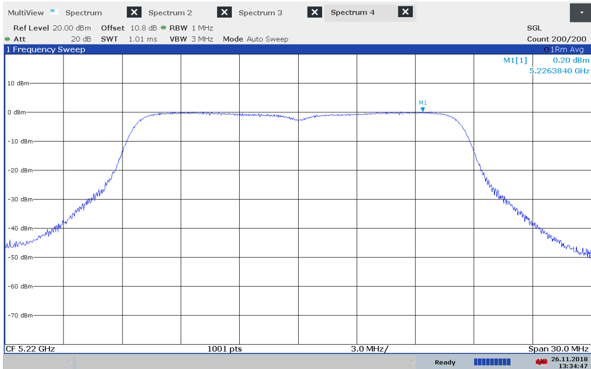
Power Spectral Density, 5220 MHz, 802.11a - 6Mbps, Method 2
