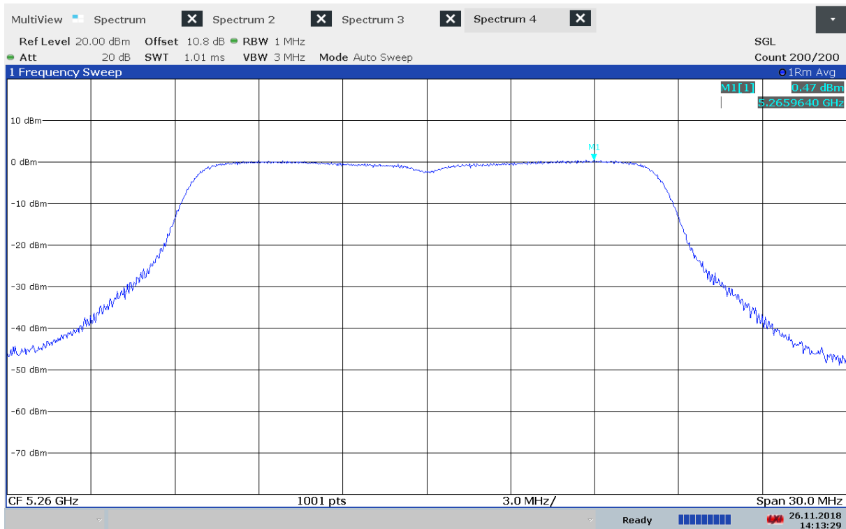
Power Spectral Density, 5260 MHz, 802.11n – MCS0, Method 2
