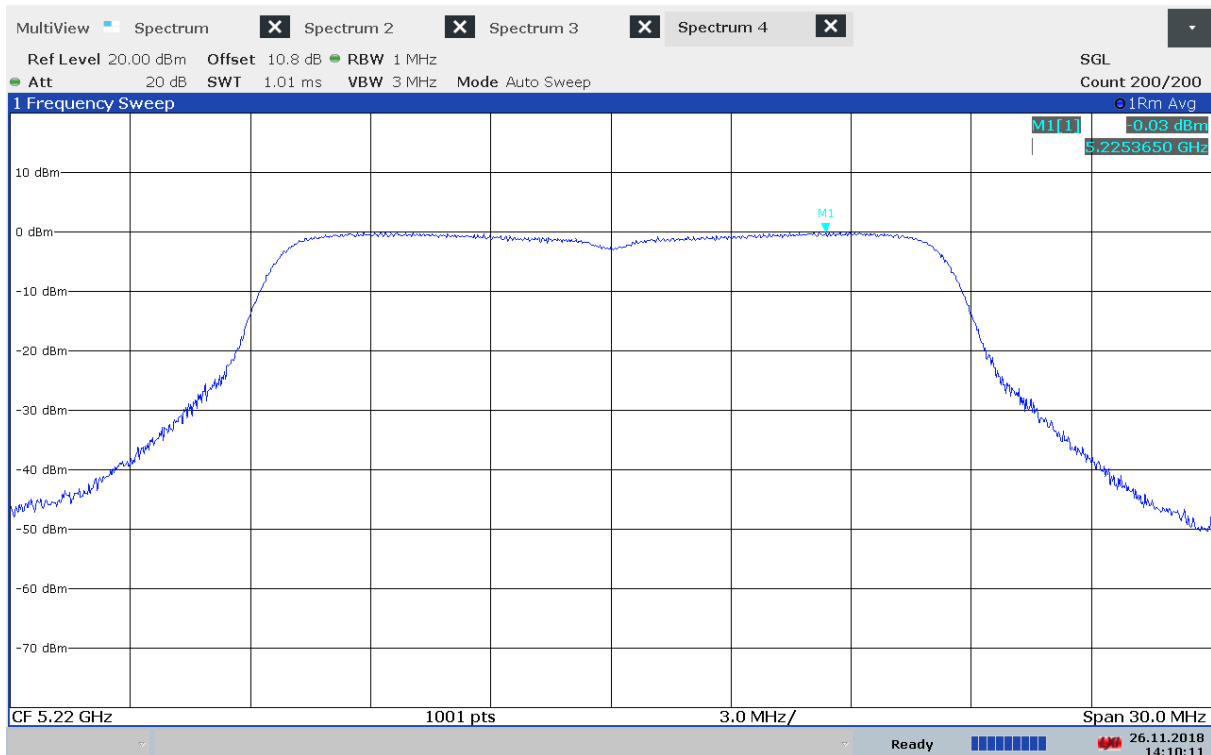
Power Spectral Density, 5220 MHz, 802.11n - MCS0, Method 2
