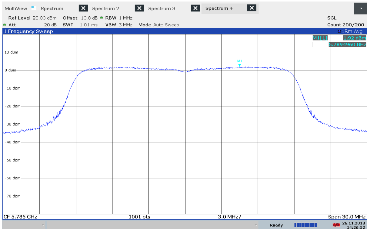
Power Spectral Density, 5785 MHz, 802.11n – MCS0, Method 2
