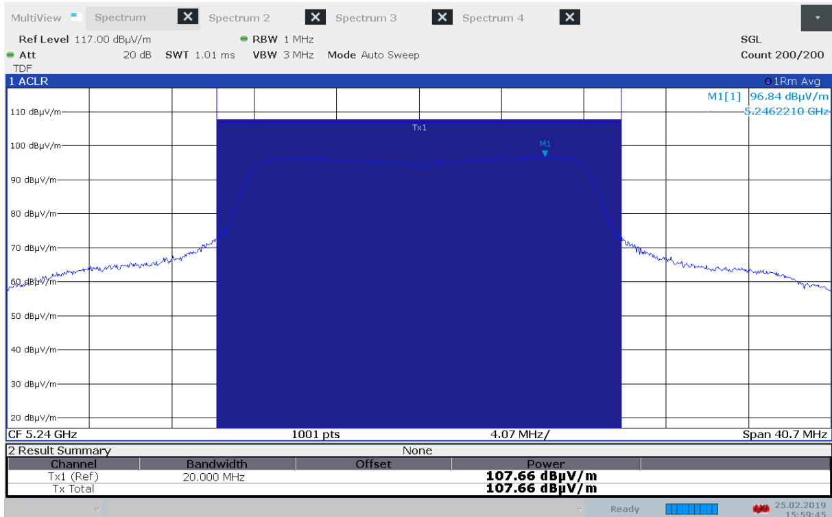
Maximum Field Strength, 5240 MHz, Method 1, 802.11a 6Mbps
