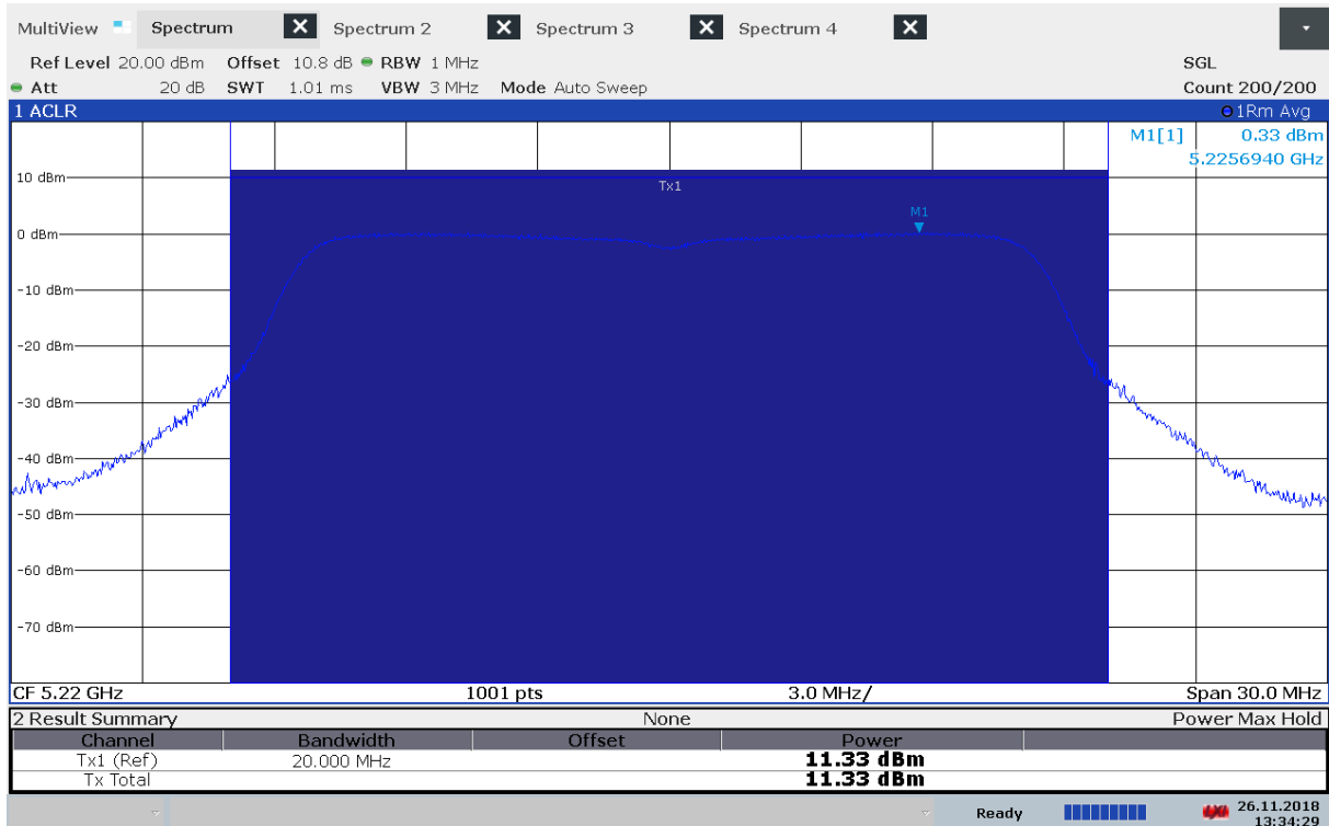
Output Power, 5220 MHz, Method 1, 802.11a 6Mbps, Conducted
