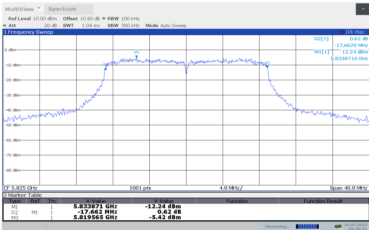
6 dB Bandwidth, 5825 MHz, 802.11n MCS0
