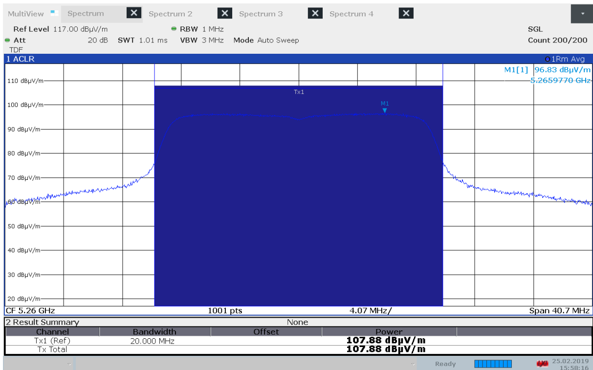
Maximum Field Strength, 5260 MHz, Method 1, 802.11n MCS0
