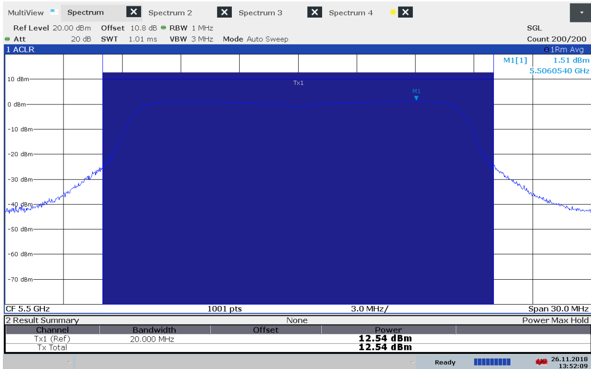
Output Power, 5500 MHz, Method 1, 802.11a 6Mbps, Conducted
