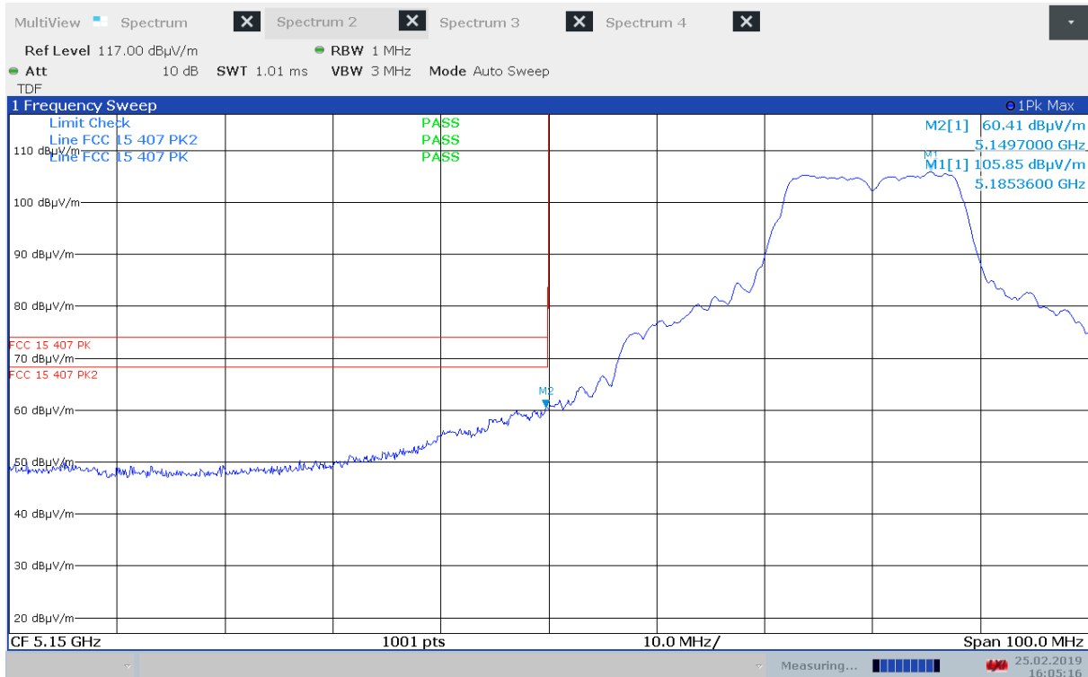
Unwanted Emissions, Band Edge, 5150 MHz, Ch036, 802.11a 6Mbps, Radiated
