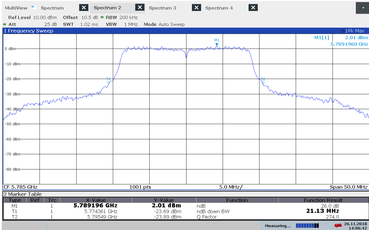
Emission Bandwidth B, 5785 MHz, 802.11a 6Mbps
