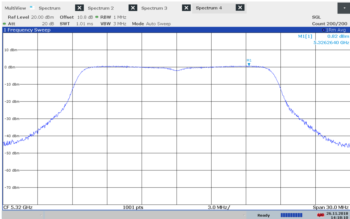
Power Spectral Density, 5320 MHz, 802.11n – MCS0, Method 2
