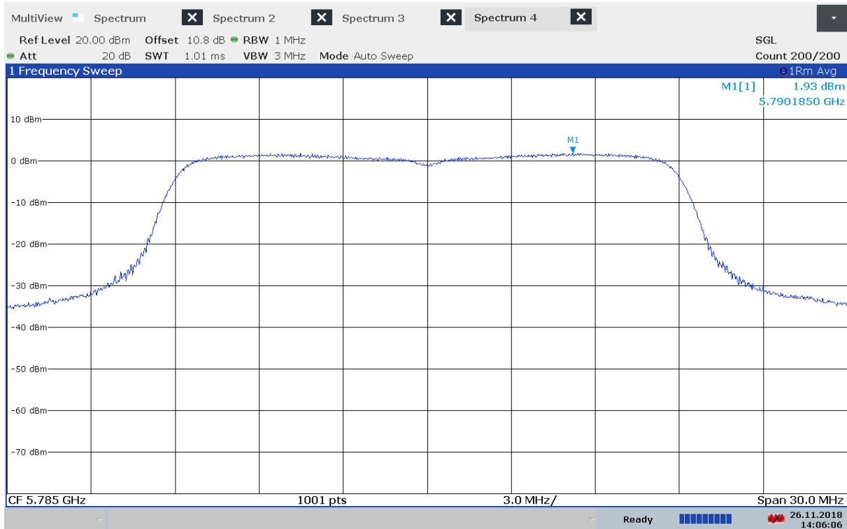
Power Spectral Density, 5785 MHz, 802.11a - 6Mbps, Method 2
