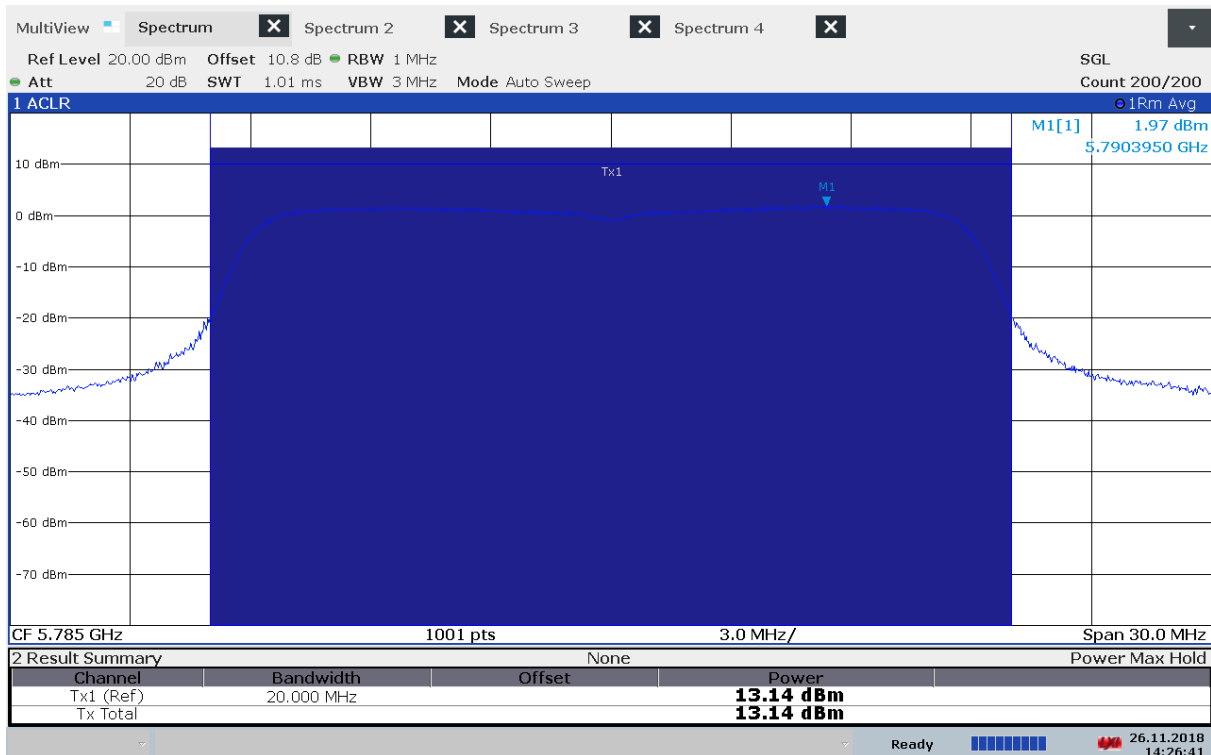
Output Power, 5785 MHz, Method 1, 802.11n MCS0, Conducted
