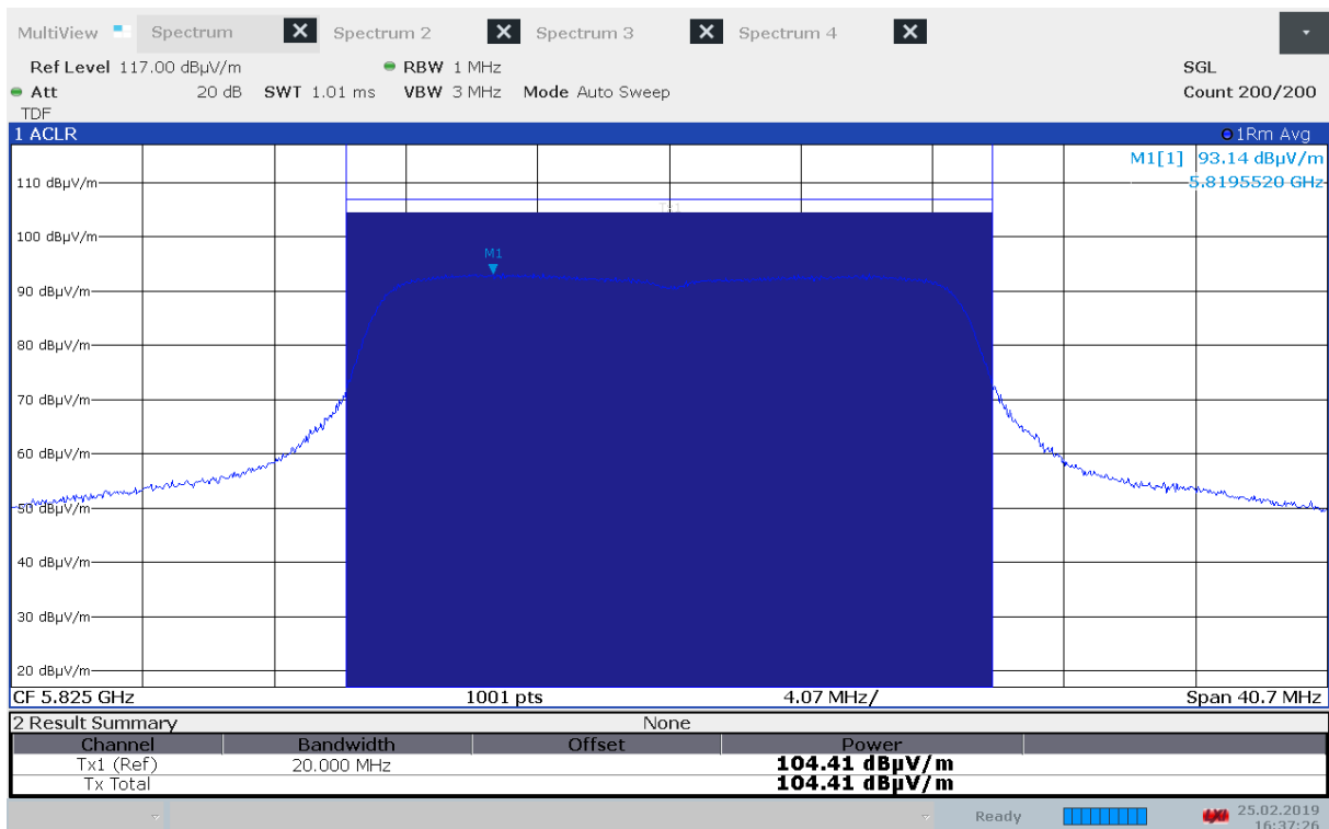
Maximum Field Strength, 5825 MHz, Method 1, 802.11n MCS0
