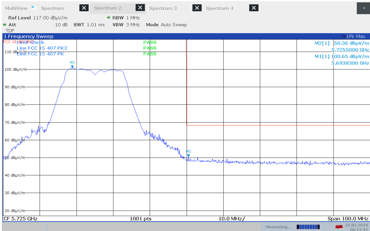
Unwanted Emissions, Band Edge, 5725 MHz, Ch140, 802.11a 6Mbps, Radiated
