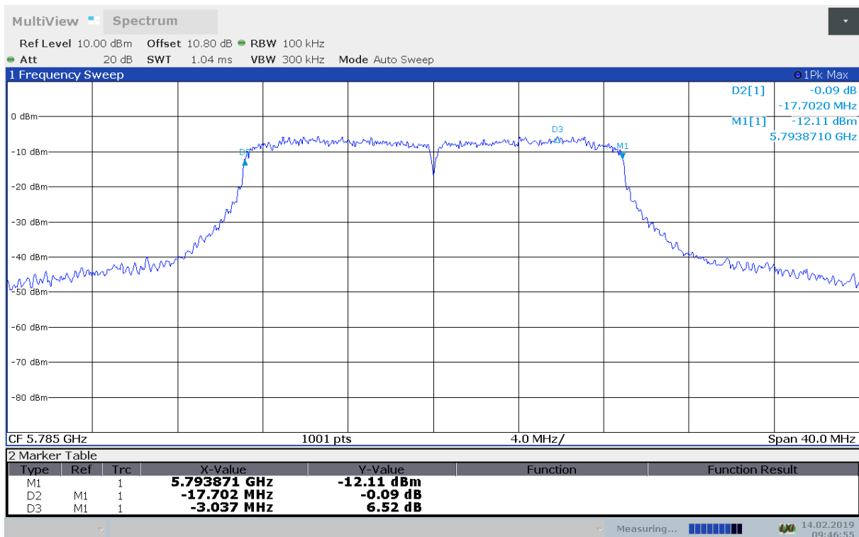
6 dB Bandwidth, 5785 MHz, 802.11n MCS0
