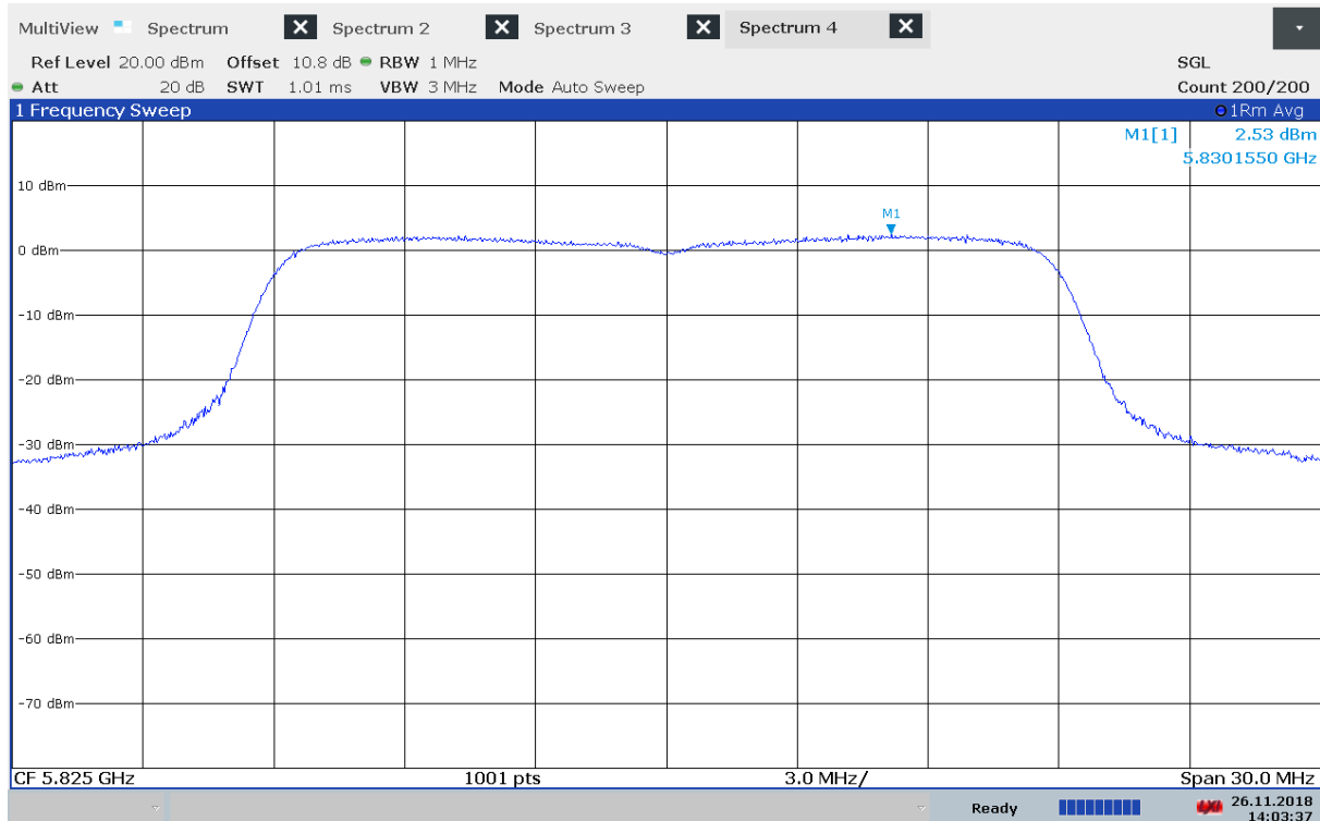
Power Spectral Density, 5825 MHz, 802.11a - 6Mbps, Method 2
