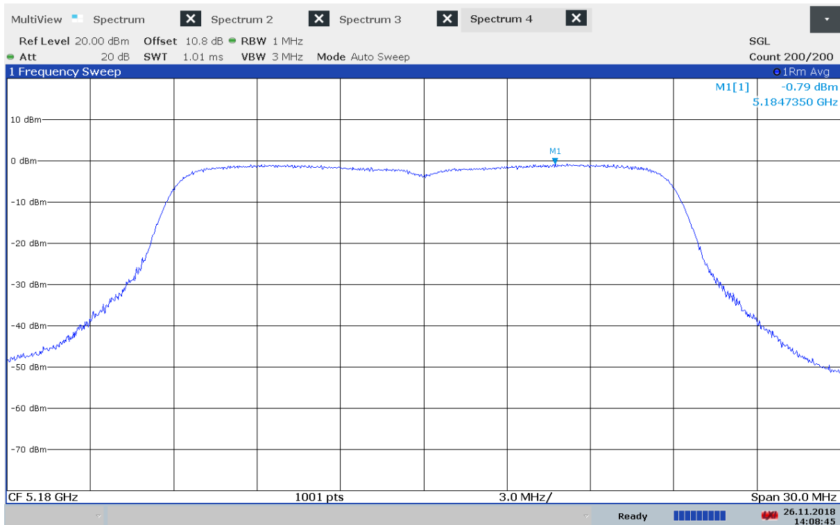
Power Spectral Density, 5180 MHz, 802.11n – MCS0, Method 2
