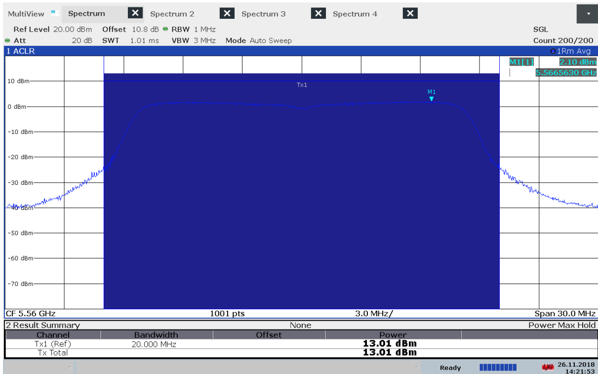
Output Power, 5560 MHz, Method 1, 802.11n MCS0, Conducted
