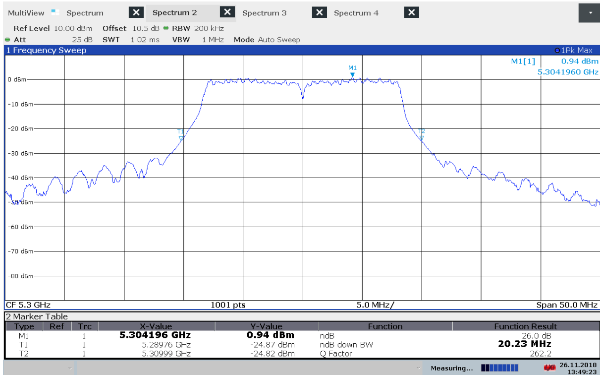
Emission Bandwidth B, 5300 MHz, 802.11a 6Mbps
