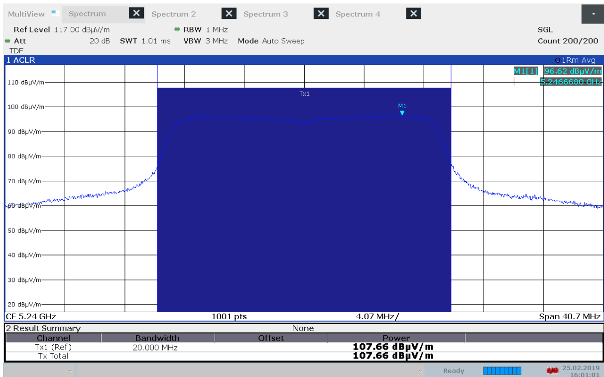
Maximum Field Strength, 5240 MHz, Method 1, 802.11n MCS0
