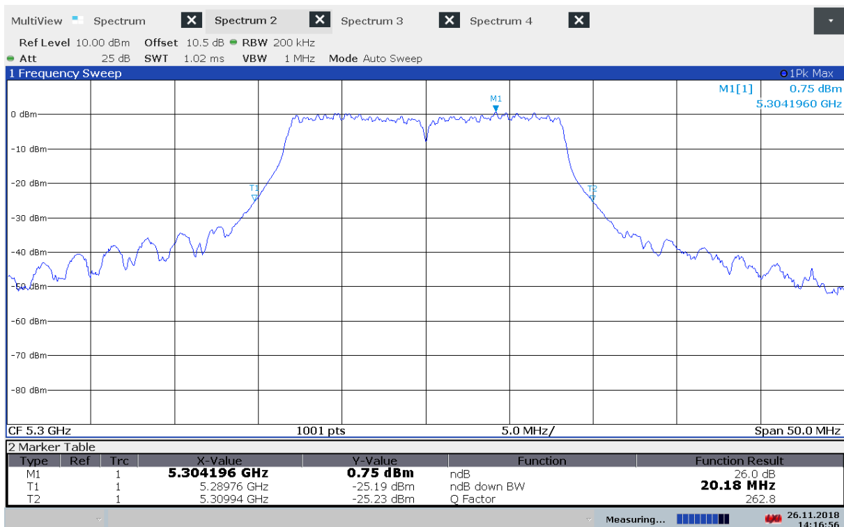
Emission Bandwidth B, 5300 MHz, 802.11n MCS0
