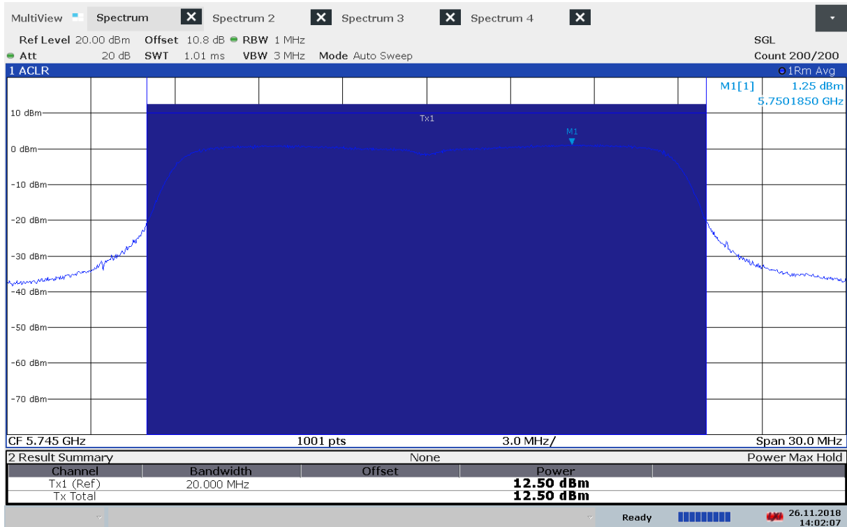
Output Power, 5745 MHz, Method 1, 802.11a 6Mbps, Conducted
