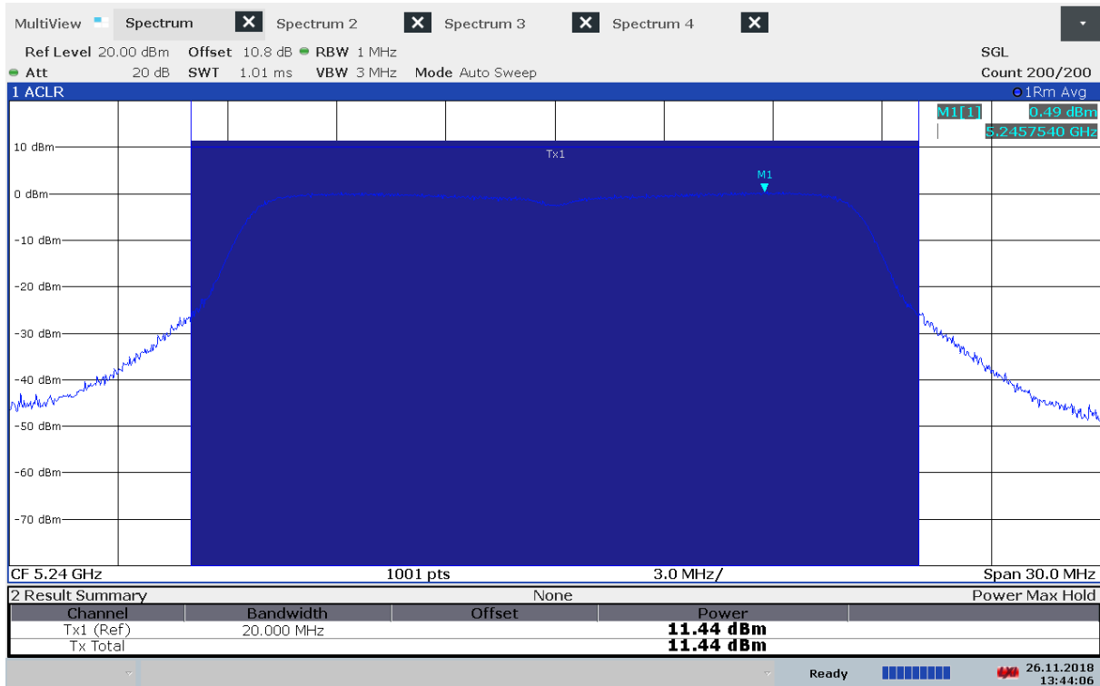
Output Power, 5240 MHz, Method 1, 802.11a 6Mbps, Conducted
