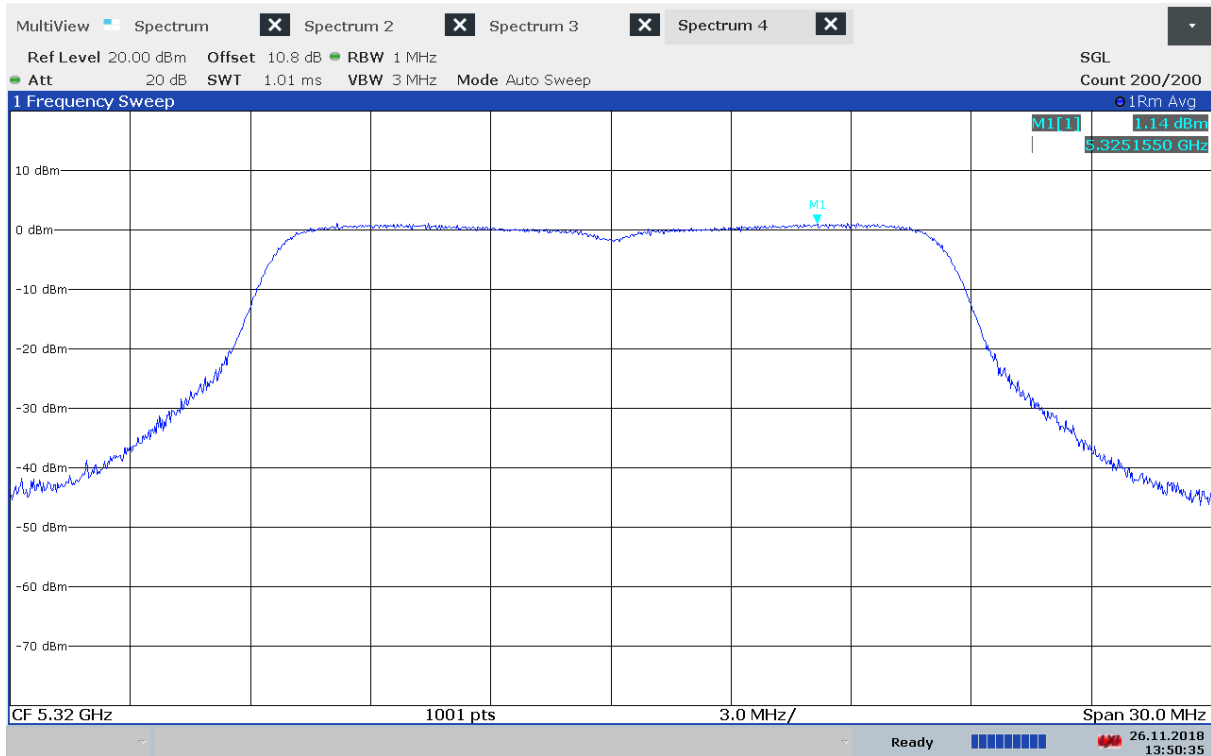
Power Spectral Density, 5320 MHz, 802.11a - 6Mbps, Method 2
