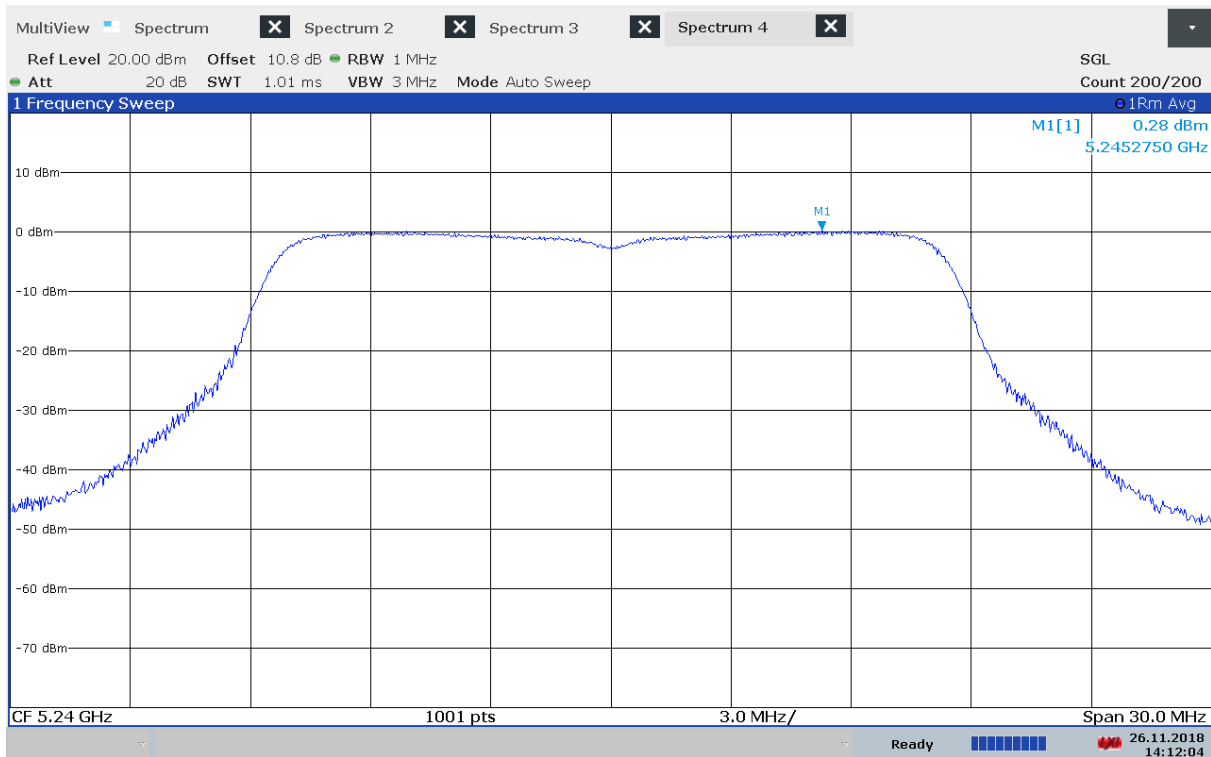
Power Spectral Density, 5240 MHz, 802.11n - MCS0, Method 2
