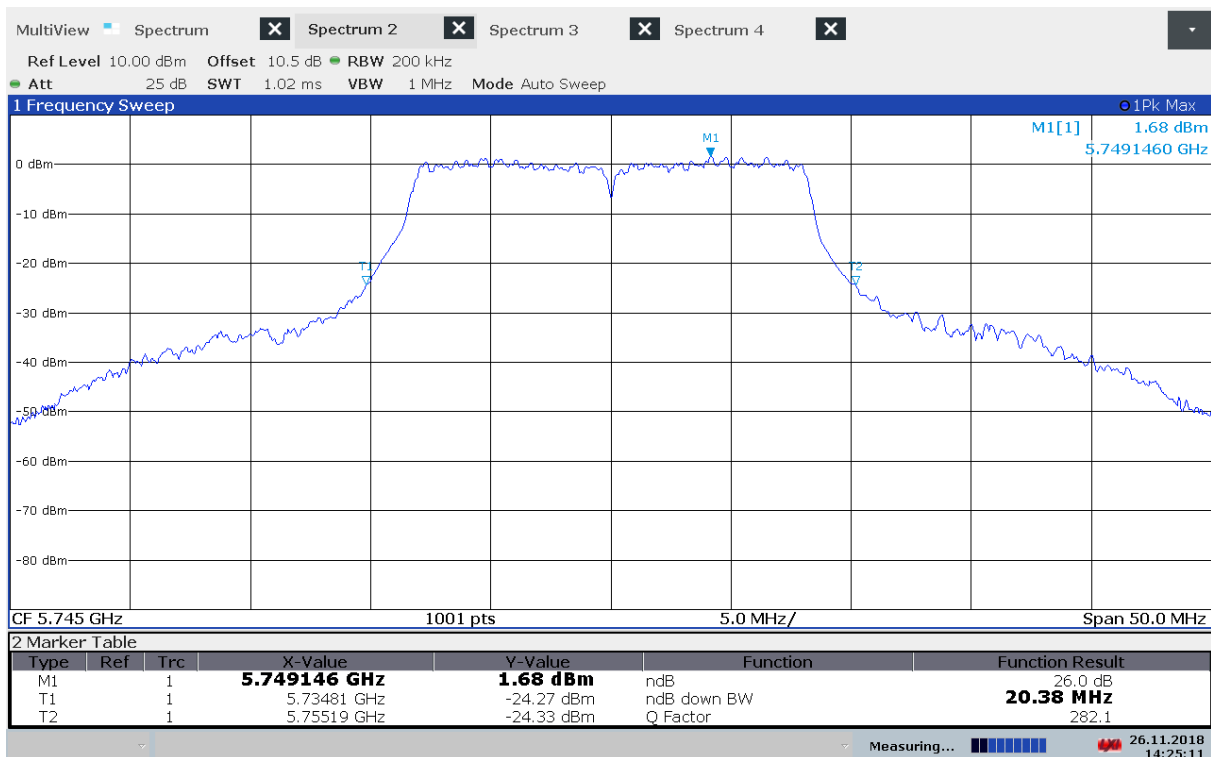
Emission Bandwidth B, 5745 MHz, 802.11n MCS0
