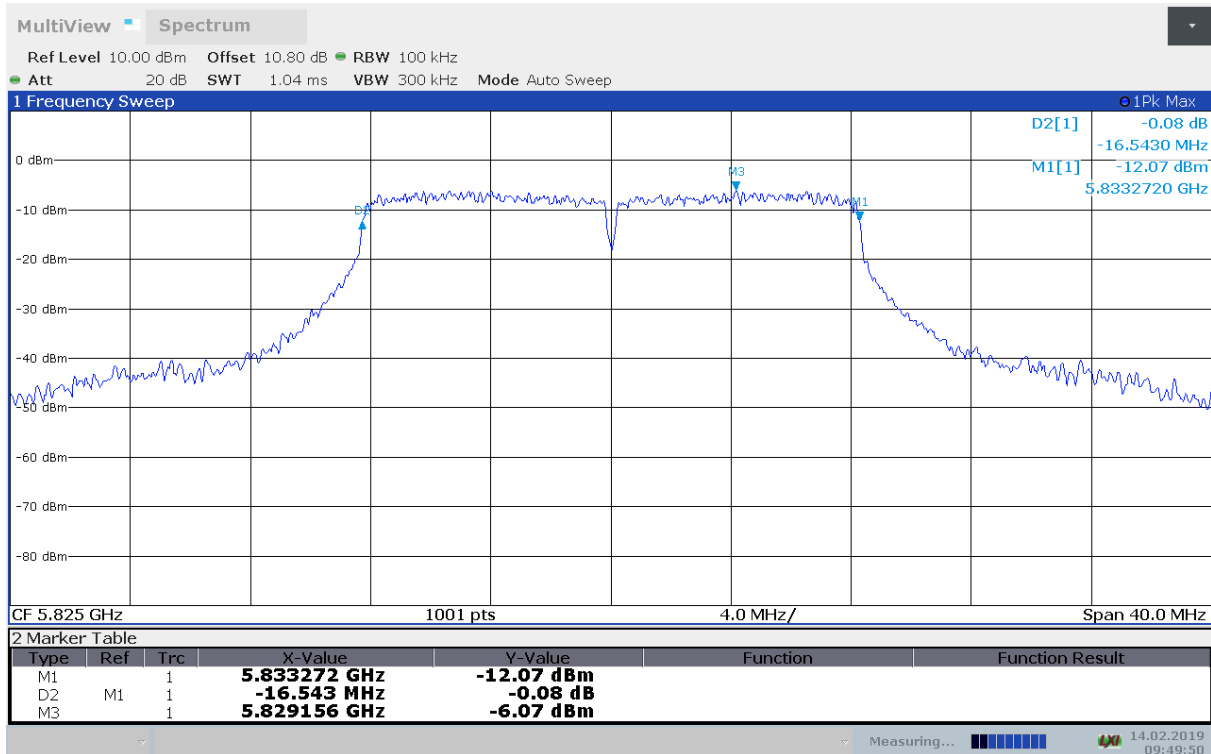
6 dB Bandwidth, 5825 MHz, 802.11a 6Mbps
