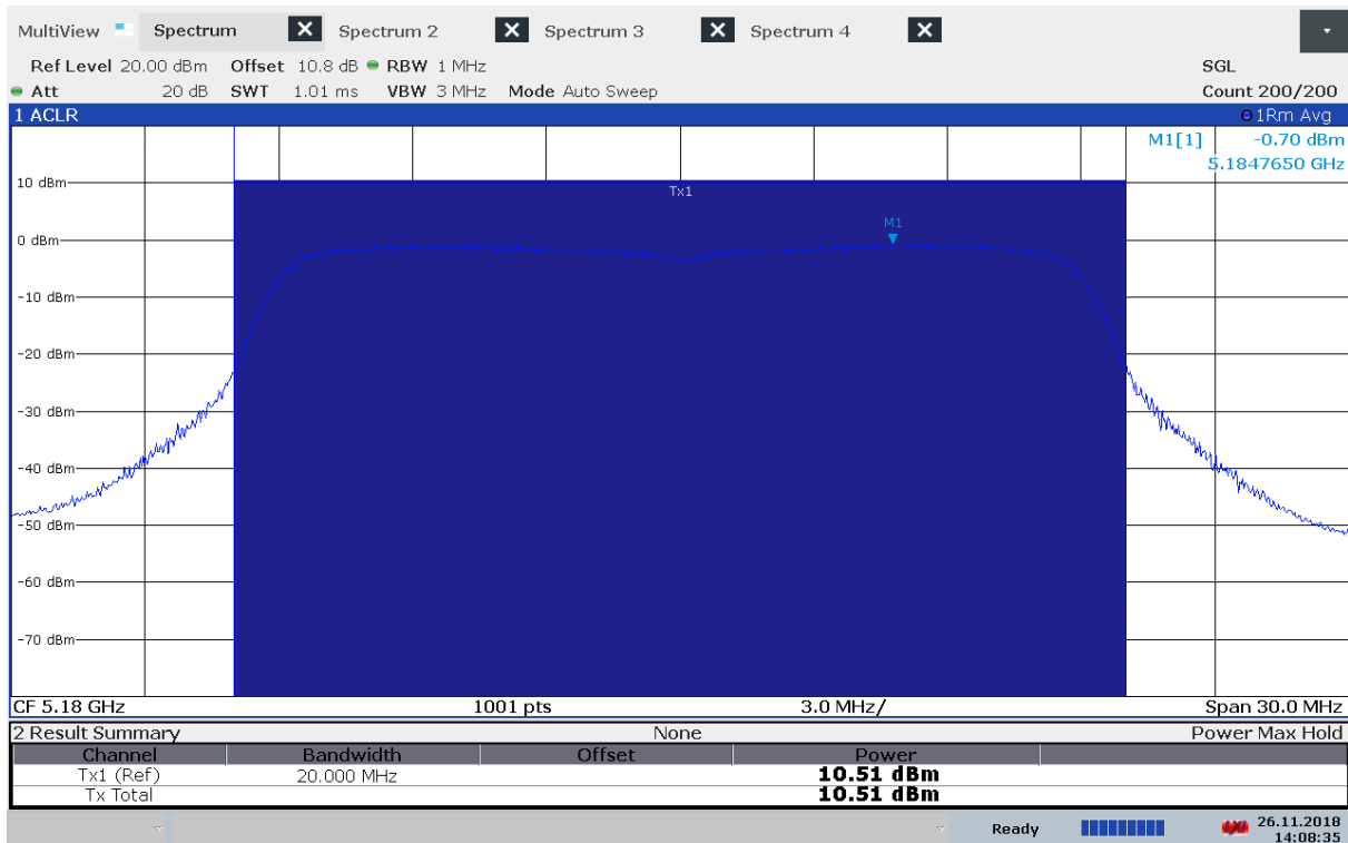
Output Power, 5180 MHz, Method 1, 802.11n MCS0, Conducted
