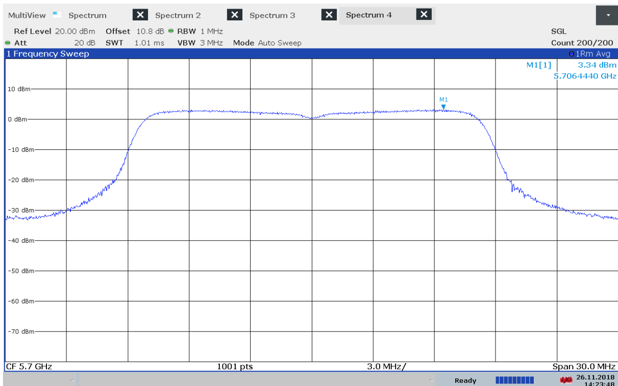
Power Spectral Density, 5700 MHz, 802.11n - MCS0, Method 2
