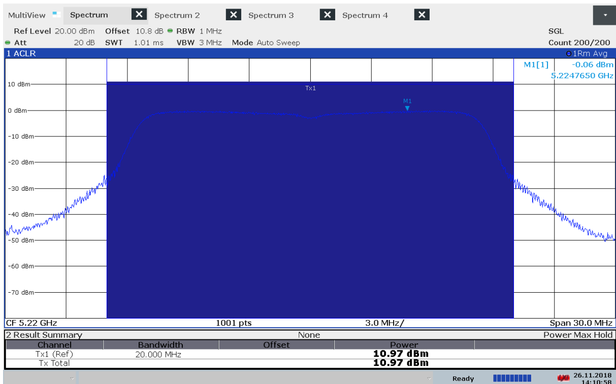
Output Power, 5220 MHz, Method 1, 802.11n MCS0, Conducted
