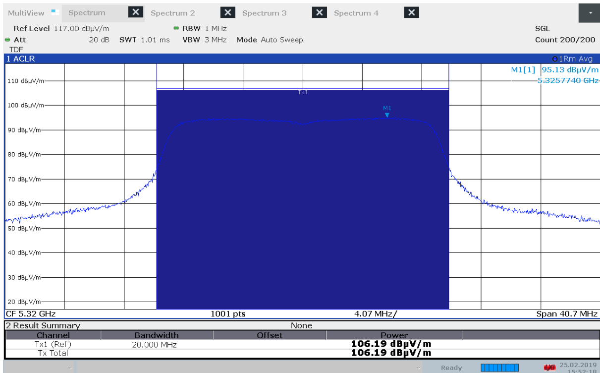
Maximum Field Strength, 5320 MHz, Method 1, 802.11n MCS0
