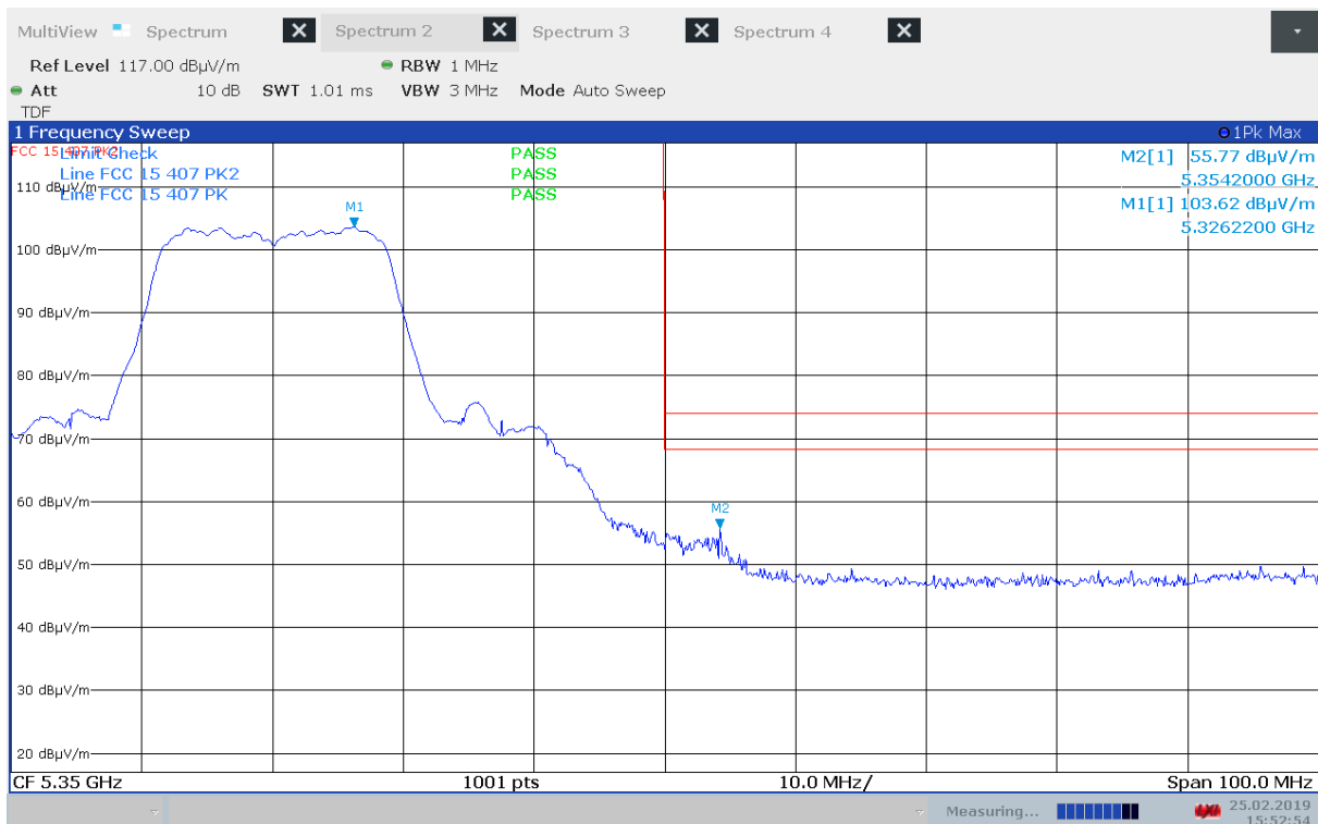
Unwanted Emissions, Band Edge, 5350 MHz, Ch064, 802.11n MCS0, Radiated
