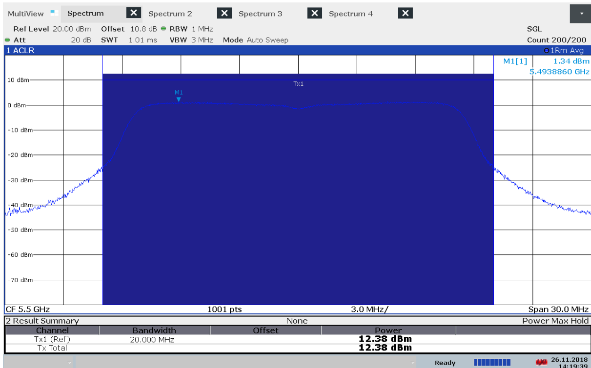
Output Power, 5500 MHz, Method 1, 802.11n MCS0, Conducted
