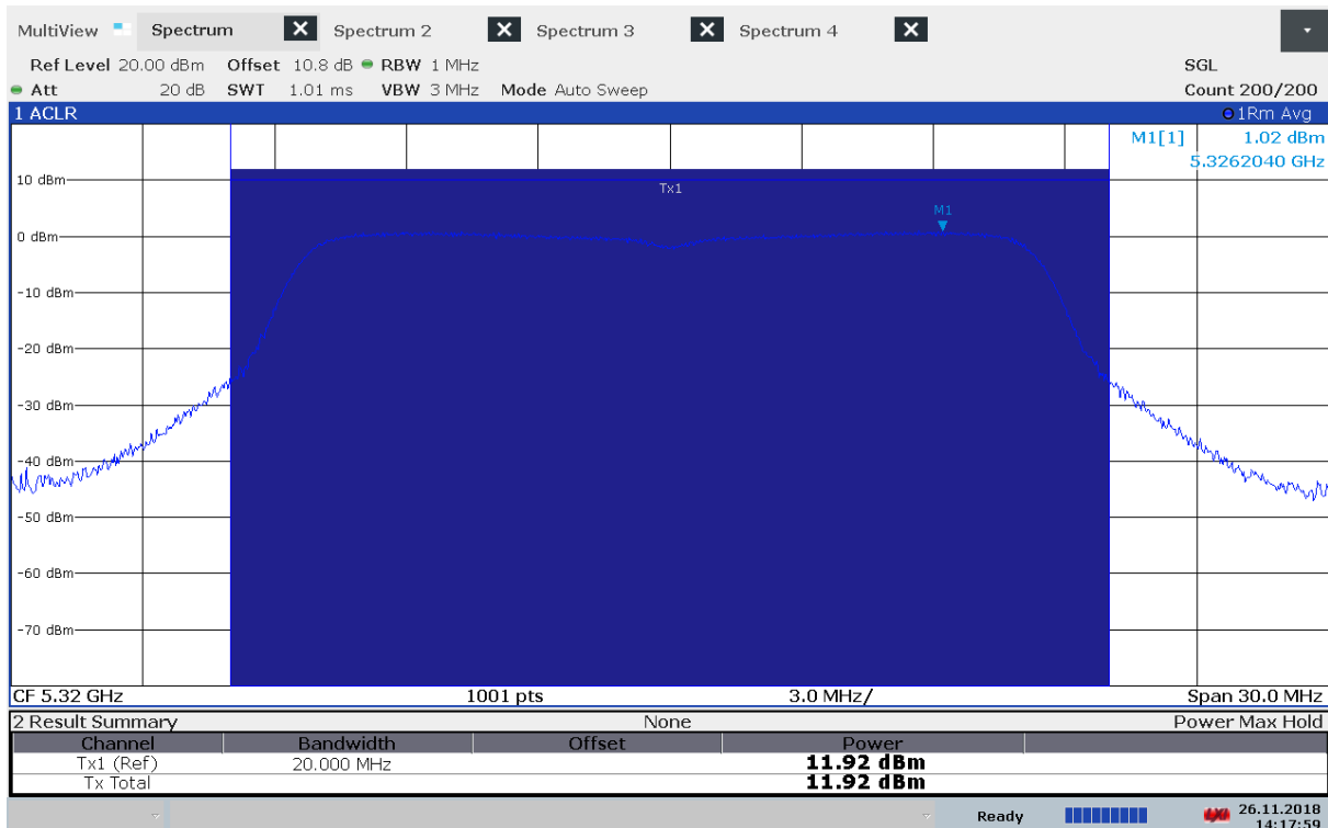
Output Power, 5320 MHz, Method 1, 802.11n MCS0, Conducted
