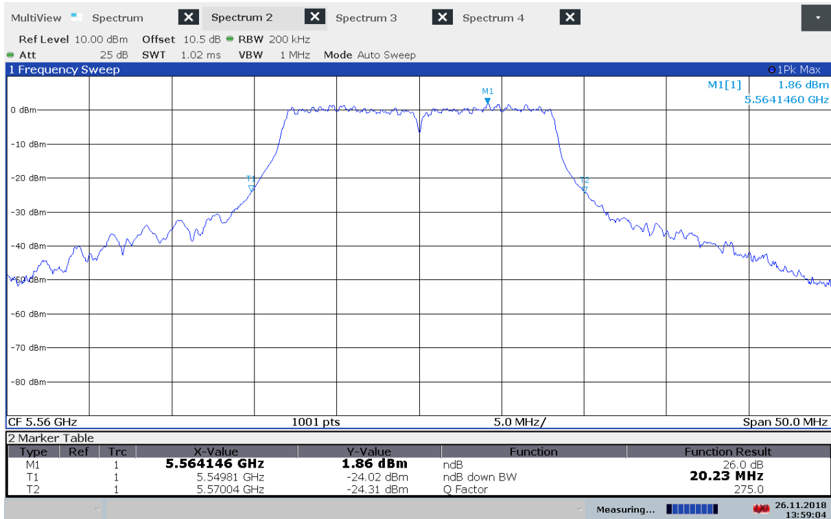
Emission Bandwidth B, 5560 MHz, 802.11a 6Mbps
