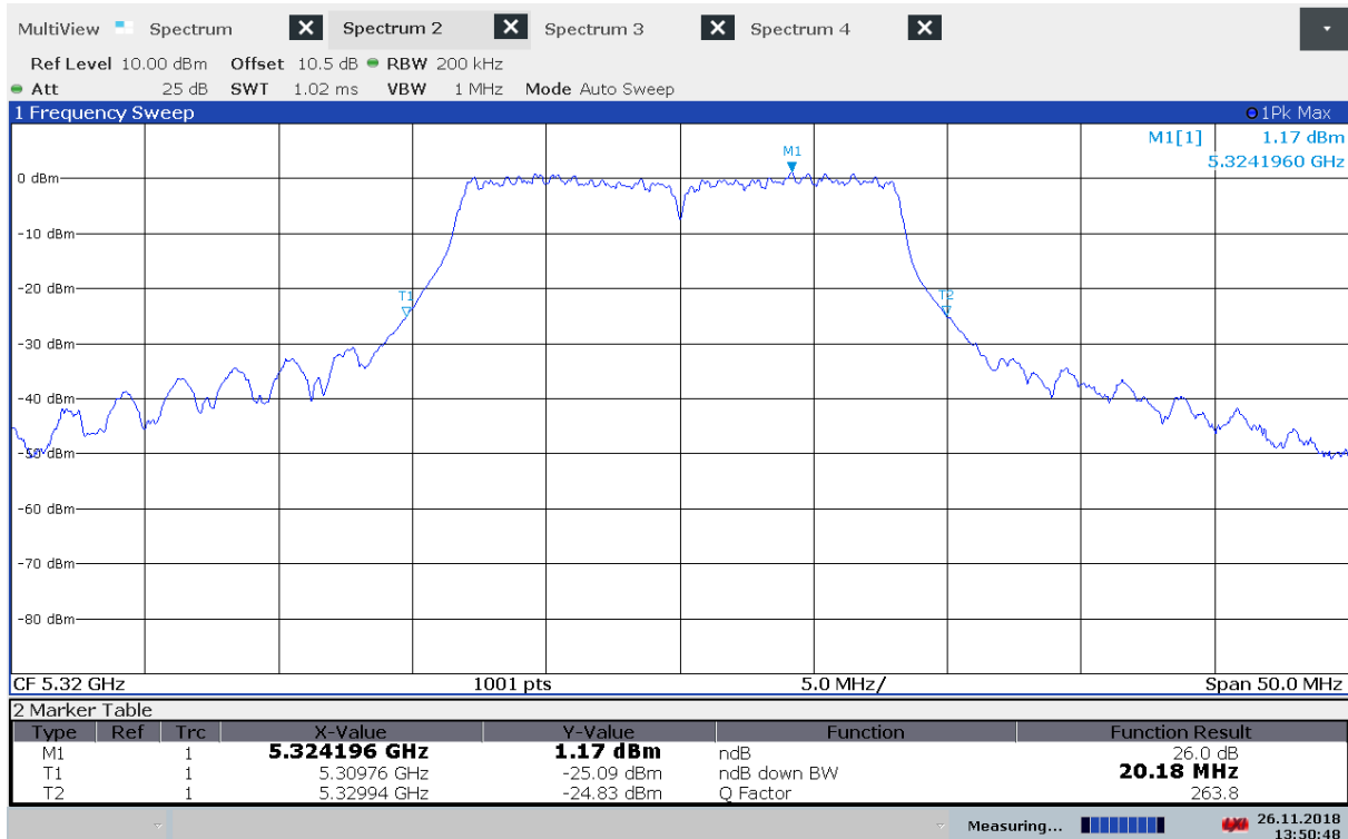
Emission Bandwidth B, 5320 MHz, 802.11a 6Mbps
