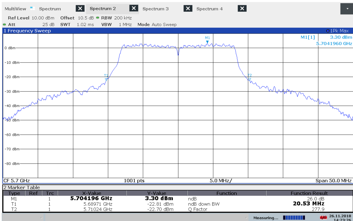
Emission Bandwidth B, 5700 MHz, 802.11n MCS0
