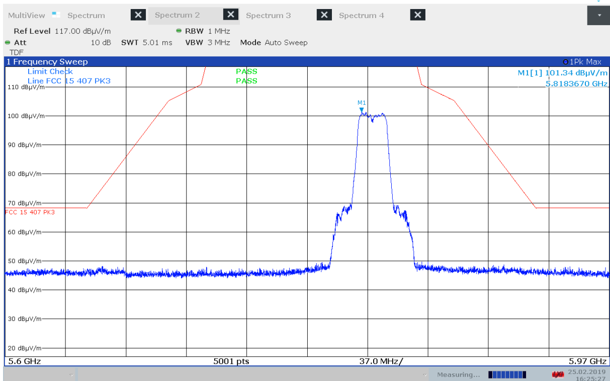
Unwanted Emissions, Band Edge, 5825 MHz, Ch165, 802.11n MCS0, Radiated
