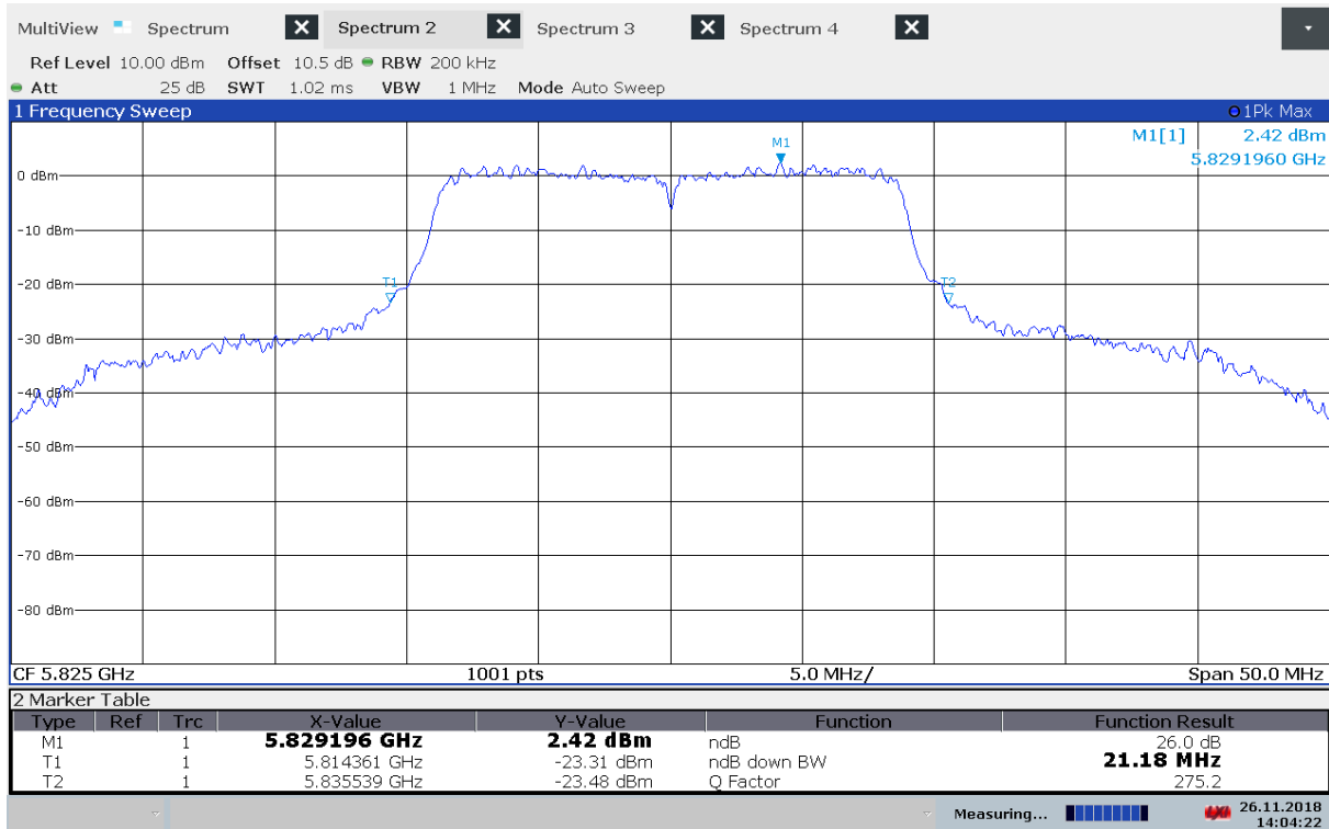
Emission Bandwidth B, 5825 MHz, 802.11a 6Mbps
