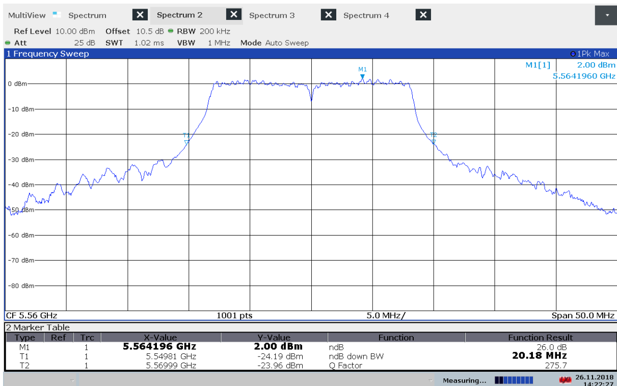
Emission Bandwidth B, 5560 MHz, 802.11n MCS0
