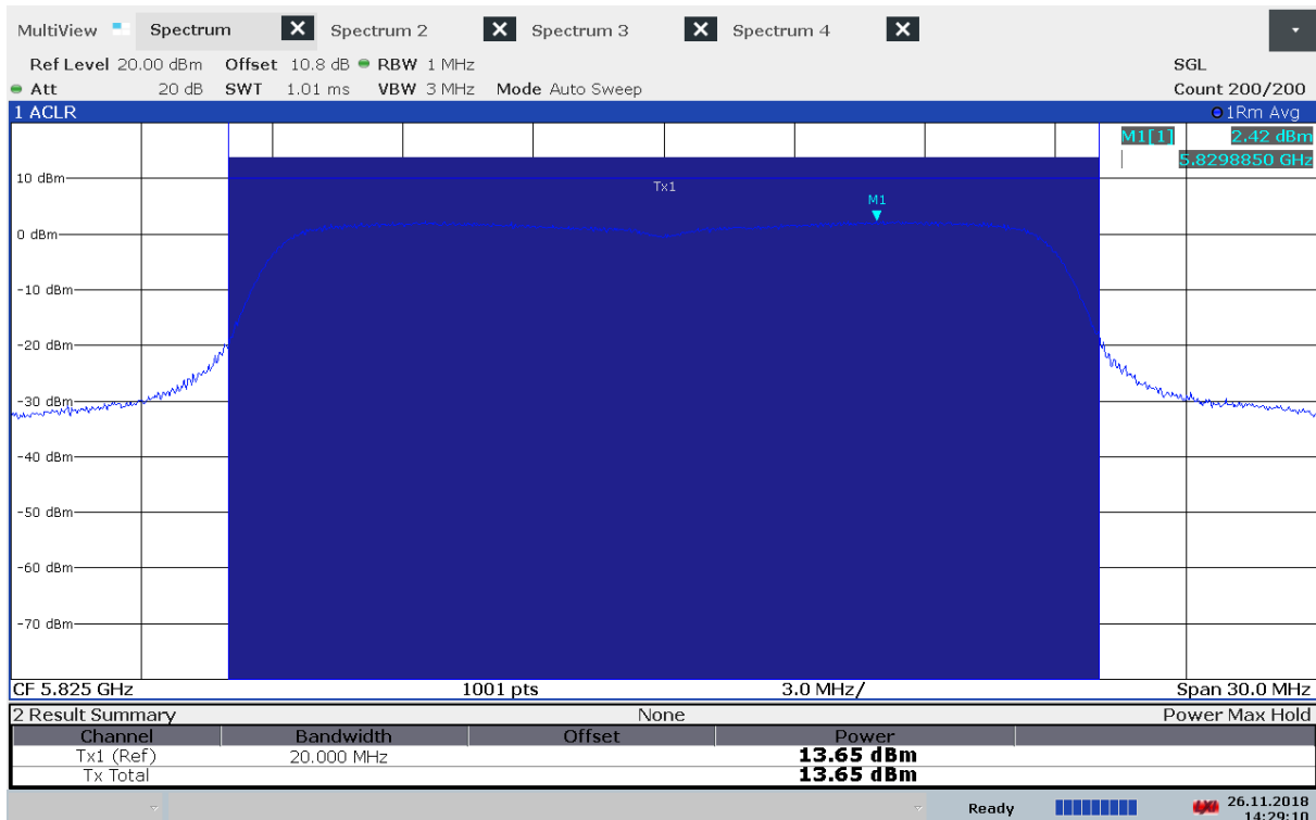
Output Power, 5825 MHz, Method 1, 802.11n MCS0, Conducted
