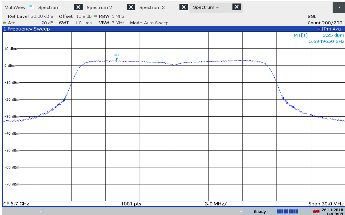
Power Spectral Density, 5700 MHz, 802.11a - 6Mbps, Method 2
