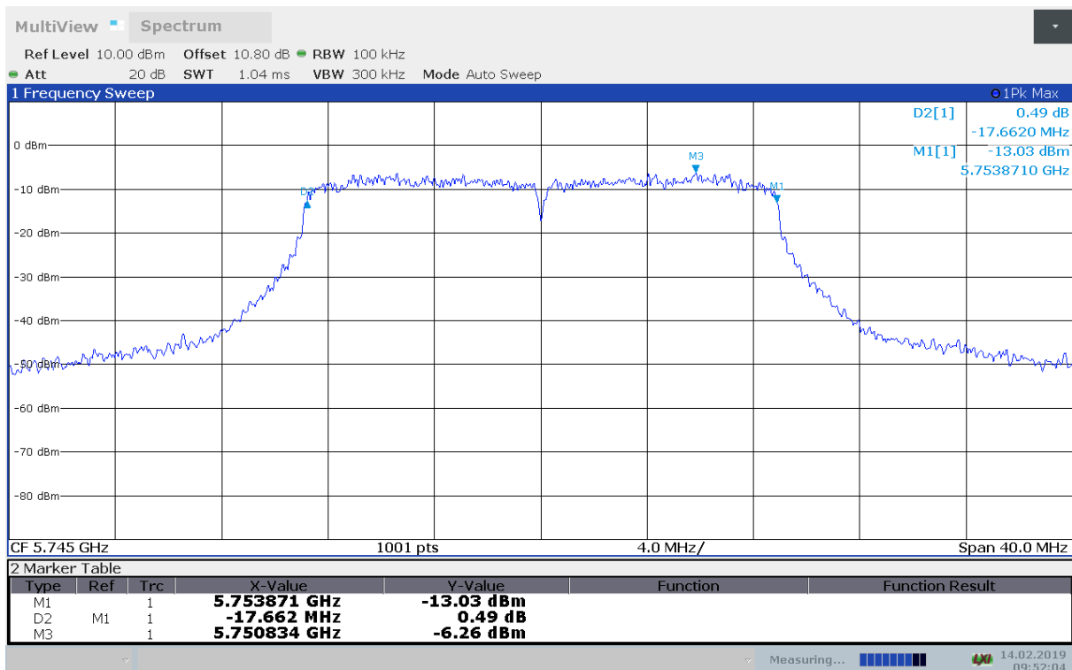
6 dB Bandwidth, 5745 MHz, 802.11n MCS0
