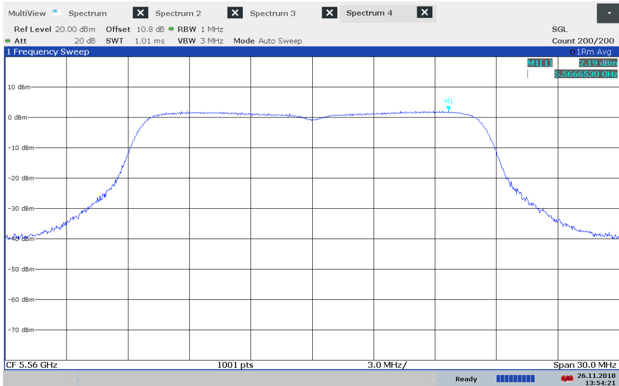
Power Spectral Density, 5560 MHz, 802.11a - 6Mbps, Method 2
