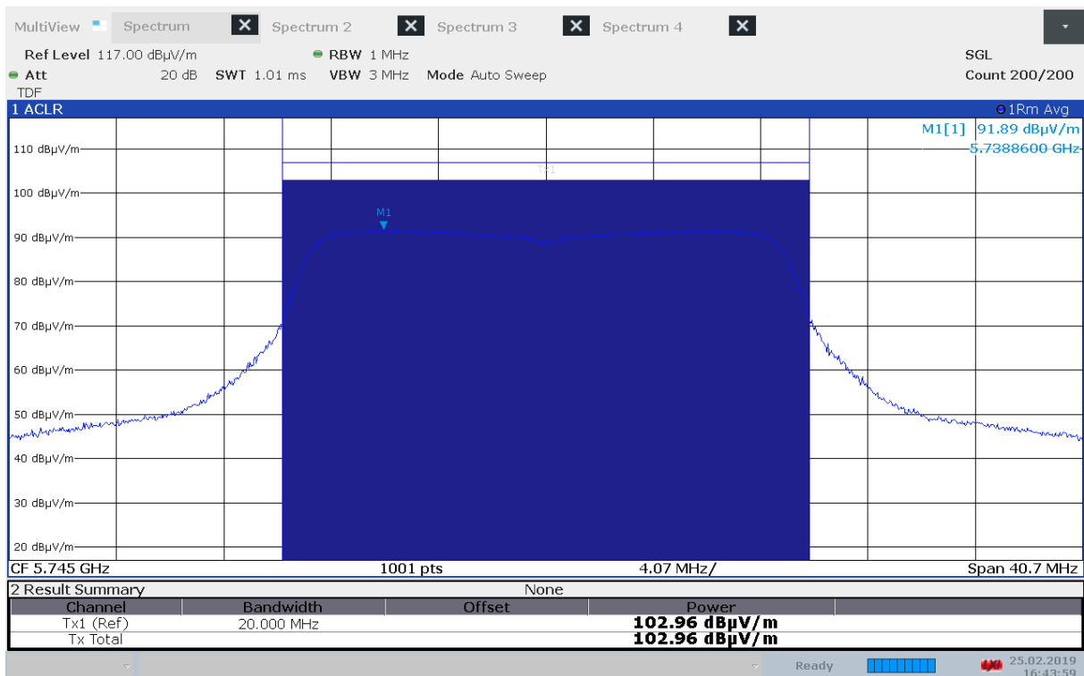
Maximum Field Strength, 5745 MHz, Method 1, 802.11n MCS0
