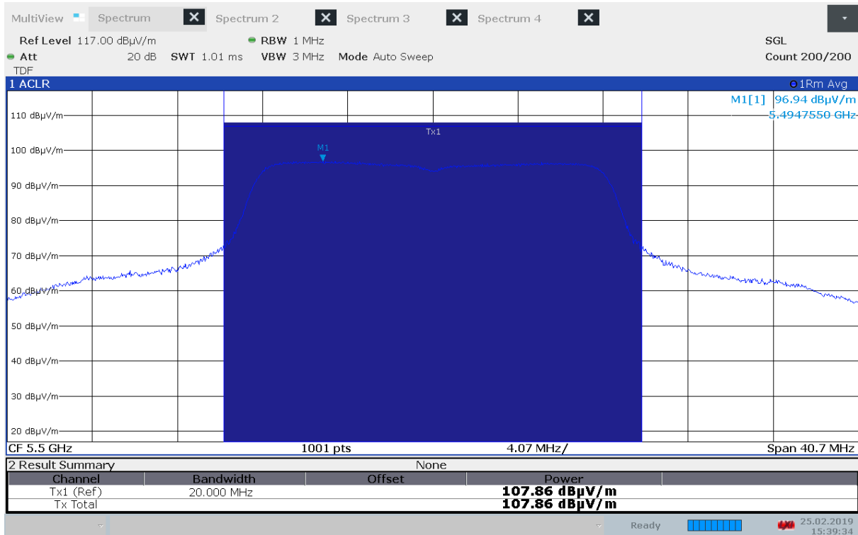
Maximum Field Strength, 5500 MHz, Method 1, 802.11a 6Mbps
