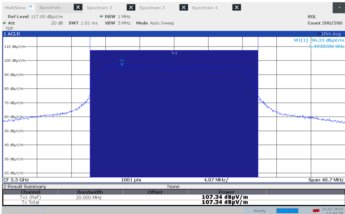
Maximum Field Strength, 5500 MHz, Method 1, 802.11n MCS0
