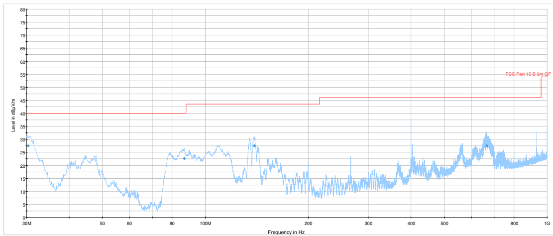
Radiated Emissions, 30– 1000 MHz, 5180MHz, 802.11a 6Mbps, EUT V
