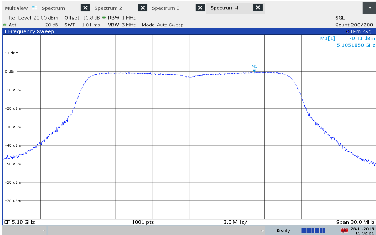
Power Spectral Density, 5180 MHz, 802.11a - 6Mbps, Method 2
