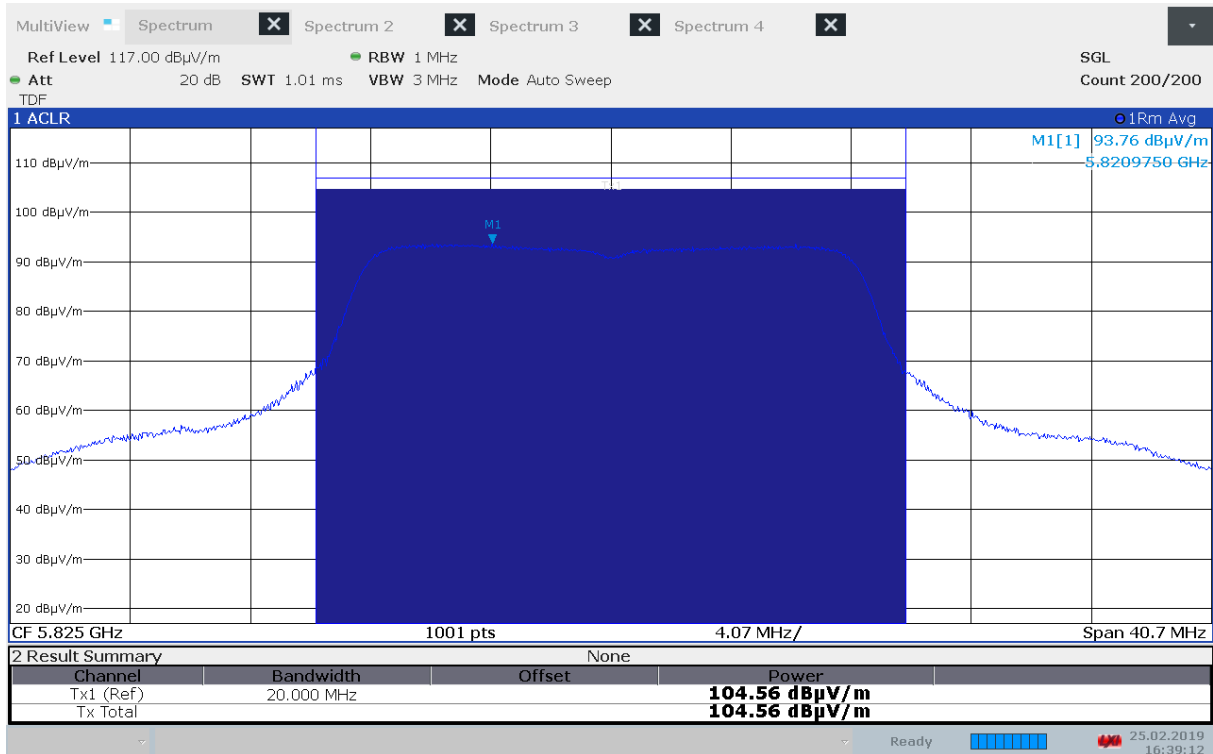
Maximum Field Strength, 5825 MHz, Method 1, 802.11a 6Mbps
