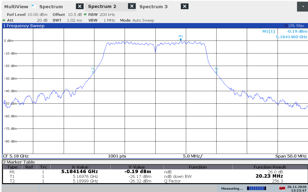
Emission Bandwidth B, 5180 MHz, 802.11a 6Mbps
