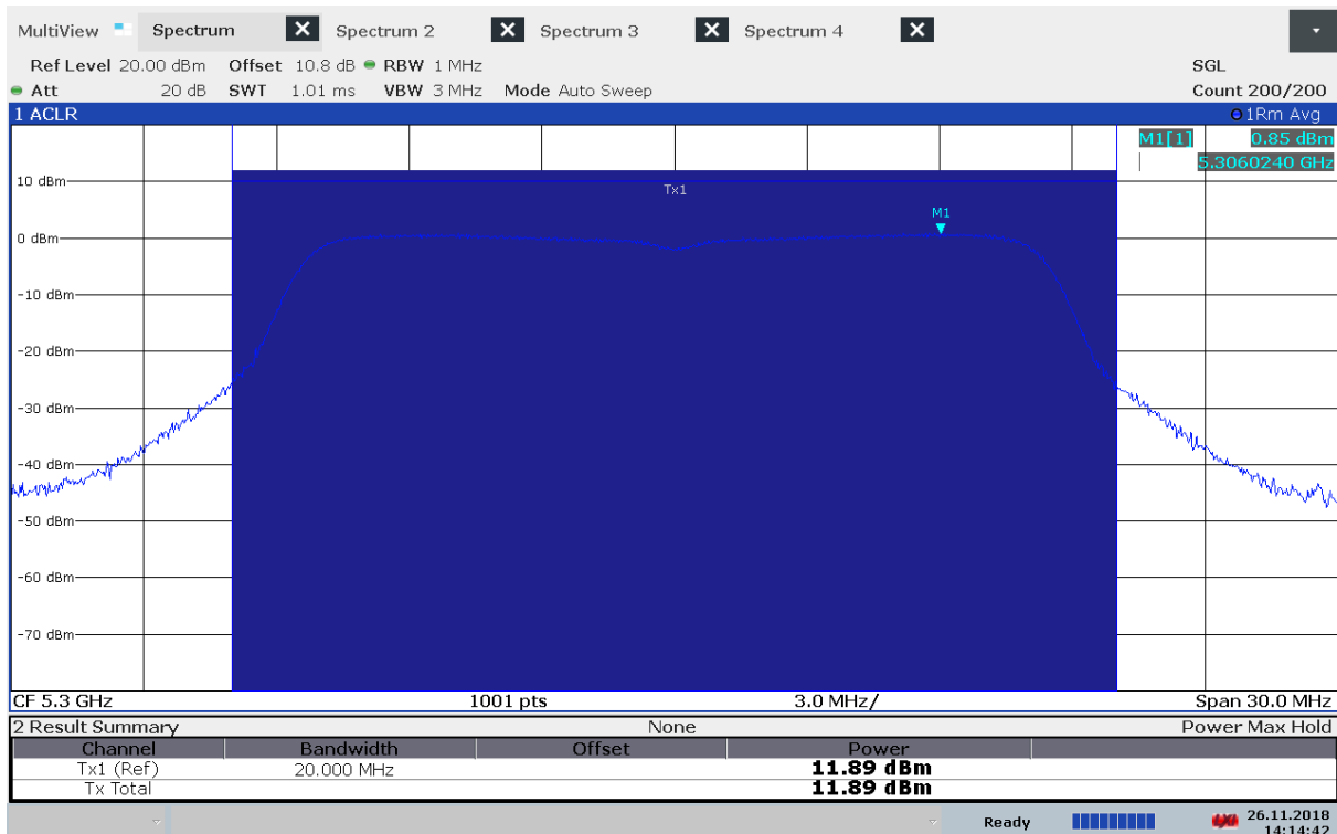
Output Power, 5300 MHz, Method 1, 802.11n MCS0, Conducted
