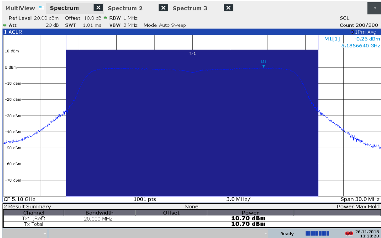
Output Power, 5180 MHz, Method 1, 802.11a 6Mbps, Conducted
