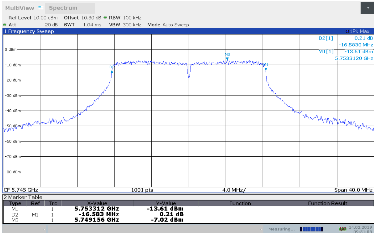
6 dB Bandwidth, 5745 MHz, 802.11a 6Mbps
