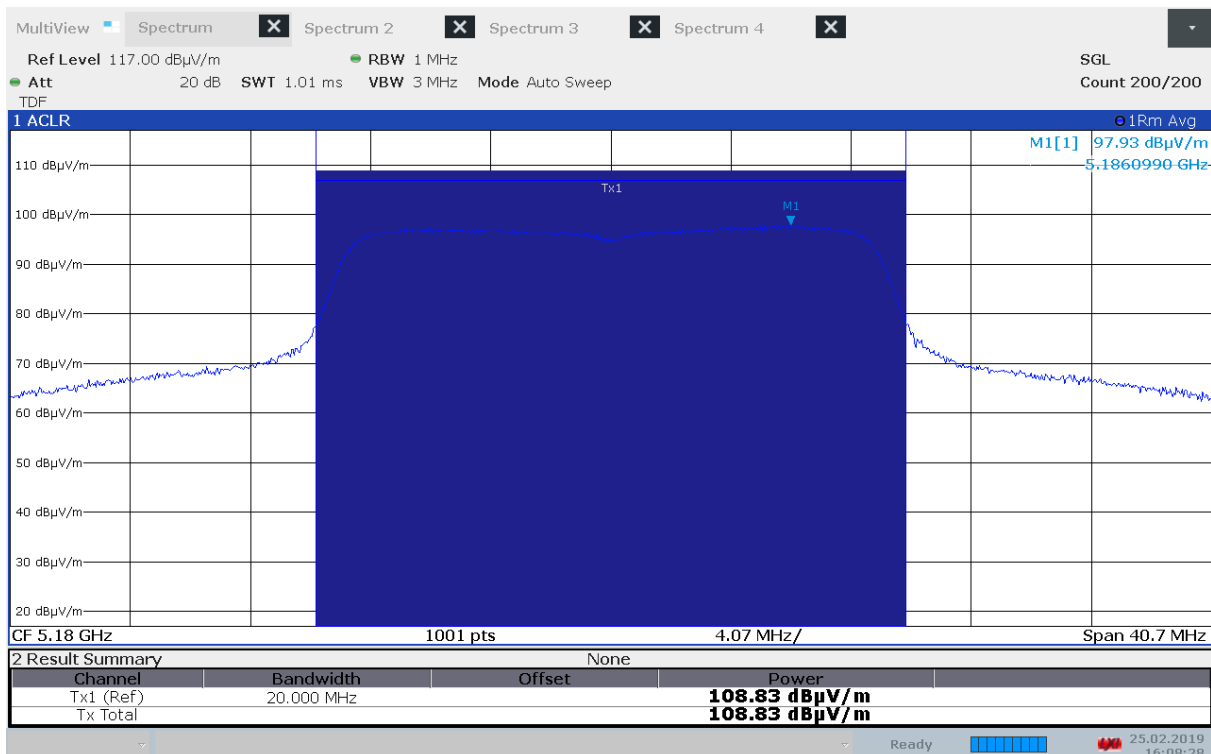
Maximum Field Strength, 5180 MHz, Method 1, 802.11n MCS0
