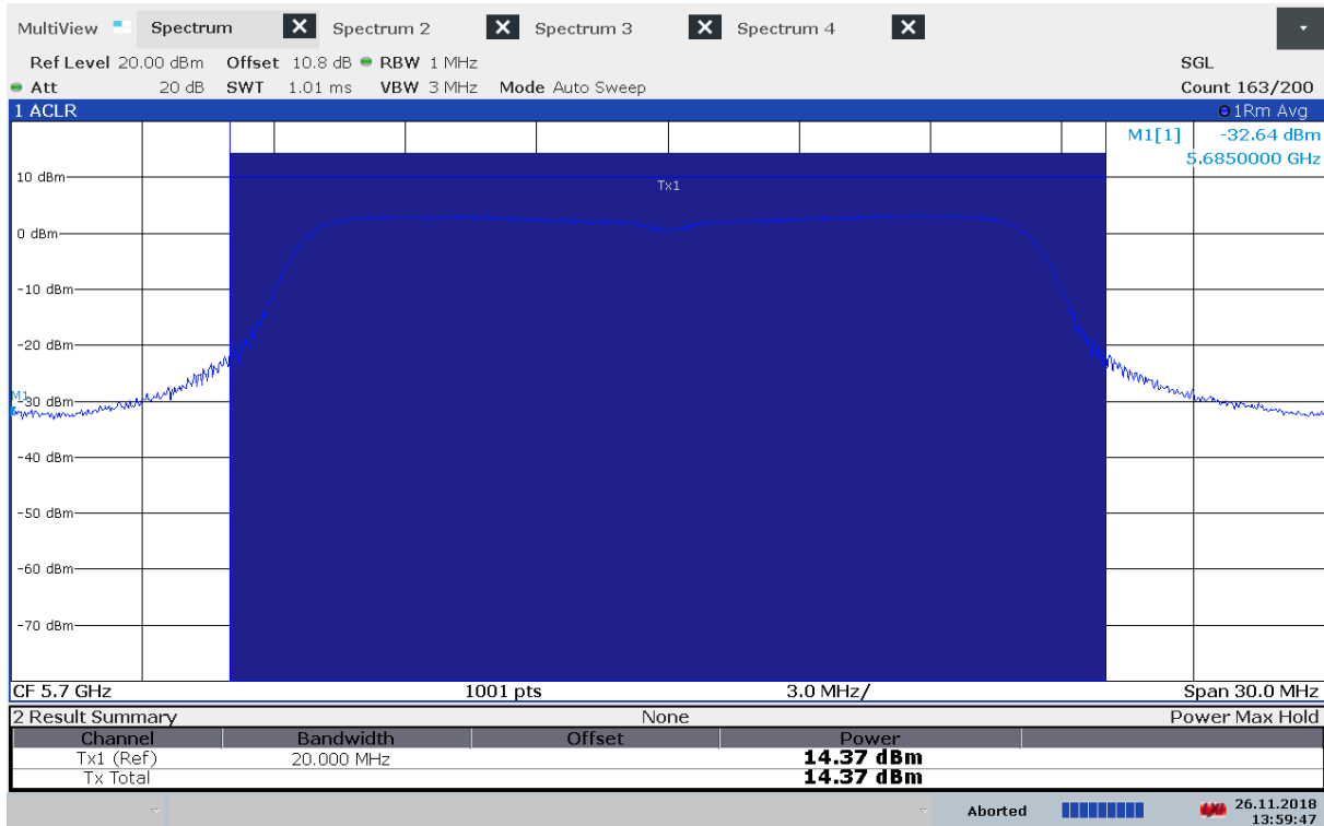
Output Power, 5700 MHz, Method 1, 802.11a 6Mbps, Conducted
