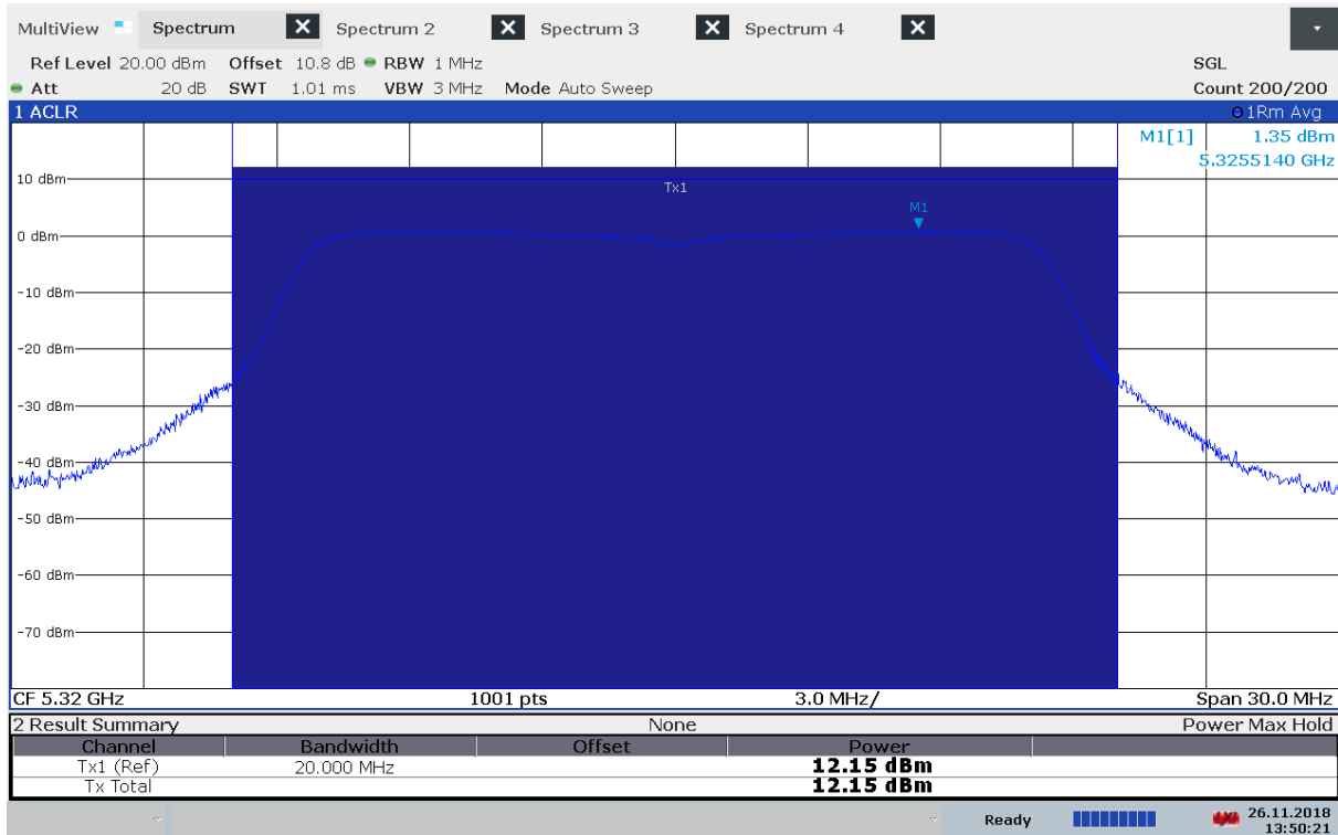
Output Power, 5320 MHz, Method 1, 802.11a 6Mbps, Conducted
