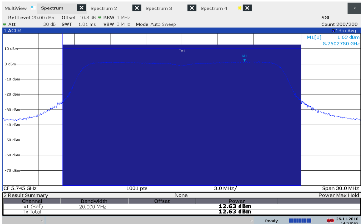
Output Power, 5745 MHz, Method 1, 802.11n MCS0, Conducted
