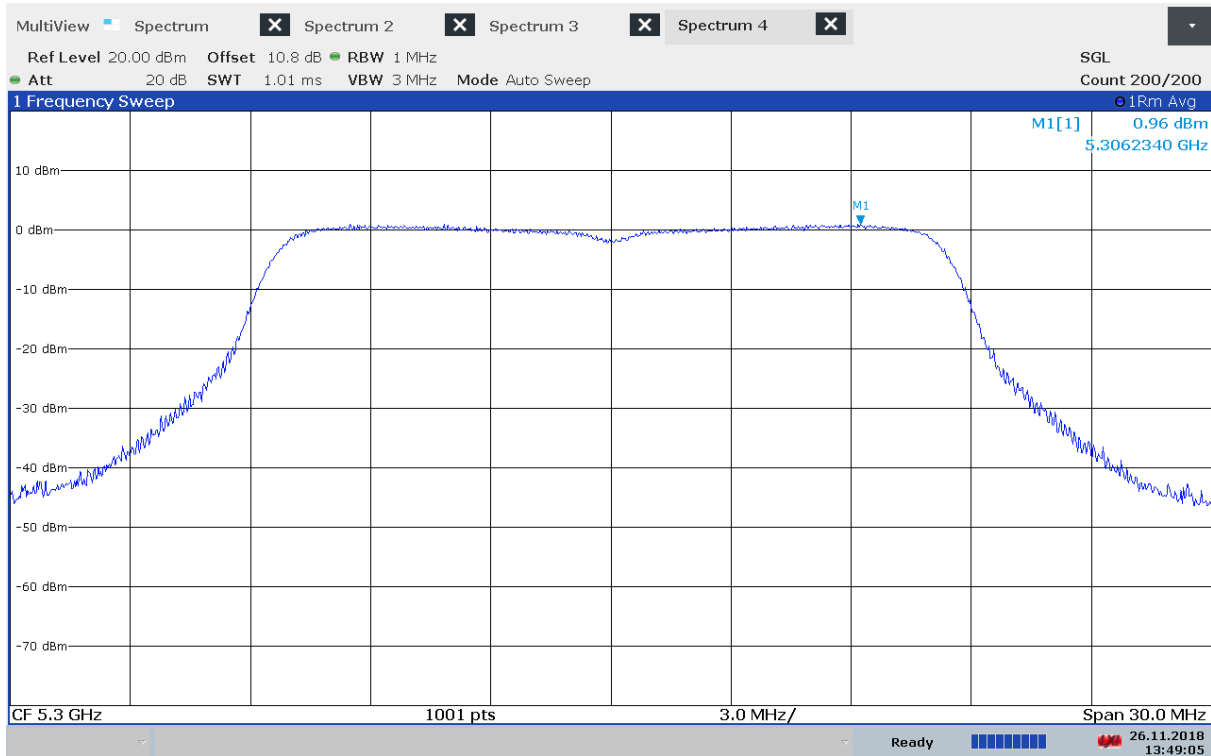
Power Spectral Density, 5300 MHz, 802.11a - 6Mbps, Method 2
