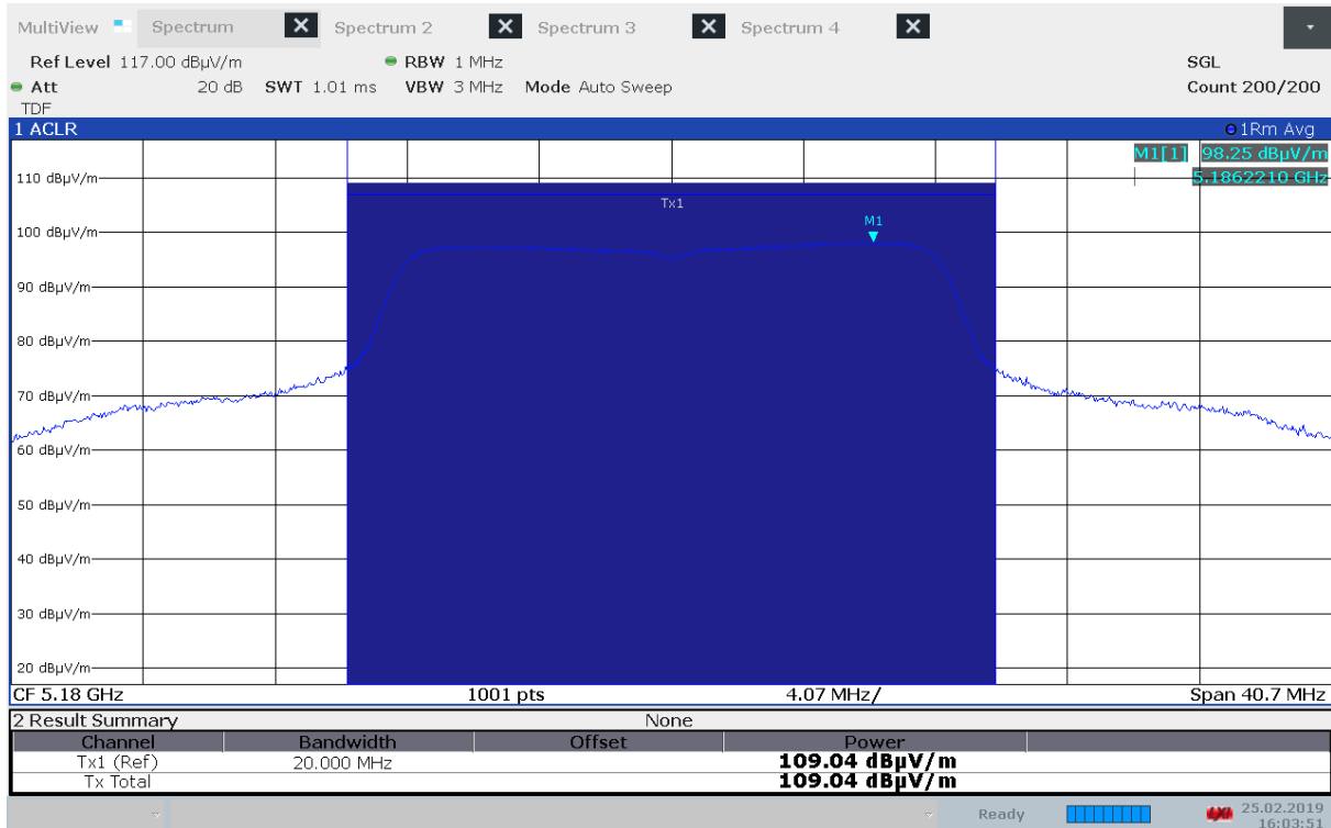
Maximum Field Strength, 5180 MHz, Method 1, 802.11a 6Mbps
