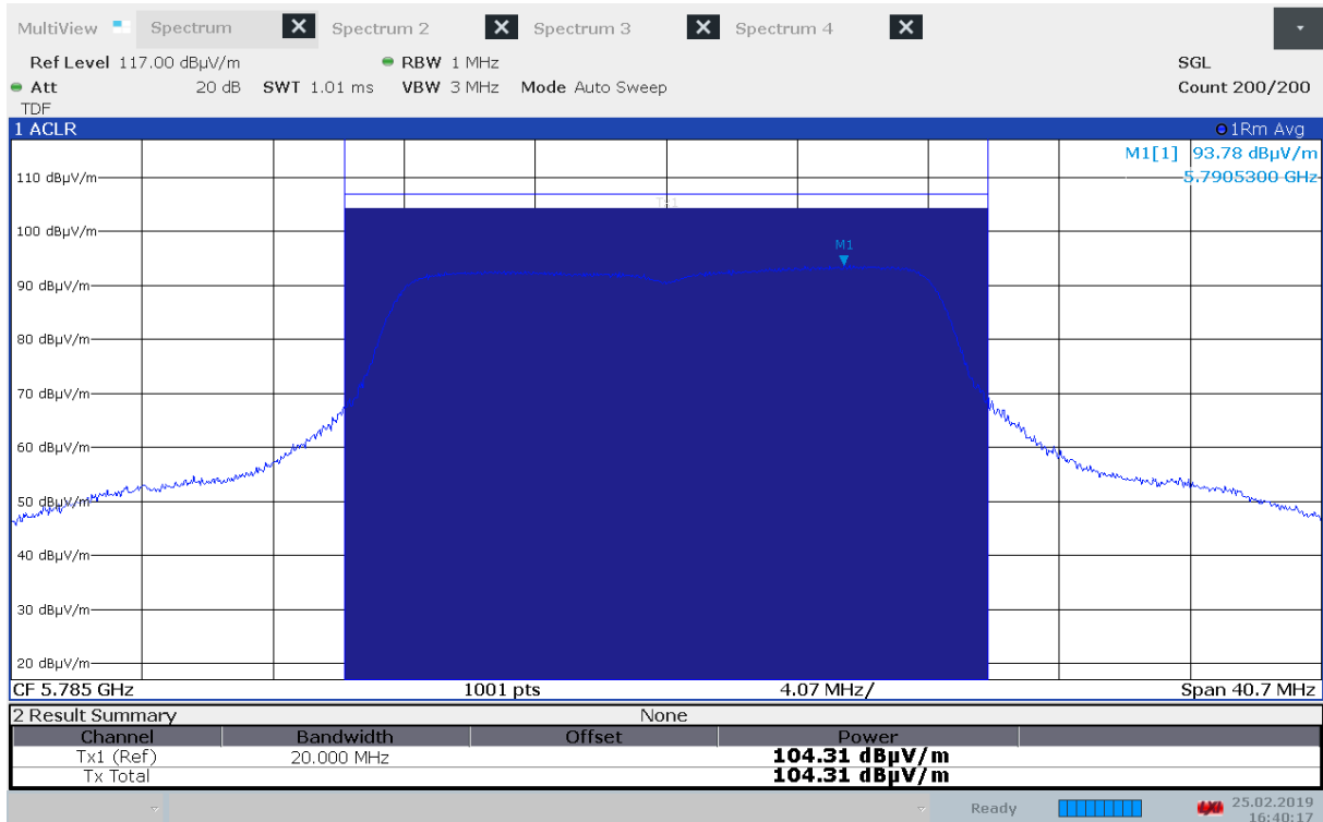
Maximum Field Strength, 5785 MHz, Method 1, 802.11a 6Mbps
