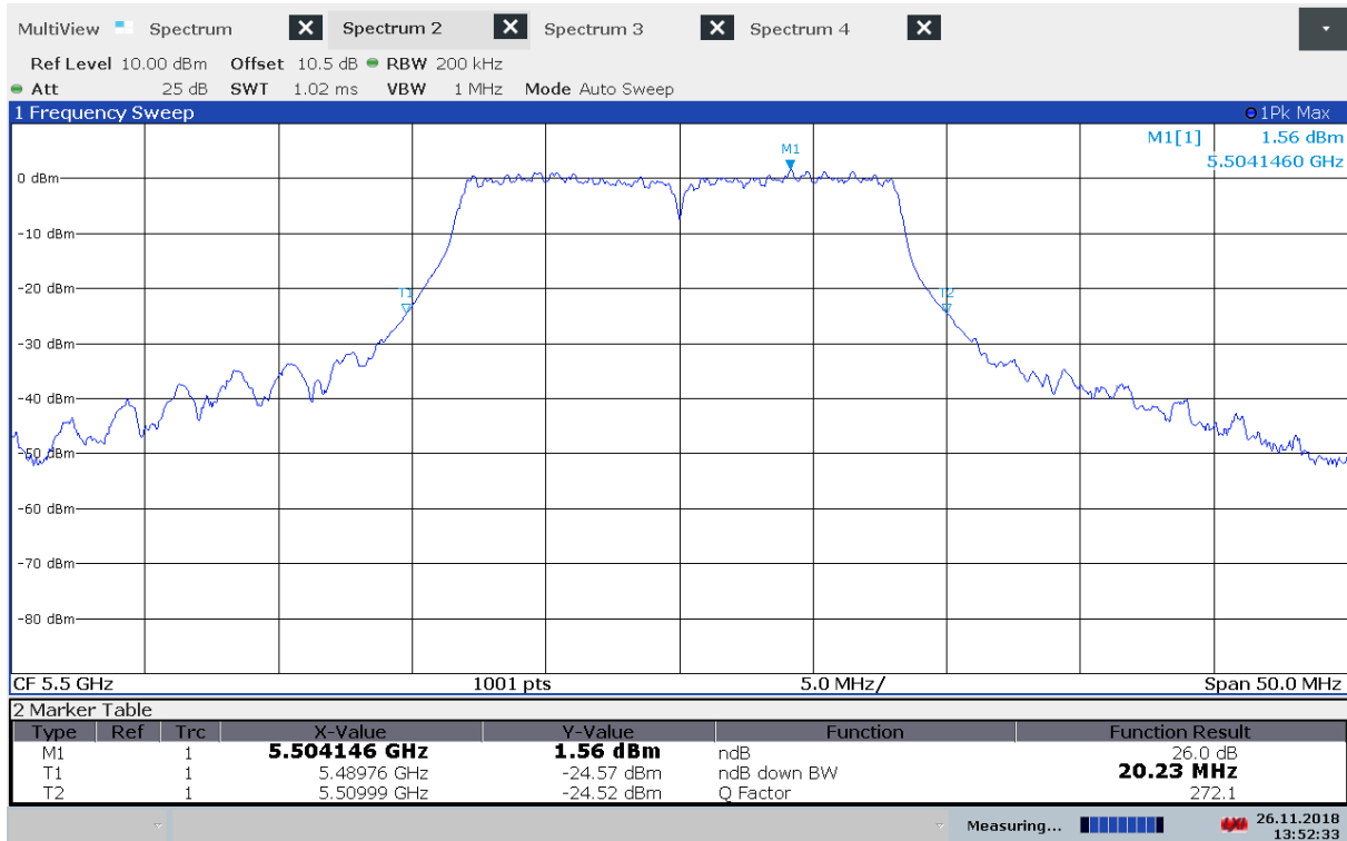
Emission Bandwidth B, 5500 MHz, 802.11a 6Mbps
