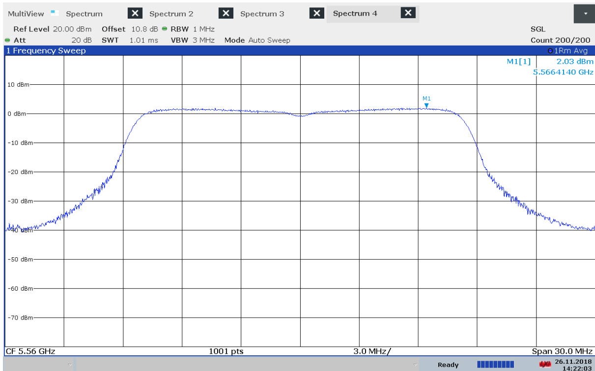
Power Spectral Density, 5560 MHz, 802.11n - MCS0, Method 2
