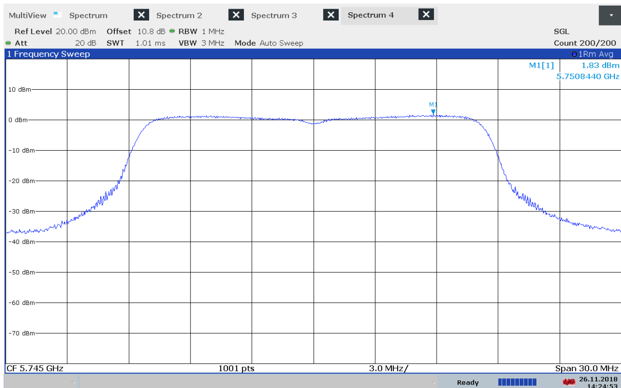
Power Spectral Density, 5745 MHz, 802.11n - MCS0, Method 2
