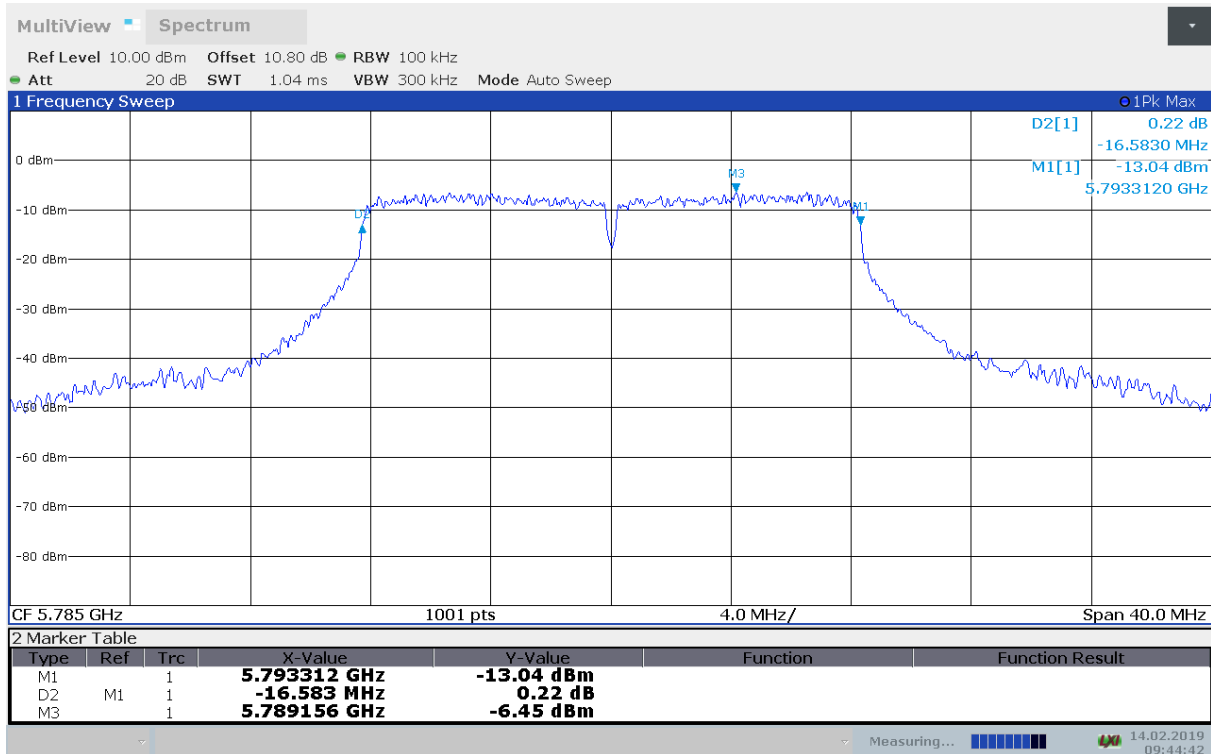
6 dB Bandwidth, 5785 MHz, 802.11a 6Mbps
