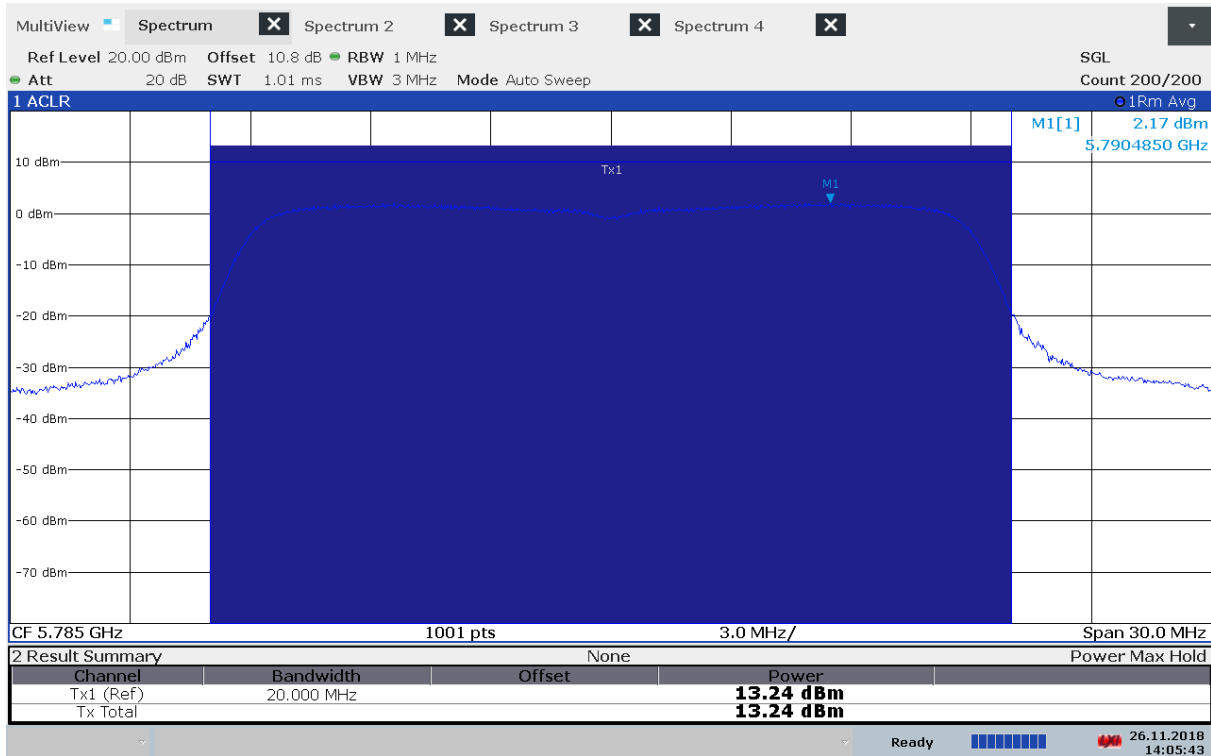
Output Power, 5785 MHz, Method 1, 802.11a 6Mbps, Conducted
