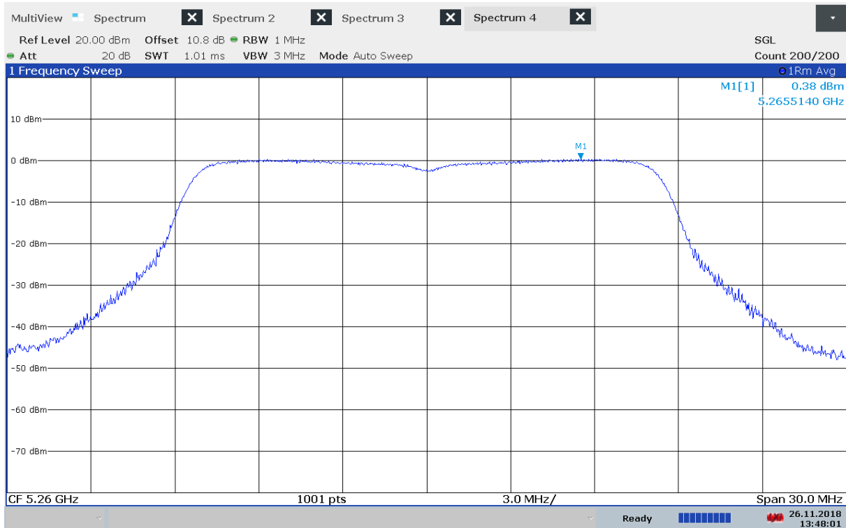
Power Spectral Density, 5260 MHz, 802.11a - 6Mbps, Method 2
