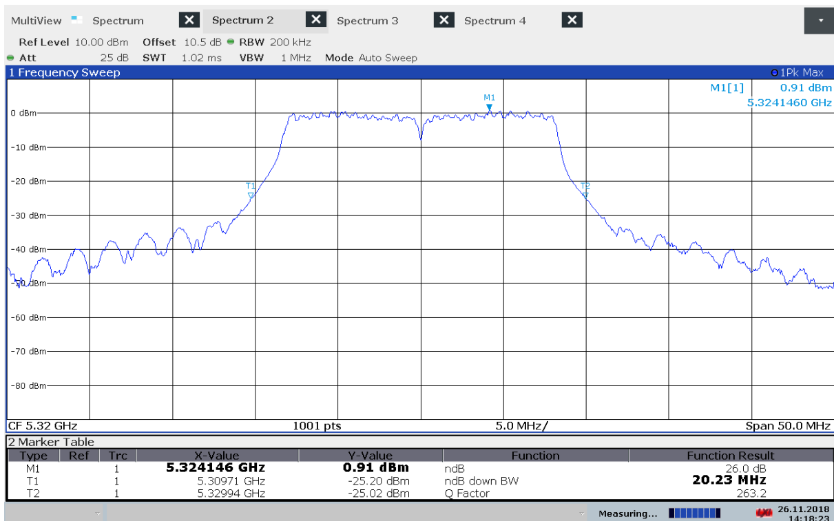
Emission Bandwidth B, 5320 MHz, 802.11n MCS0
