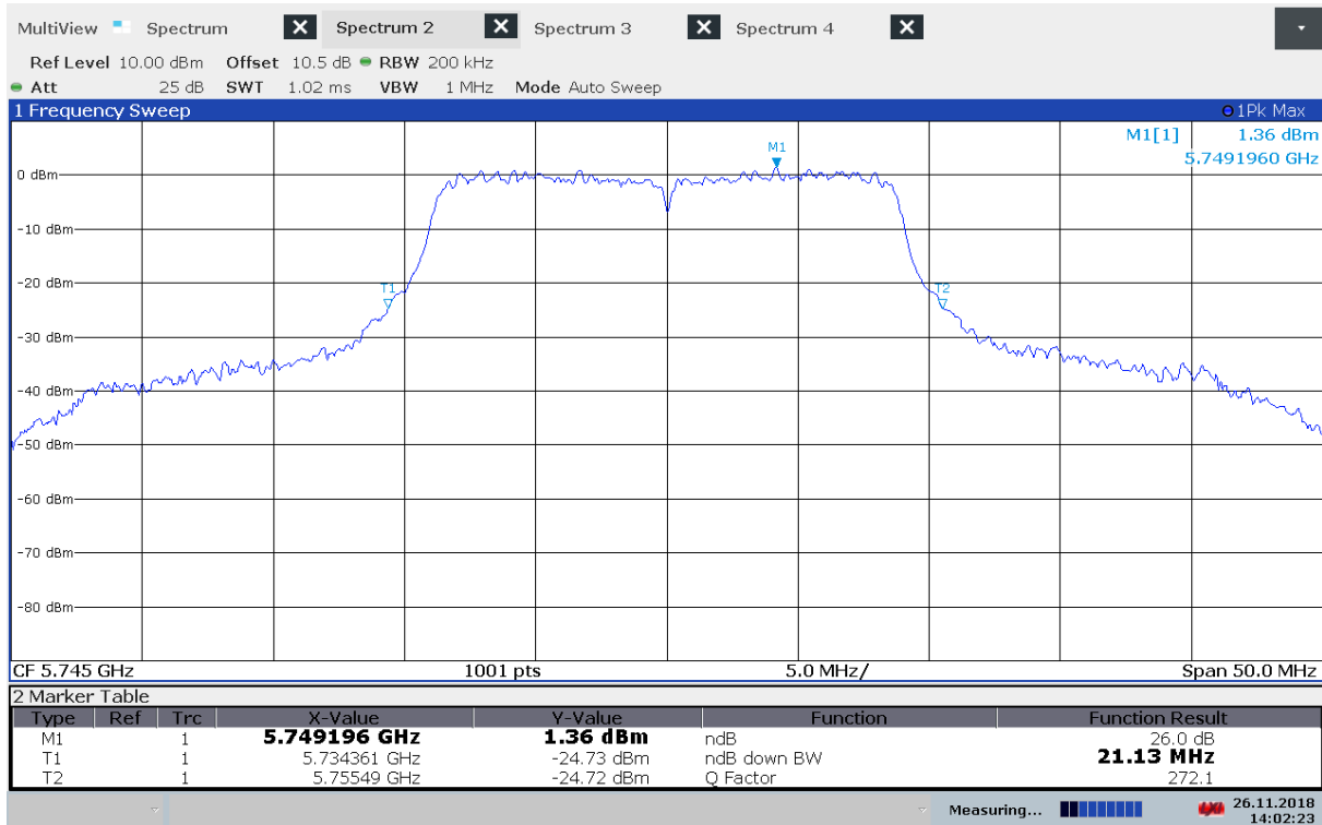
Emission Bandwidth B, 5745 MHz, 802.11a 6Mbps
