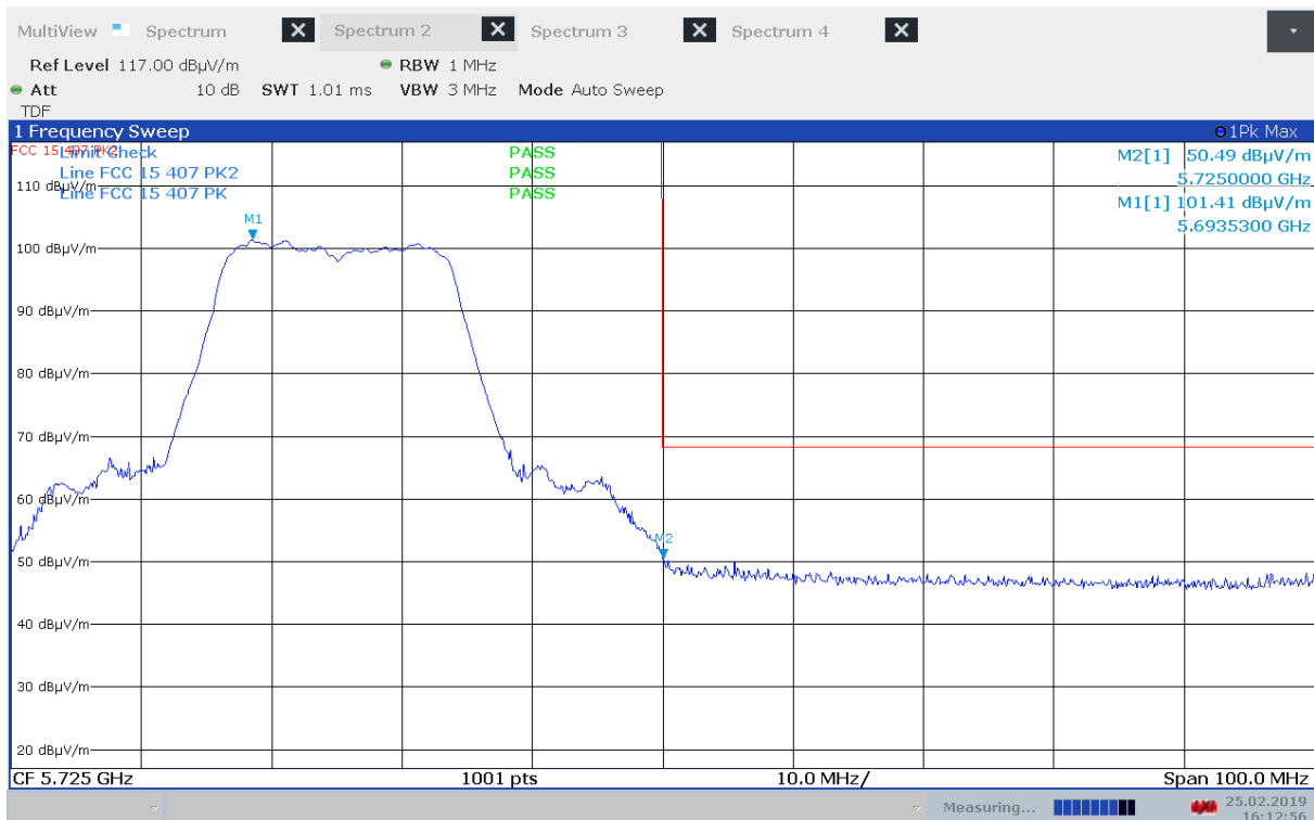
Unwanted Emissions, Band Edge, 5725 MHz, Ch140, 802.11n MCS0, Radiated
