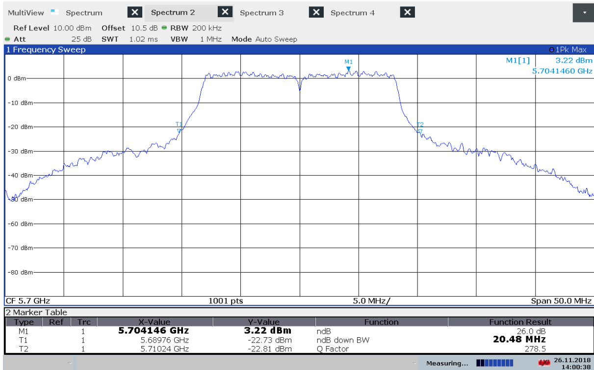
Emission Bandwidth B, 5700 MHz, 802.11a 6Mbps
