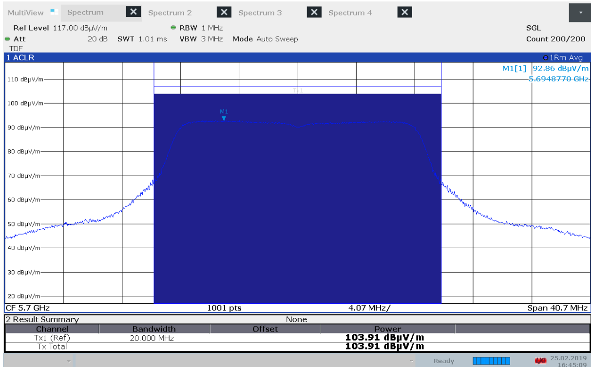
Maximum Field Strength, 5700 MHz, Method 1, 802.11a 6Mbps
