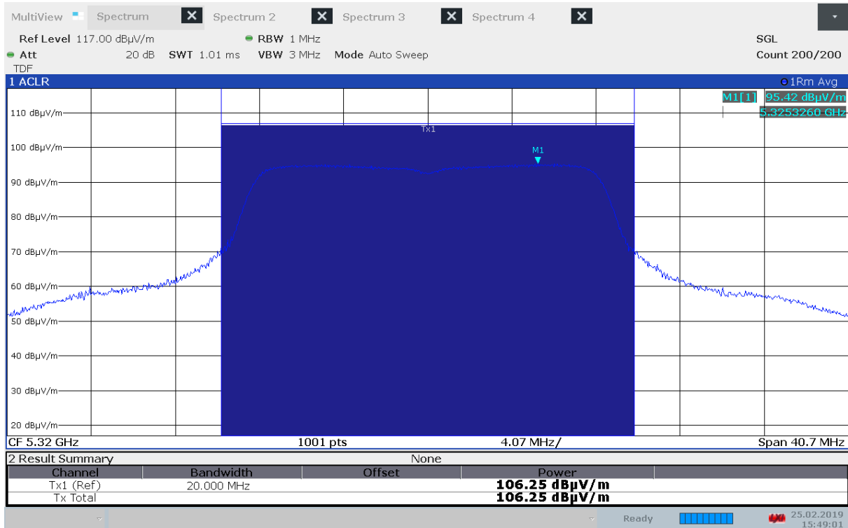
Maximum Field Strength, 5320 MHz, Method 1, 802.11a 6Mbps
