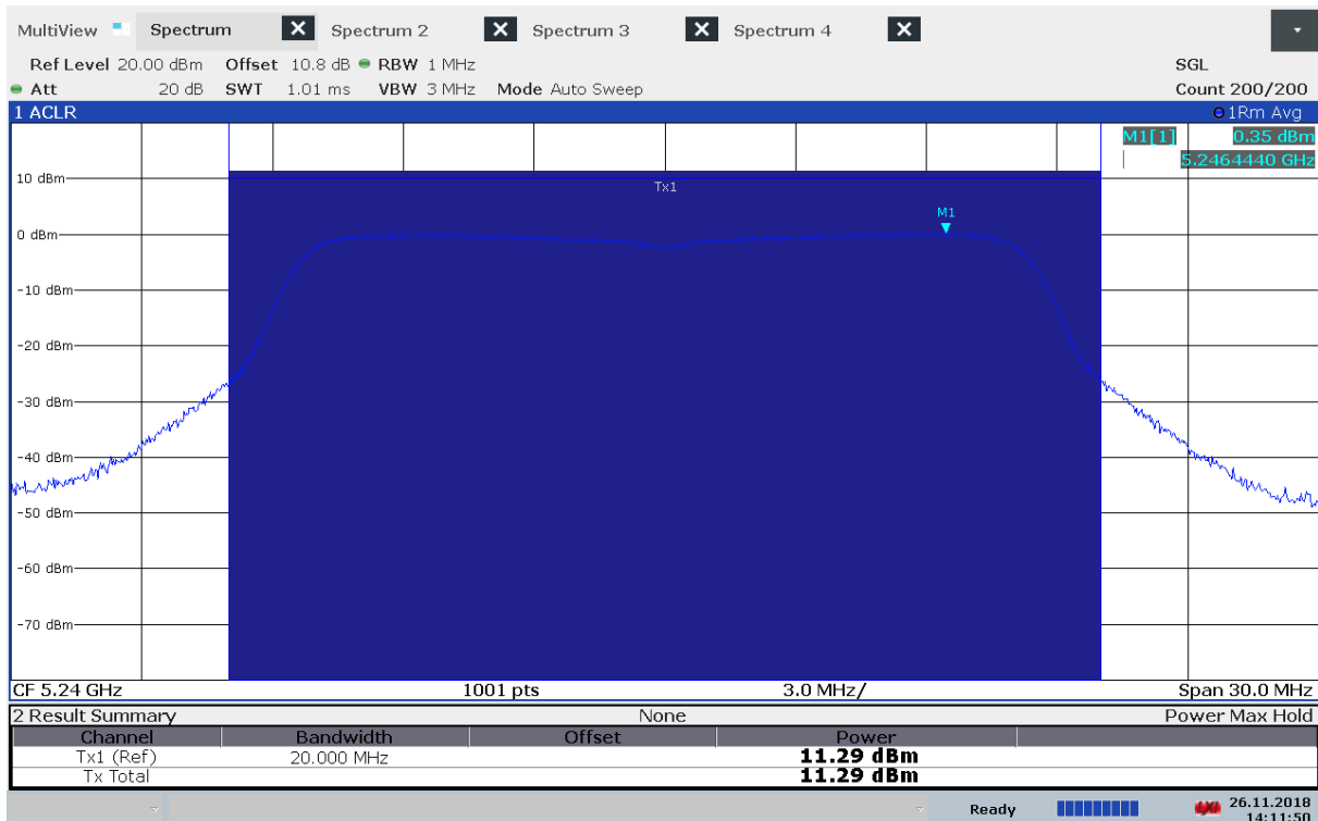
Output Power, 5240 MHz, Method 1, 802.11n MCS0, Conducted
