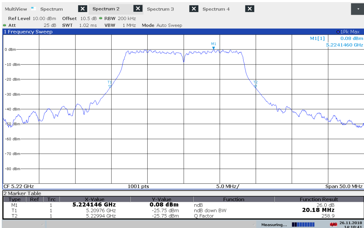
Emission Bandwidth B, 5220 MHz, 802.11n MCS0
