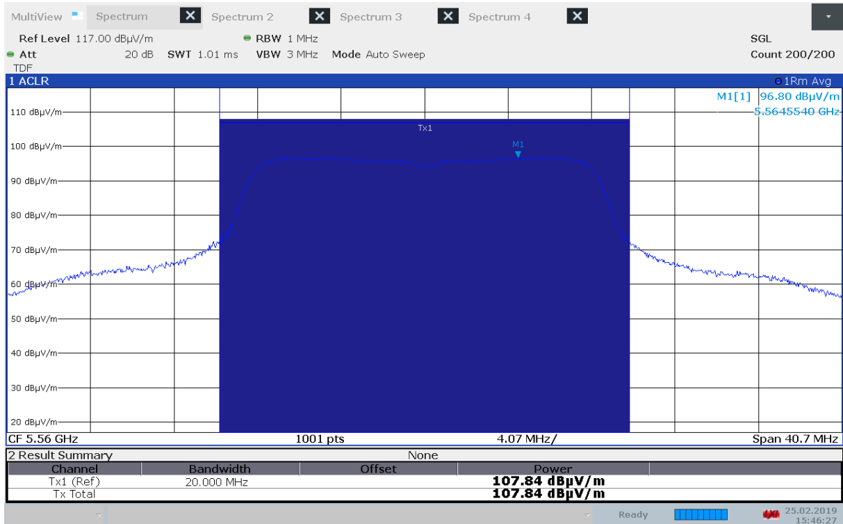
Maximum Field Strength, 5560 MHz, Method 1, 802.11a 6Mbps
