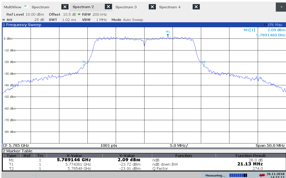
Emission Bandwidth B, 5785 MHz, 802.11n MCS0
