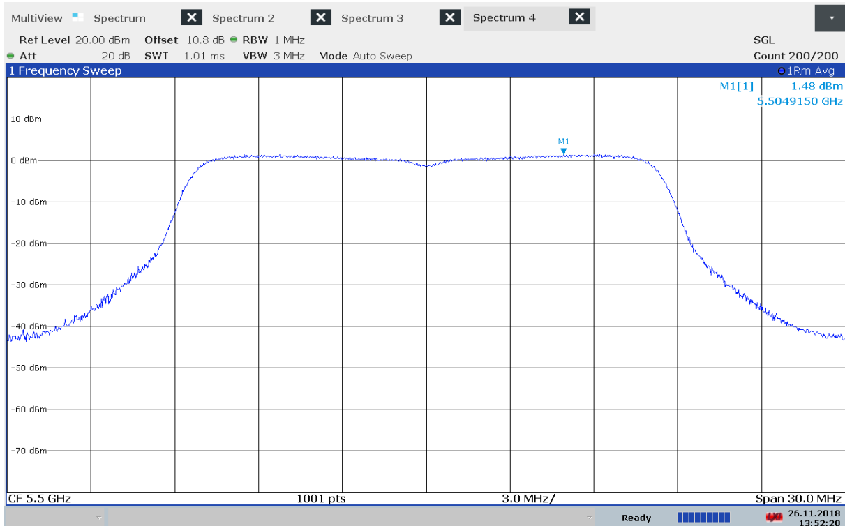
Power Spectral Density, 5500 MHz, 802.11a - 6Mbps, Method 2
