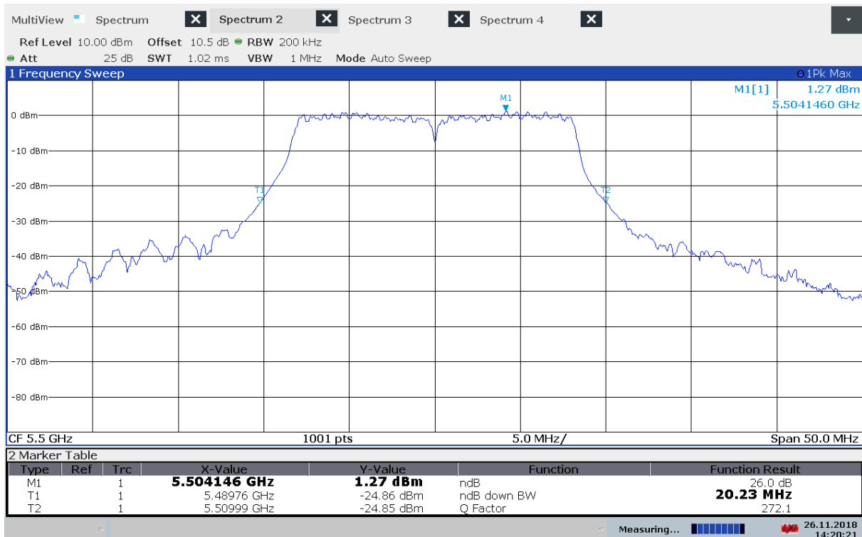
Emission Bandwidth B, 5500 MHz, 802.11n MCS0
