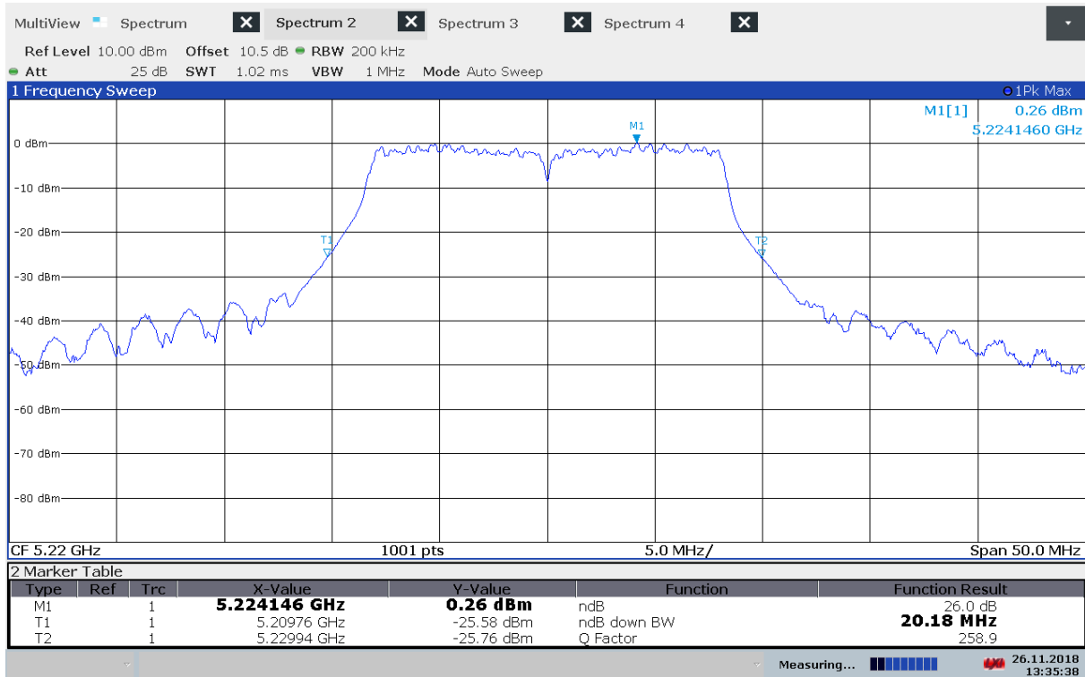
Emission Bandwidth B, 5220 MHz, 802.11a 6Mbps
