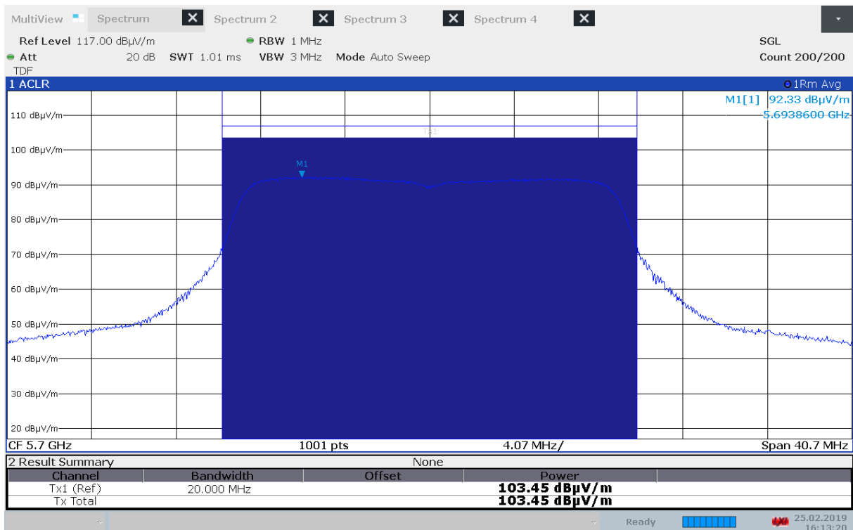
Maximum Field Strength, 5700 MHz, Method 1, 802.11n MCS0
