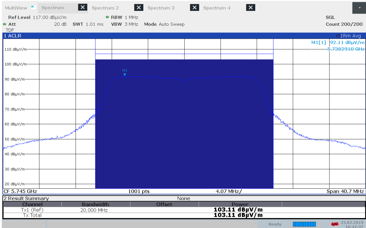
Maximum Field Strength, 5745 MHz, Method 1, 802.11a 6Mbps
