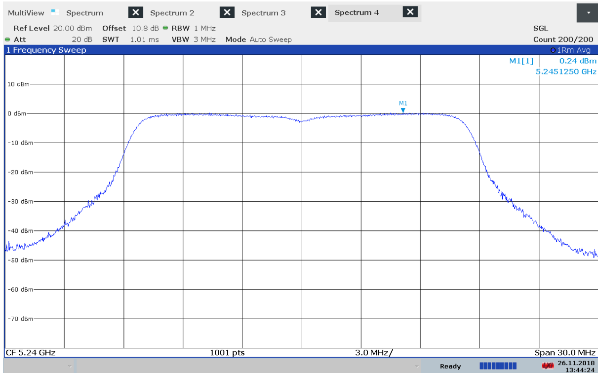
Power Spectral Density, 5240 MHz, 802.11a - 6Mbps, Method 2
