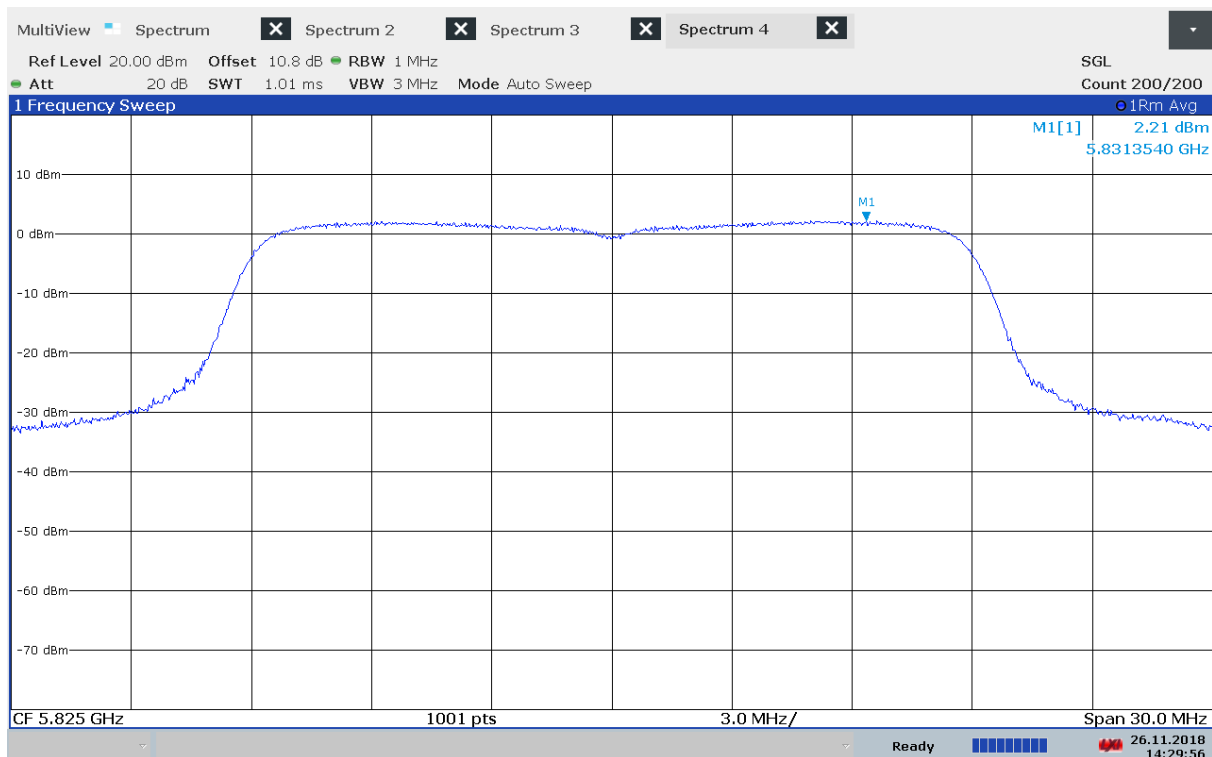
Power Spectral Density, 5825 MHz, 802.11n - MCS0, Method 2
