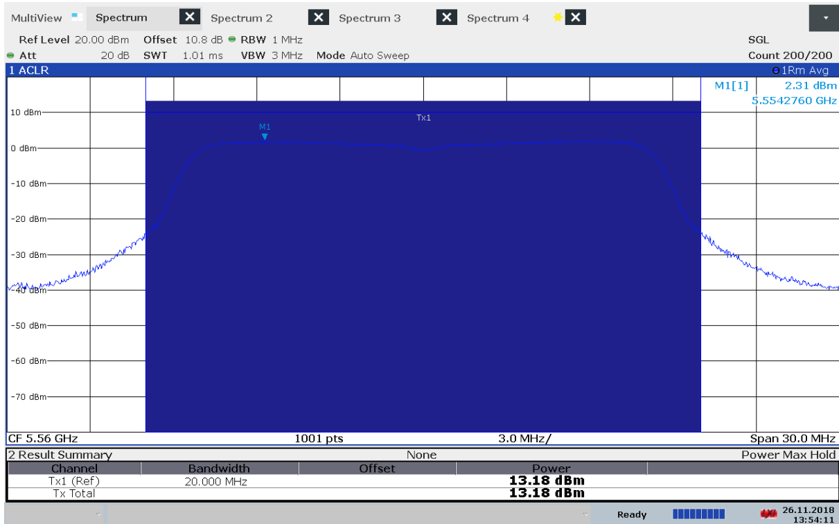
Output Power, 5560 MHz, Method 1, 802.11a 6Mbps, Conducted
