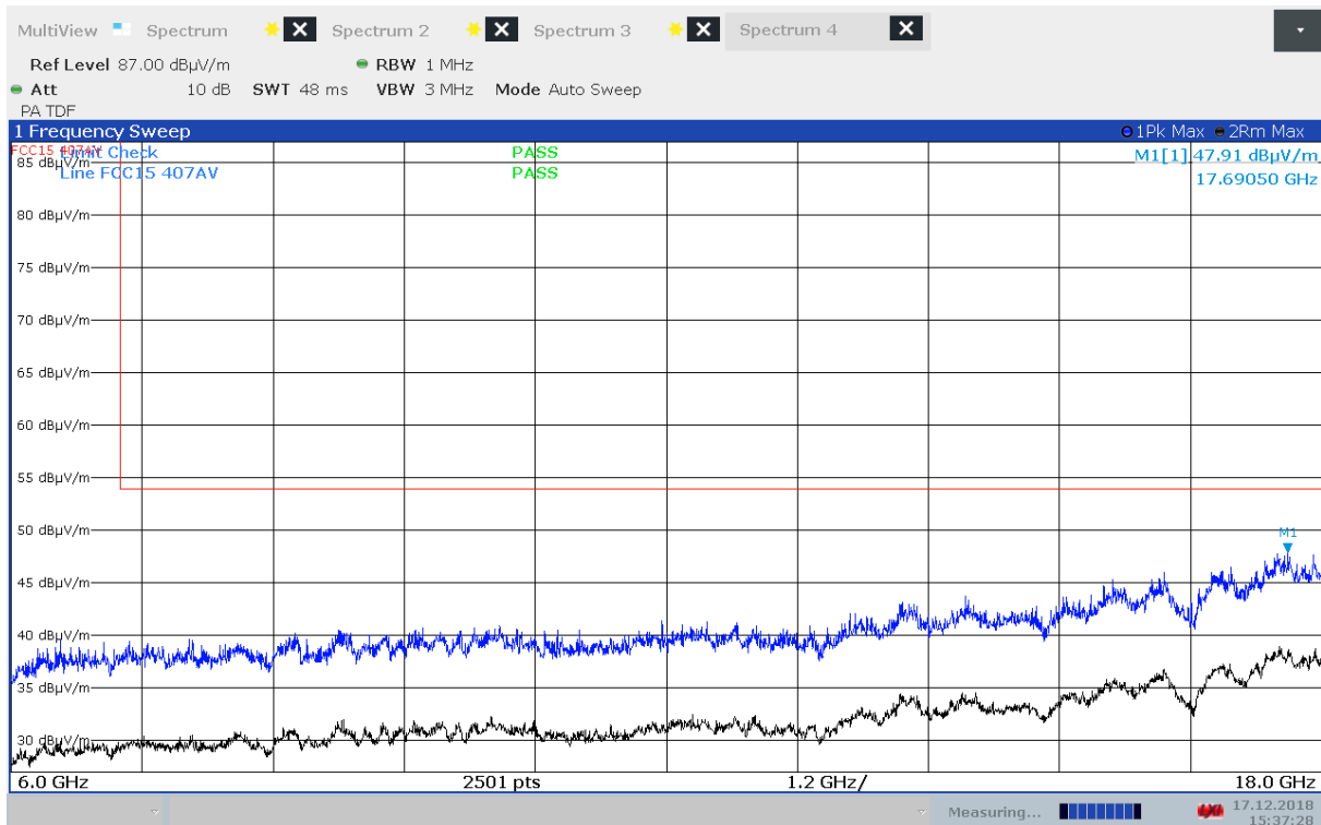
Radiated Emissions, 6000 - 18000 MHz, 5745 MHz, 802.11a 6Mbps, EUT V, VP
