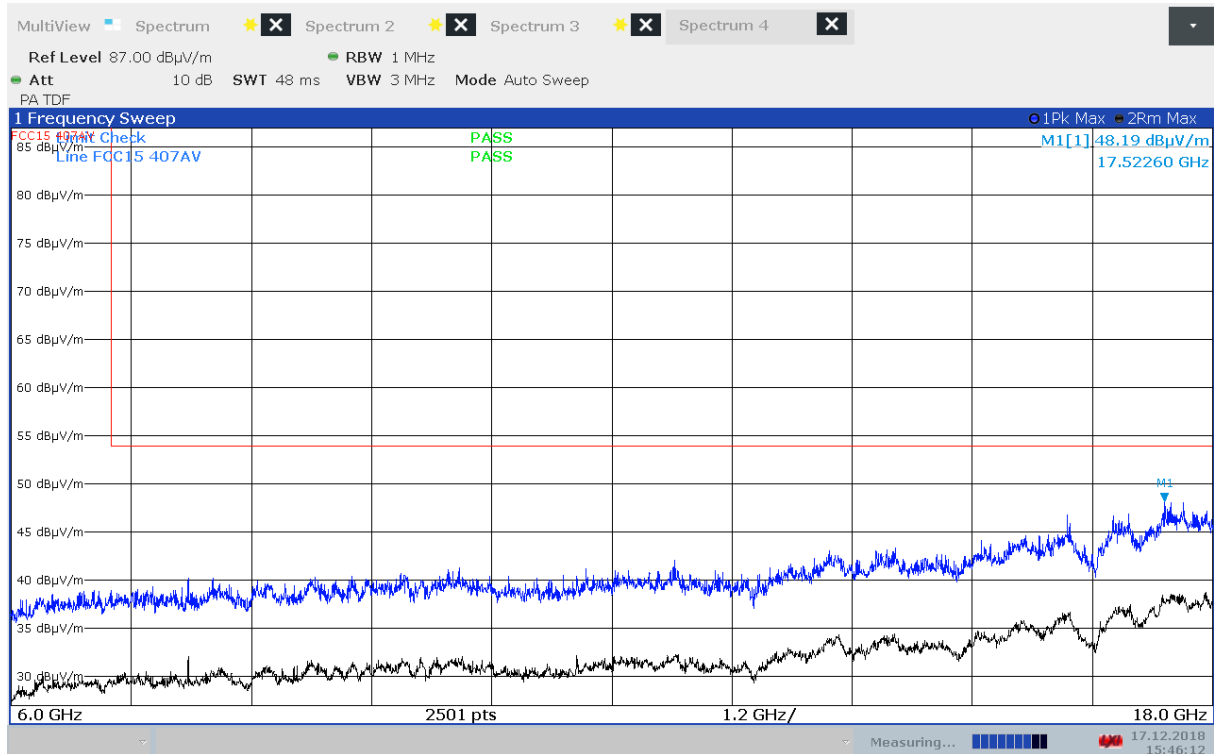
Radiated Emissions, 6000 - 18000 MHz, 5825 MHz, 802.11a 6Mbps, EUT V, HP
