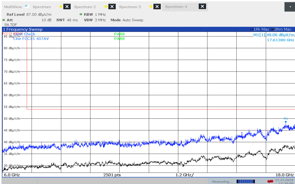
Radiated Emissions, 6000 - 18000 MHz, 5700 MHz, 802.11a 6Mbps, EUT V, VP
