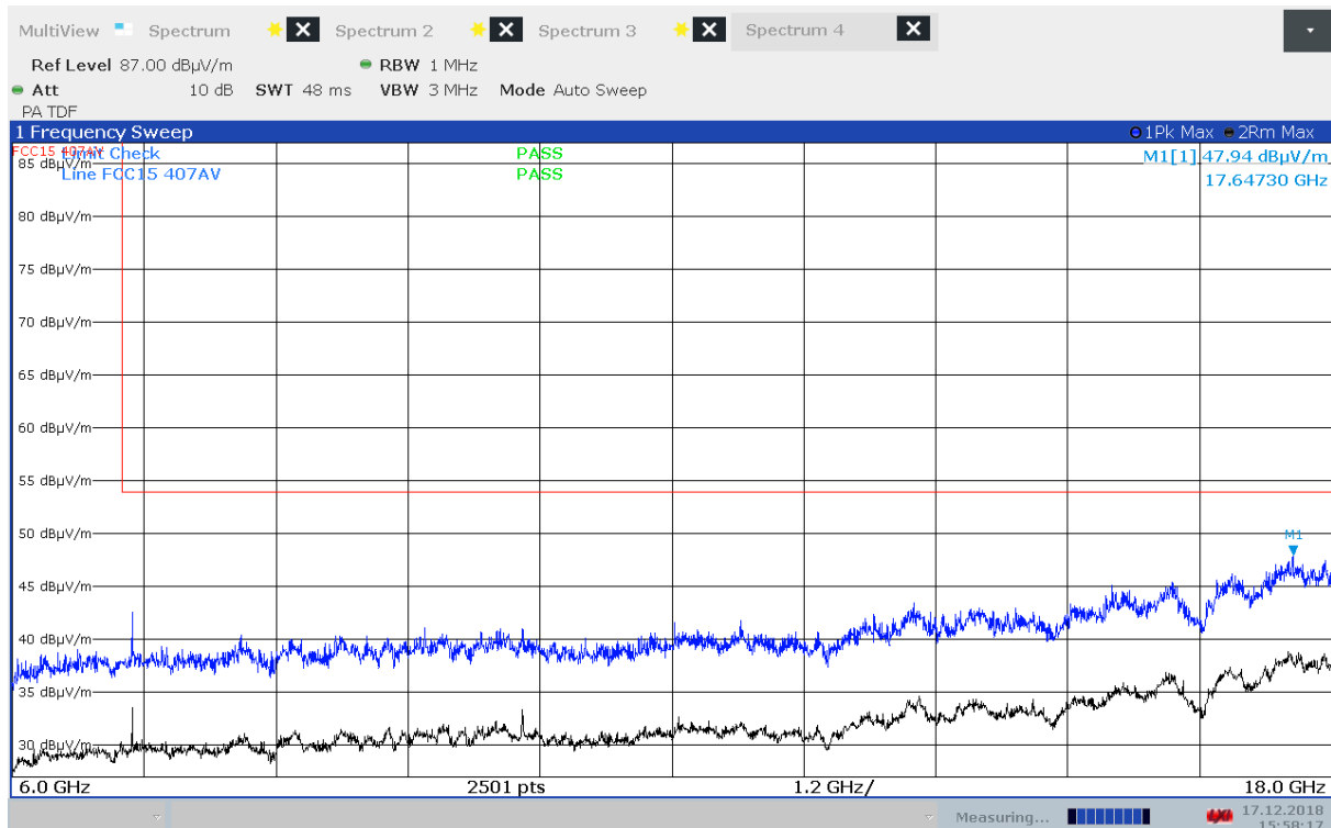
Radiated Emissions, 6000 - 18000 MHz, 5320 MHz, 802.11a 6Mbps, EUT V, VP
