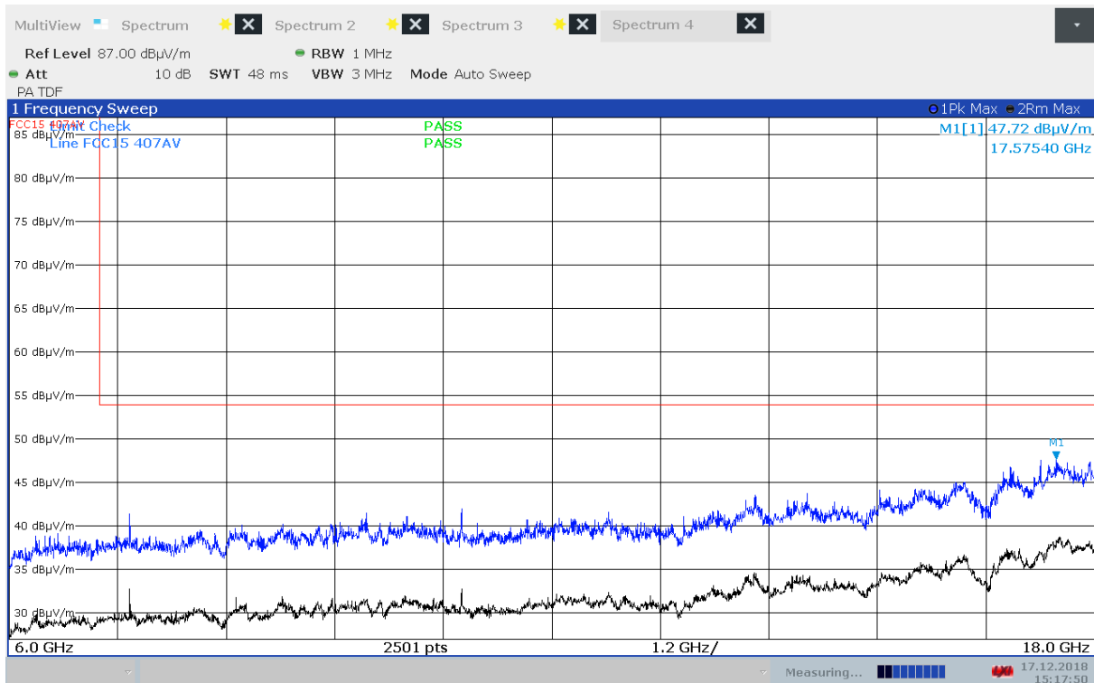
Radiated Emissions, 6000 - 18000 MHz, 5500 MHz, 802.11a 6Mbps, EUT V, VP
