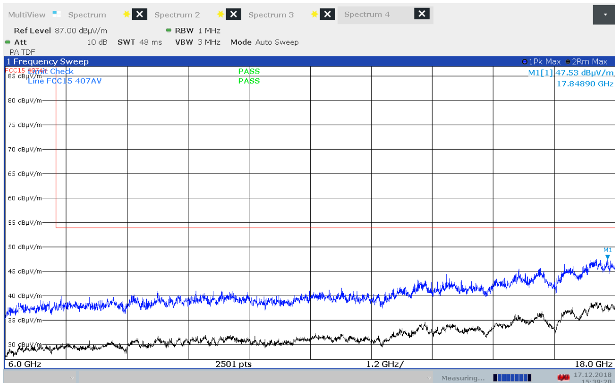
Radiated Emissions, 6000 - 18000 MHz, 5745 MHz, 802.11a 6Mbps, EUT V, HP
