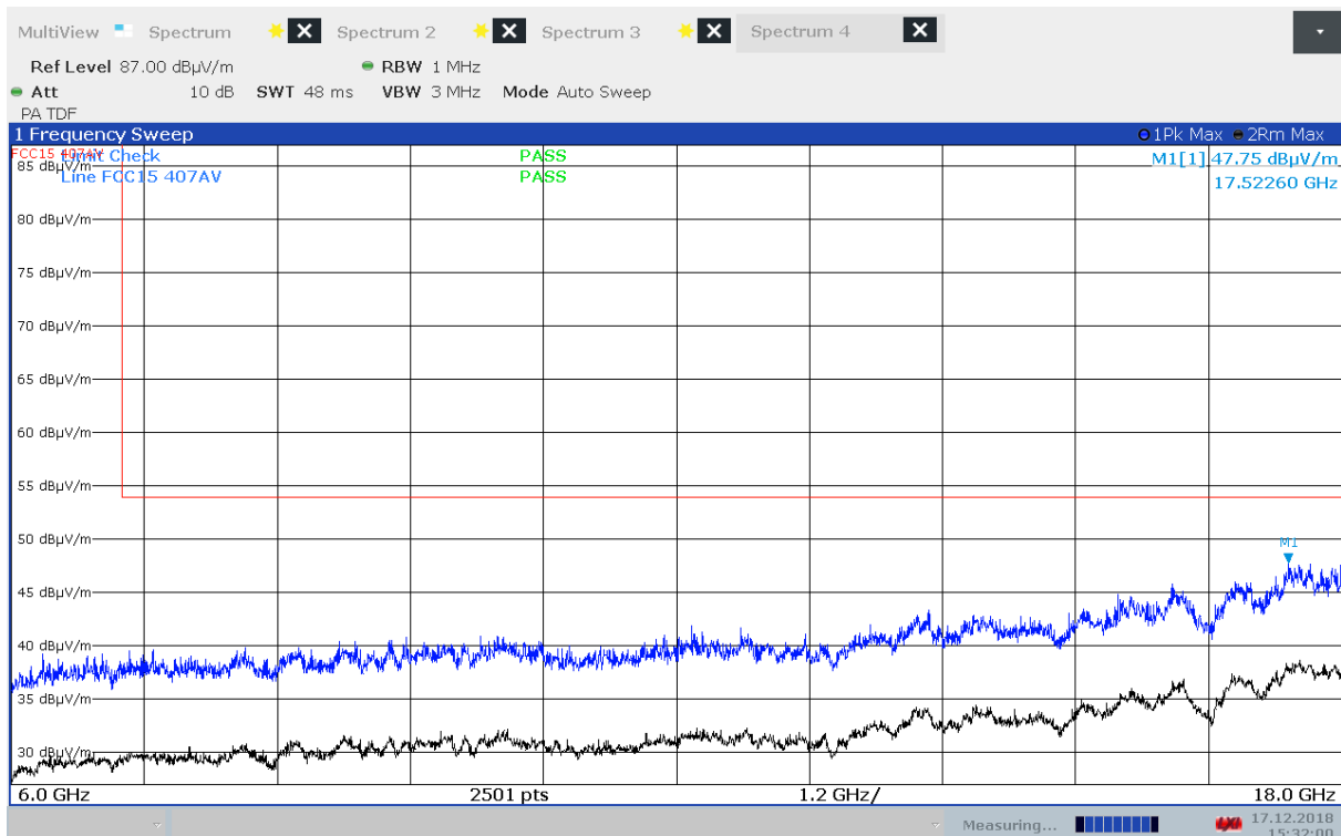
Radiated Emissions, 6000 - 18000 MHz, 5700 MHz, 802.11a 6Mbps, EUT V, HP
