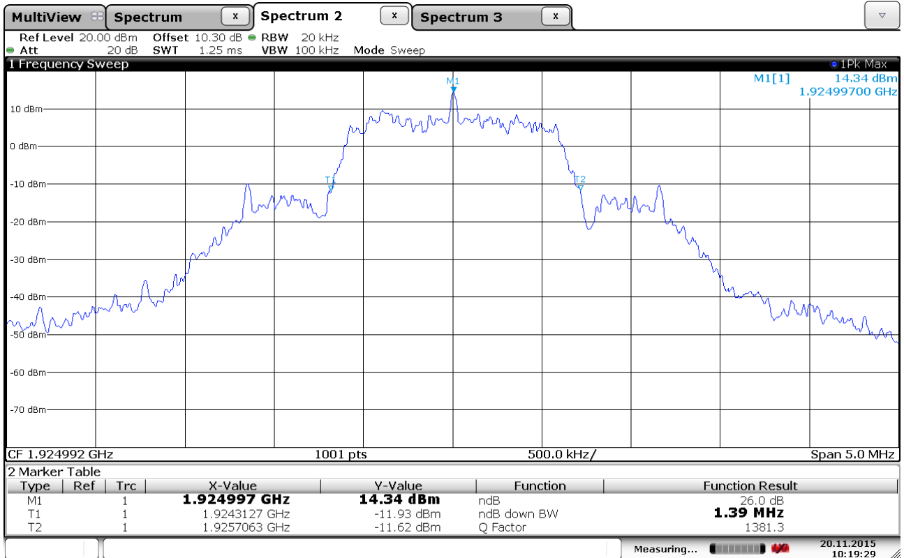
Emission Bandwidth B, Mid Channel
