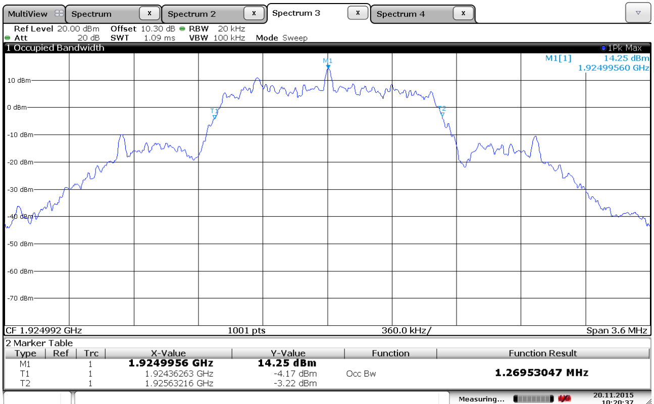
99% Bandwidth, Mid Channel
