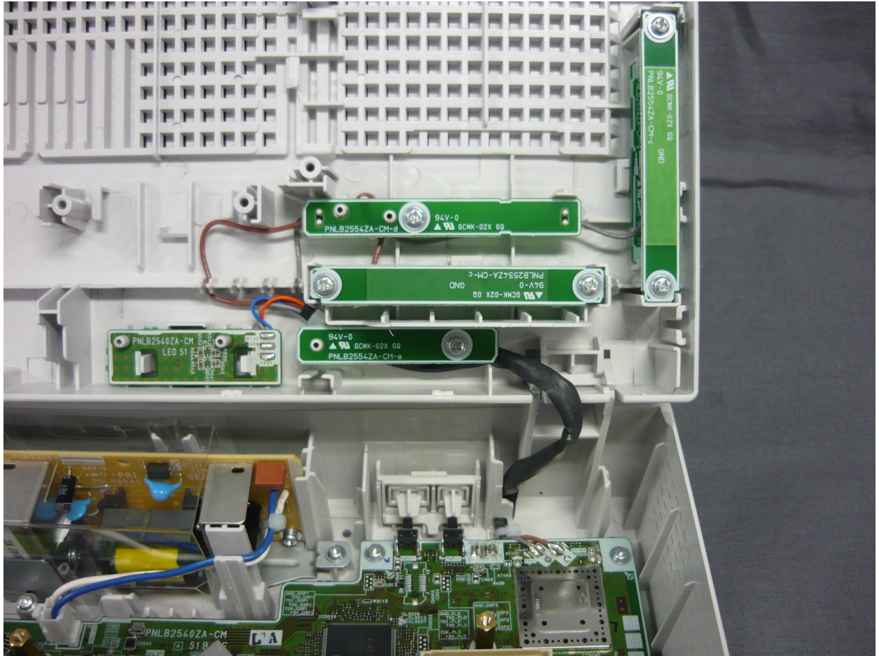
Internal view (Antenna and radio block)
