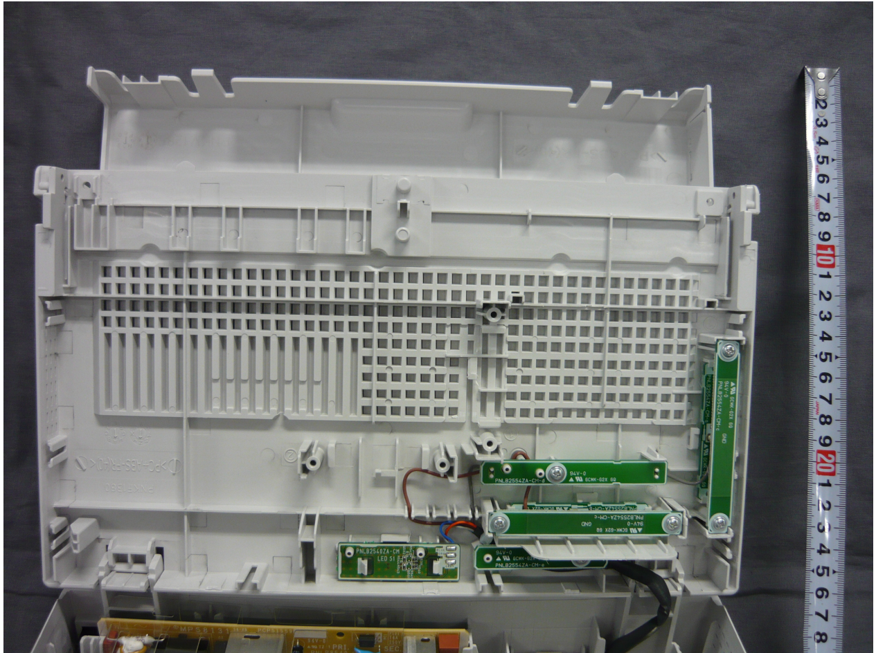
Internal view (Antenna block)
