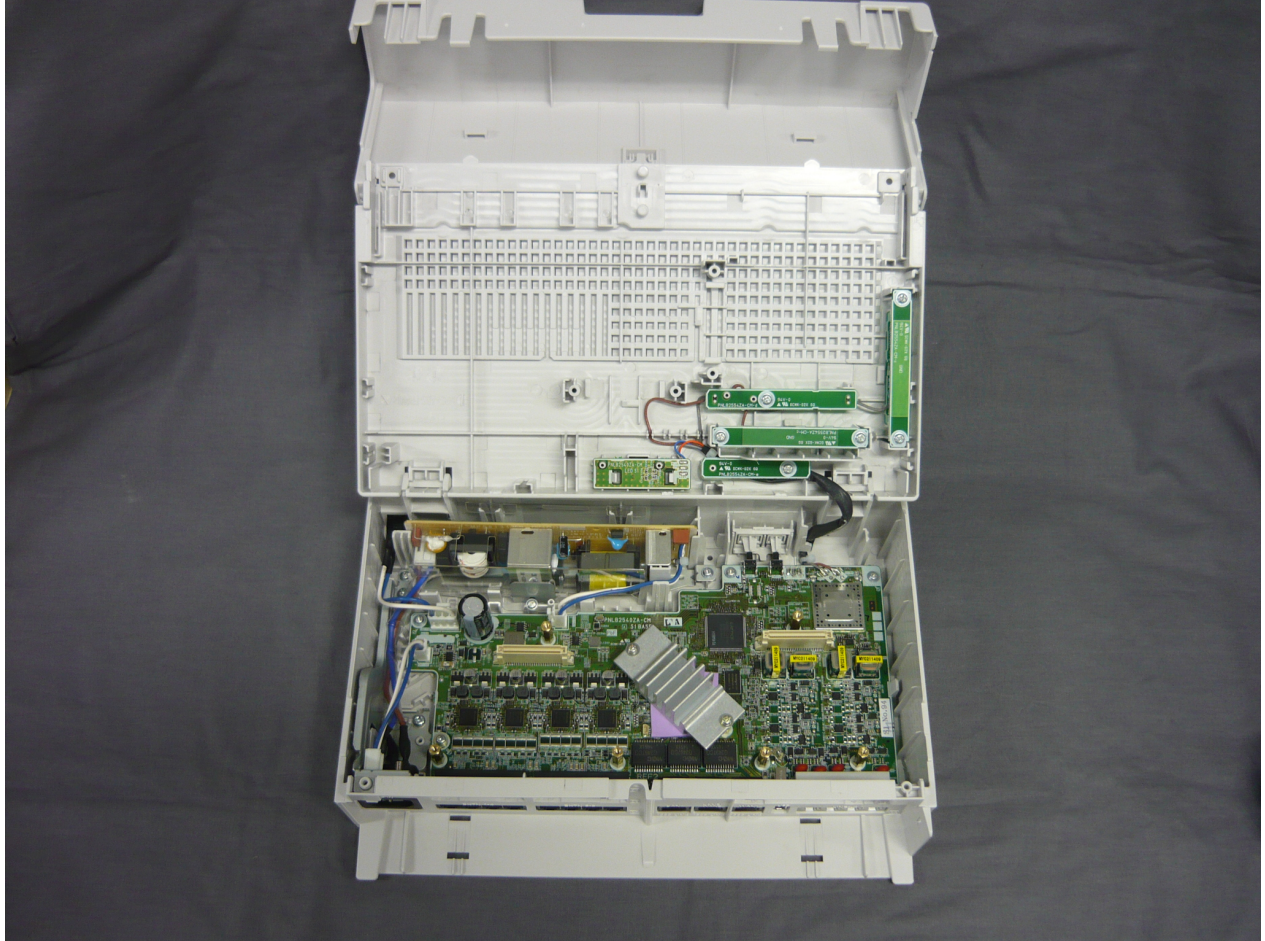
Internal view (front cover opened)
