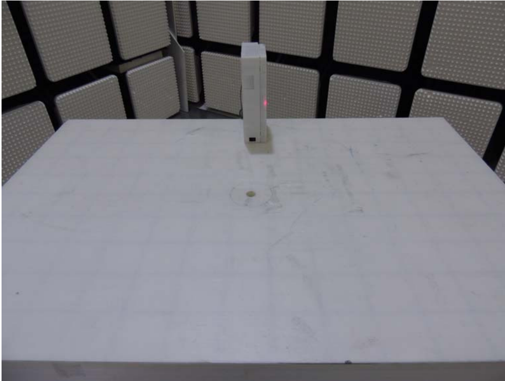
Photograph 2: Set-up for Radiated Emission, below 1GHz, EUT Configuration Y-Axis, Front View
