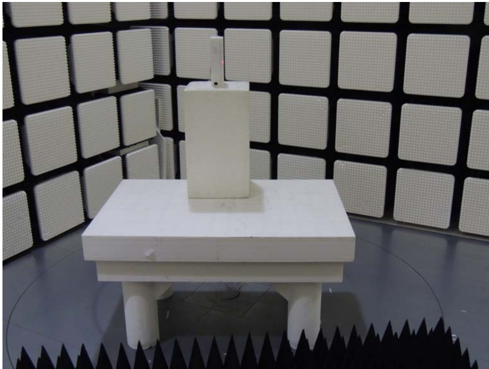
Photograph 4: Set-up for Radiated Emission, Above 1GHz, EUT Configuration Y-Axis, Front View
