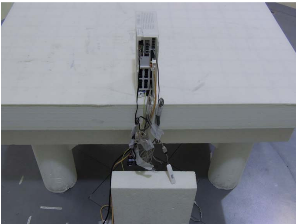
Photograph 3: Set-up for Radiated Emission, below 1GHz, EUT Configuration Y-Axis of Transmitter, Rear View
