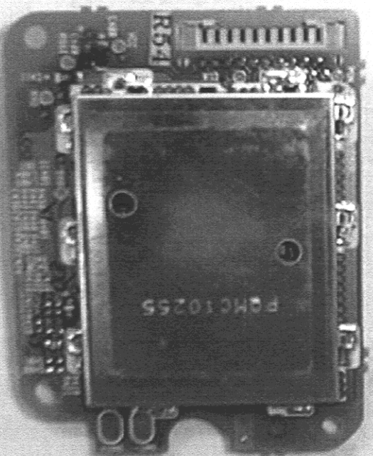
With Cover
