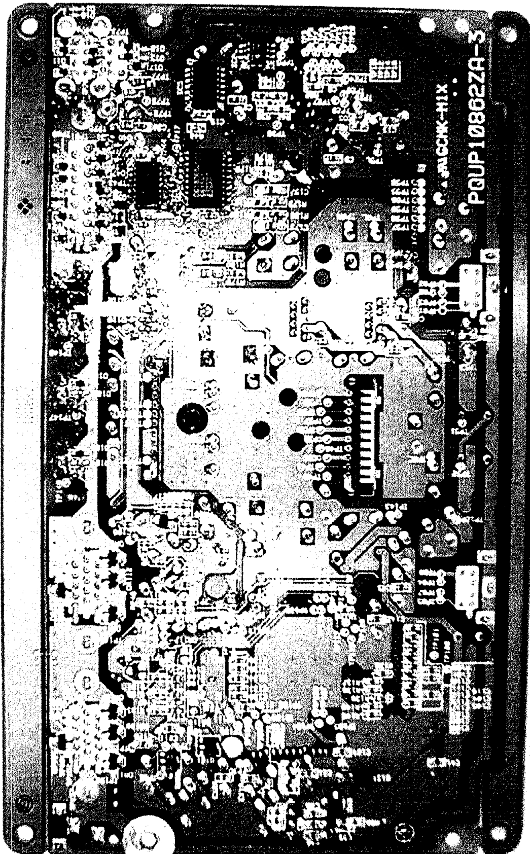
Main Board (Bottom Side)
