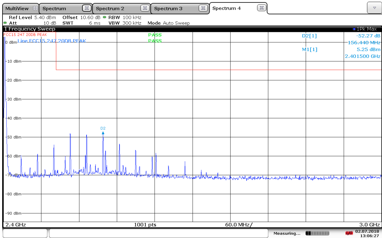
Conducted Emissions, 2400 -3000MHz, ch00
