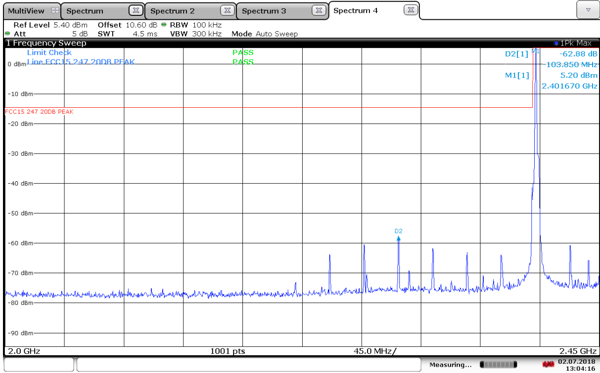
Conducted Emissions, 2000 -2450MHz, ch00
