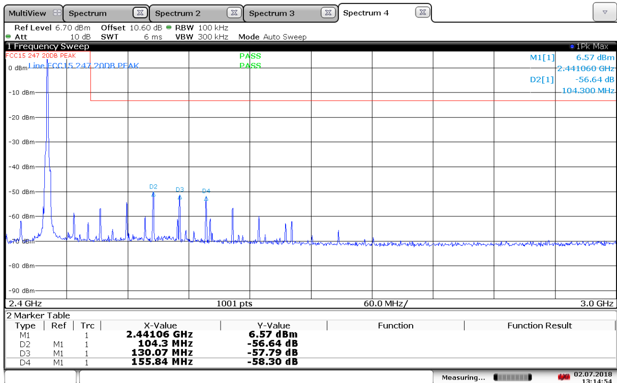
Conducted Emissions, 2400 -3000MHz, ch39
