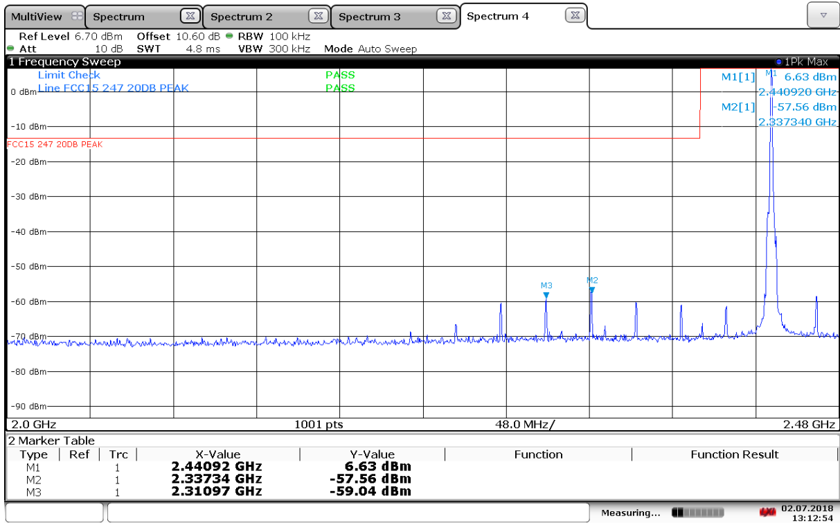
Conducted Emissions, 2000 -2480MHz, ch39
