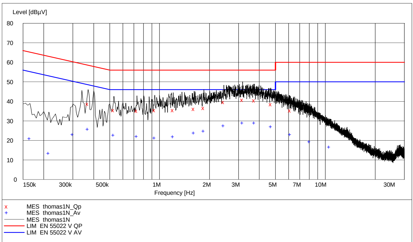
On-Hook, Charging Mode, AC Adaptor PNLV226(UC), 120V 60Hz
