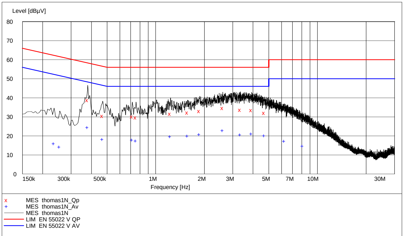
Off-Hook, Speech Mode, AC Adaptor PNLV226(UC), 120V 60Hz
