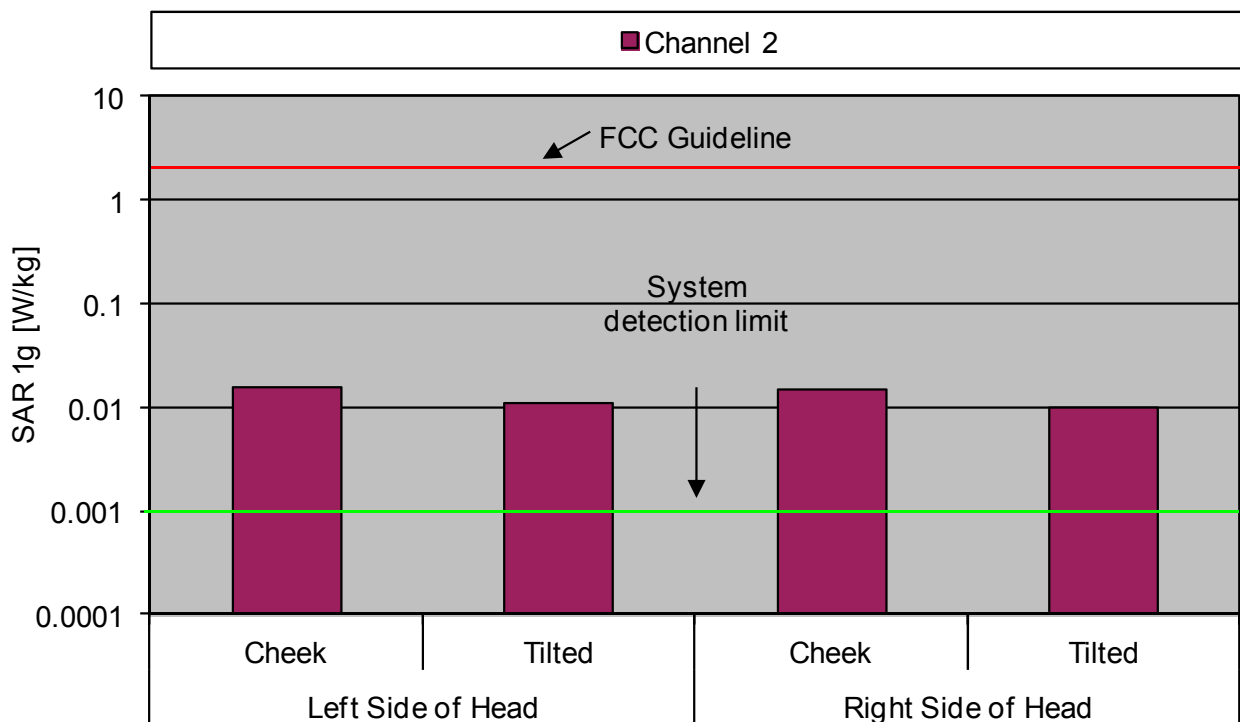
Fig. 8: The reported SAR values for head configuration for the Panasonic KX-PRWA13, for the US DECT standard in comparison to the FCC exposure limit.
