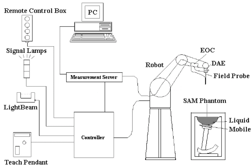
Fig. 6: The DASY4 measurement system.
