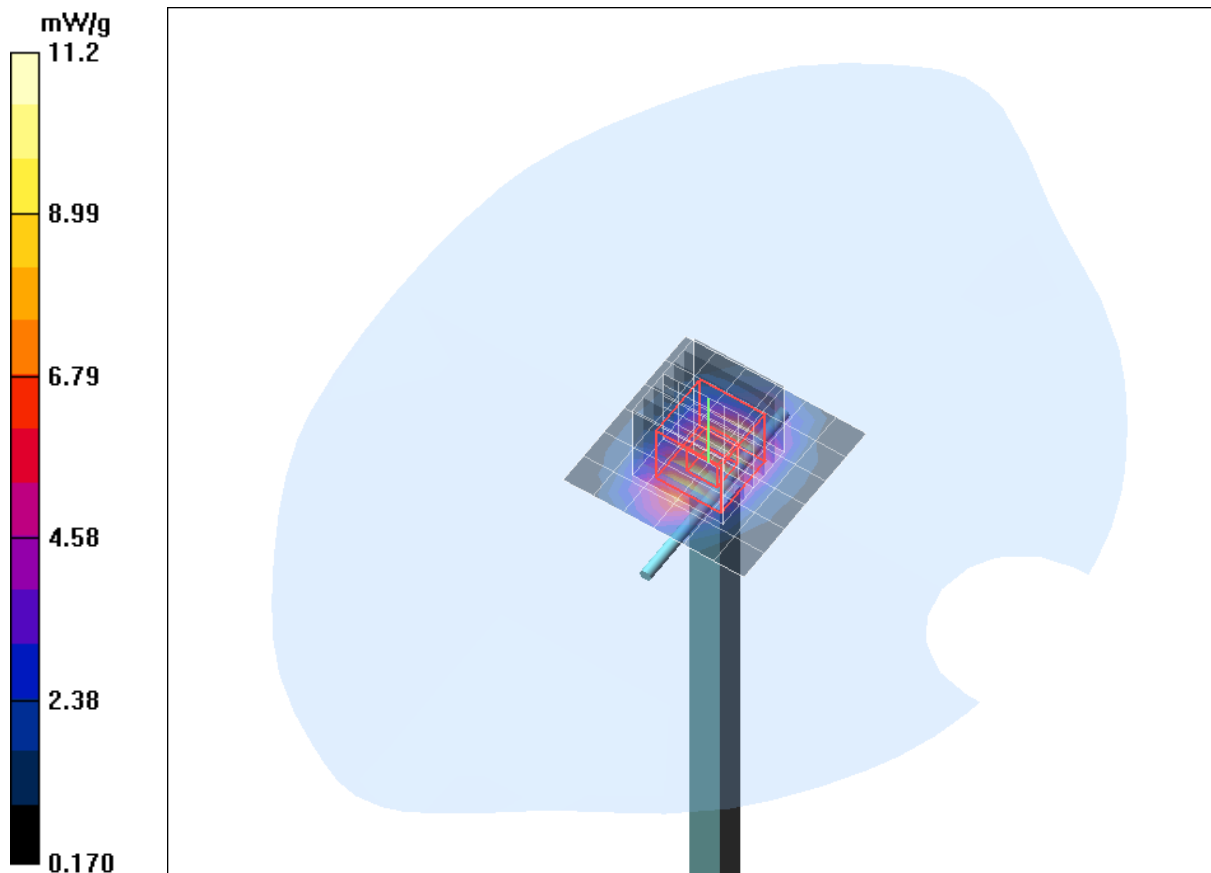
Fig. 10: Validation measurement 1900 MHz Head (December 02, 2013), coarse grid.
