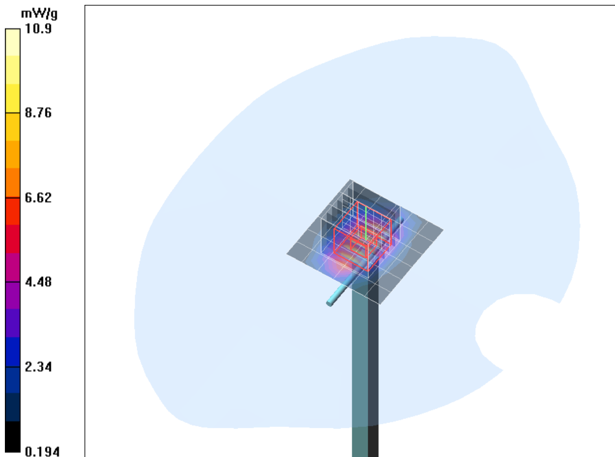
Fig. 11: Validation measurement 1900 MHz Body (December 02, 2013), coarse grid.
