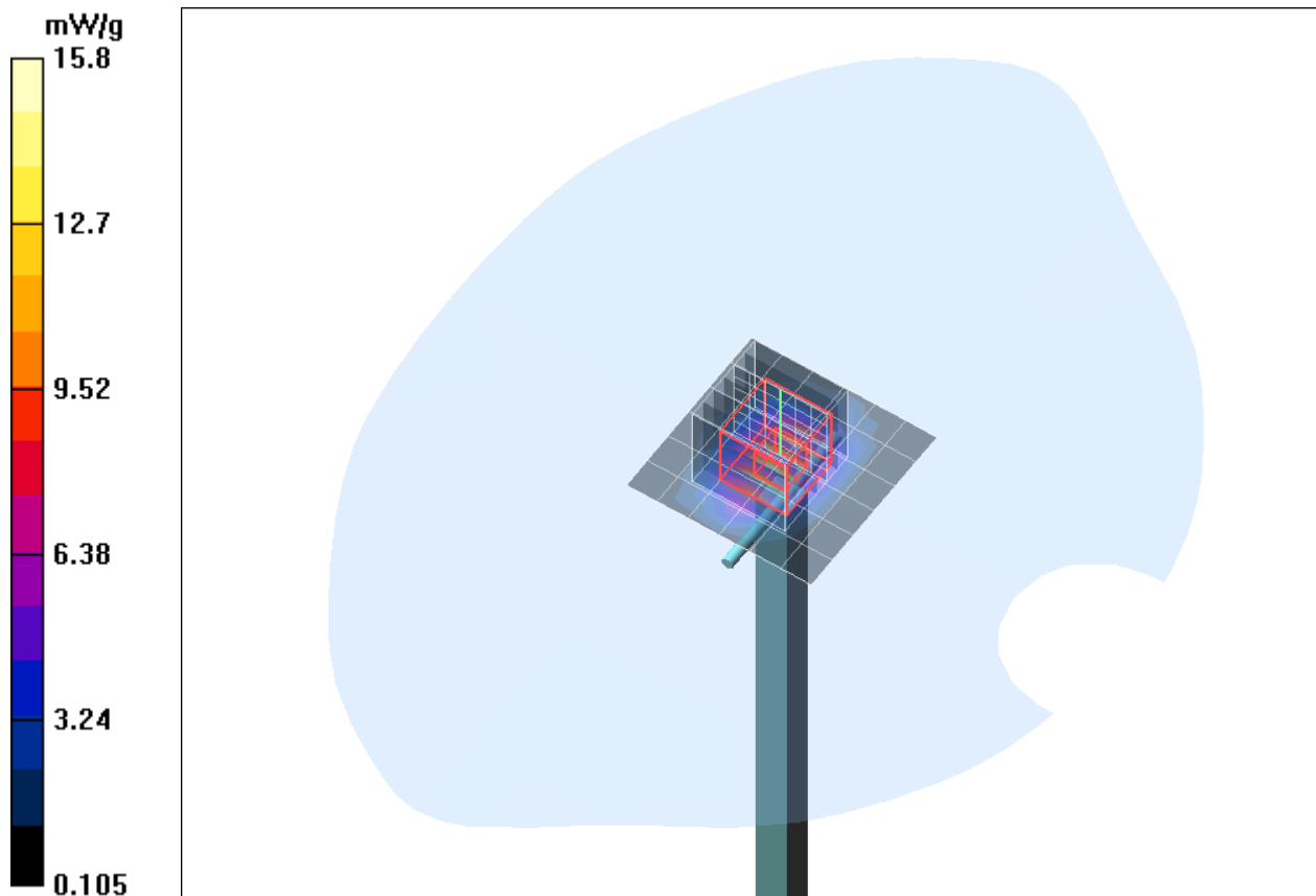
Fig. 13: Validation measurement 2450 MHz Head (November 28, 2013), coarse grid.
