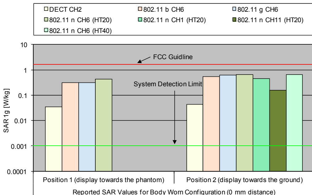
Fig. 9: The reported SAR values for body worn configuration for the Panasonic KX-PRXA10, for the US DECT and IEEE 802.11 b/g/n standard in comparison to the FCC exposure limit.
