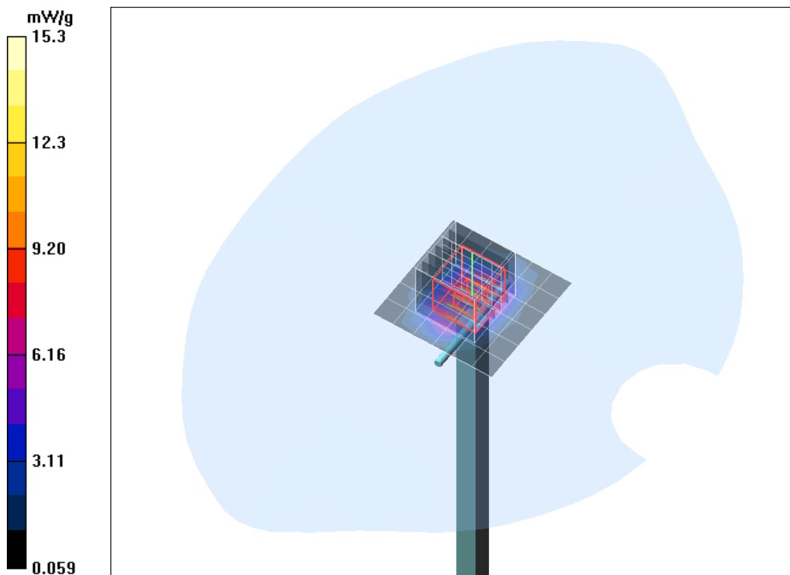
Fig. 12: Validation measurement 2450 MHz Head (November 25, 2013), coarse grid.
