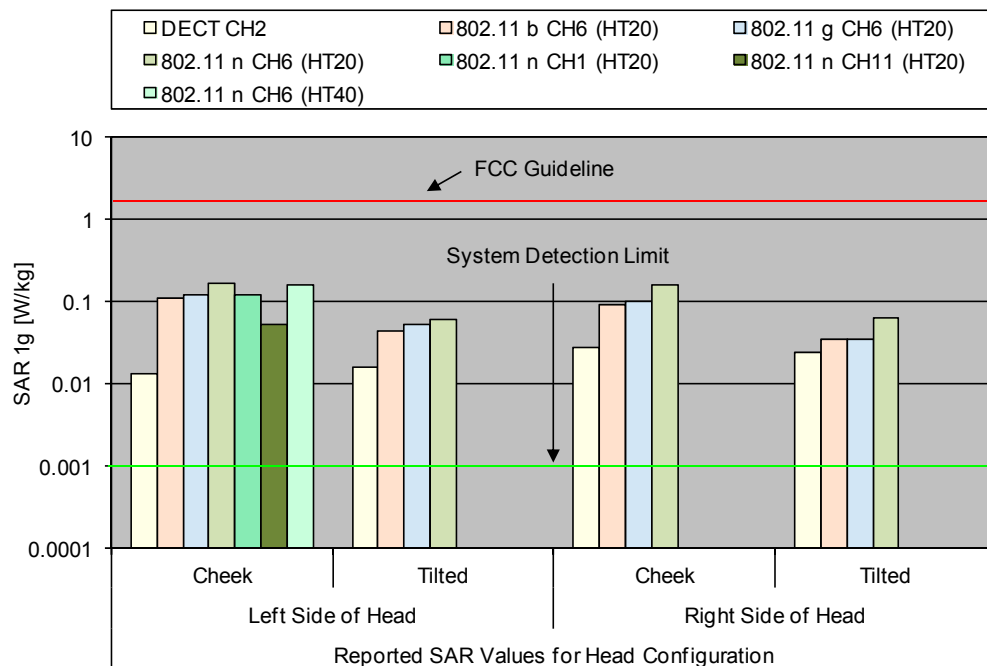
Fig. 8: The reported SAR values for head configuration for the Panasonic KX-PRXA10, for the US DECT and IEEE 802.11 b/g/n standard in comparison to the FCC exposure limit.
