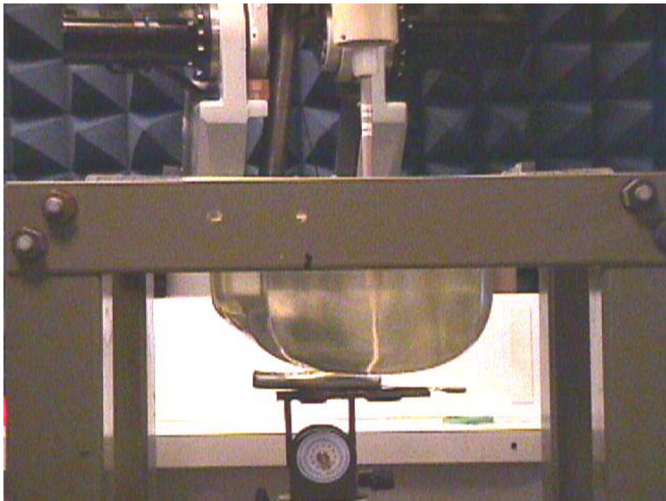
< Left Head, Check Position with the antenna fully extended – Overview >
