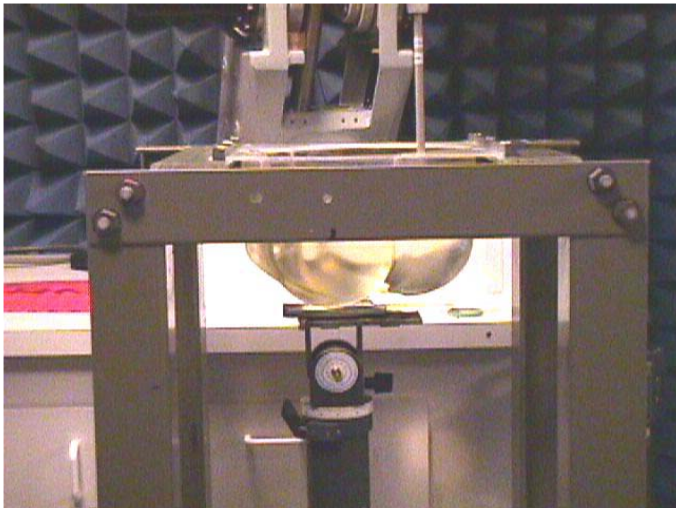
< Right Head, Check Position with the antenna retracted – Overview >
